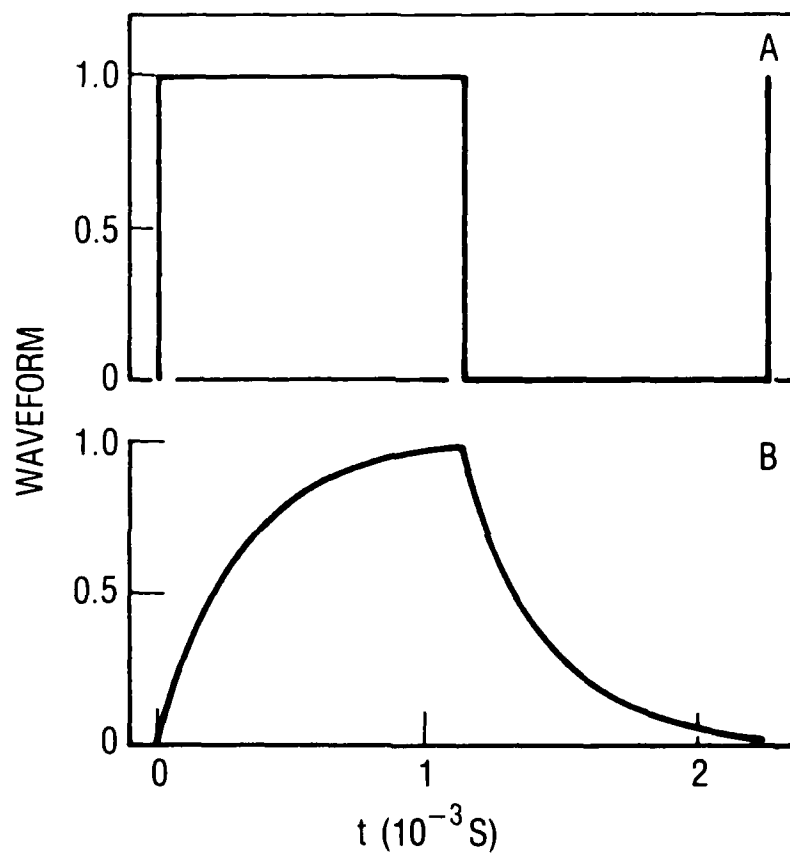
Fig. 7. Waveforms (in Arbitrary Units) for a Single-Velocity Cesium Beam Incident on a Tungsten Ionizer: f \approx 500 Hz, \tau \approx 3 \times 10^{-4} sec. A is the incident atomic beam, and B is the emerging ion current.
