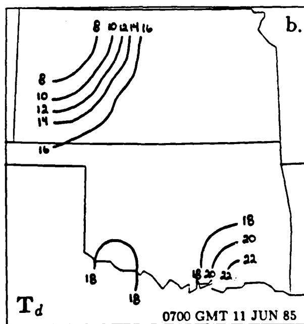
Fig. 18. As in Fig. 16 except for 0700 GMT, 11 June 1985.
