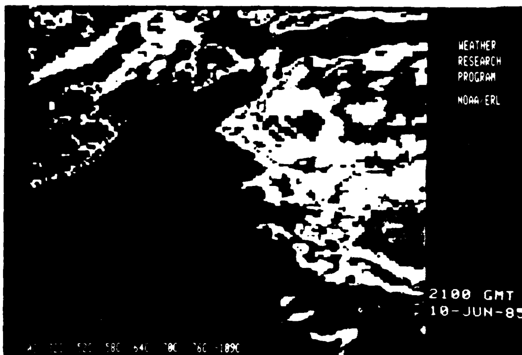
Fig 8. Visible (upper) and IR (lower) images of the forming squall line at 2100 GMT, 10 June 1985. In the IR image, green and yellow denote the most intense areas of convection.
