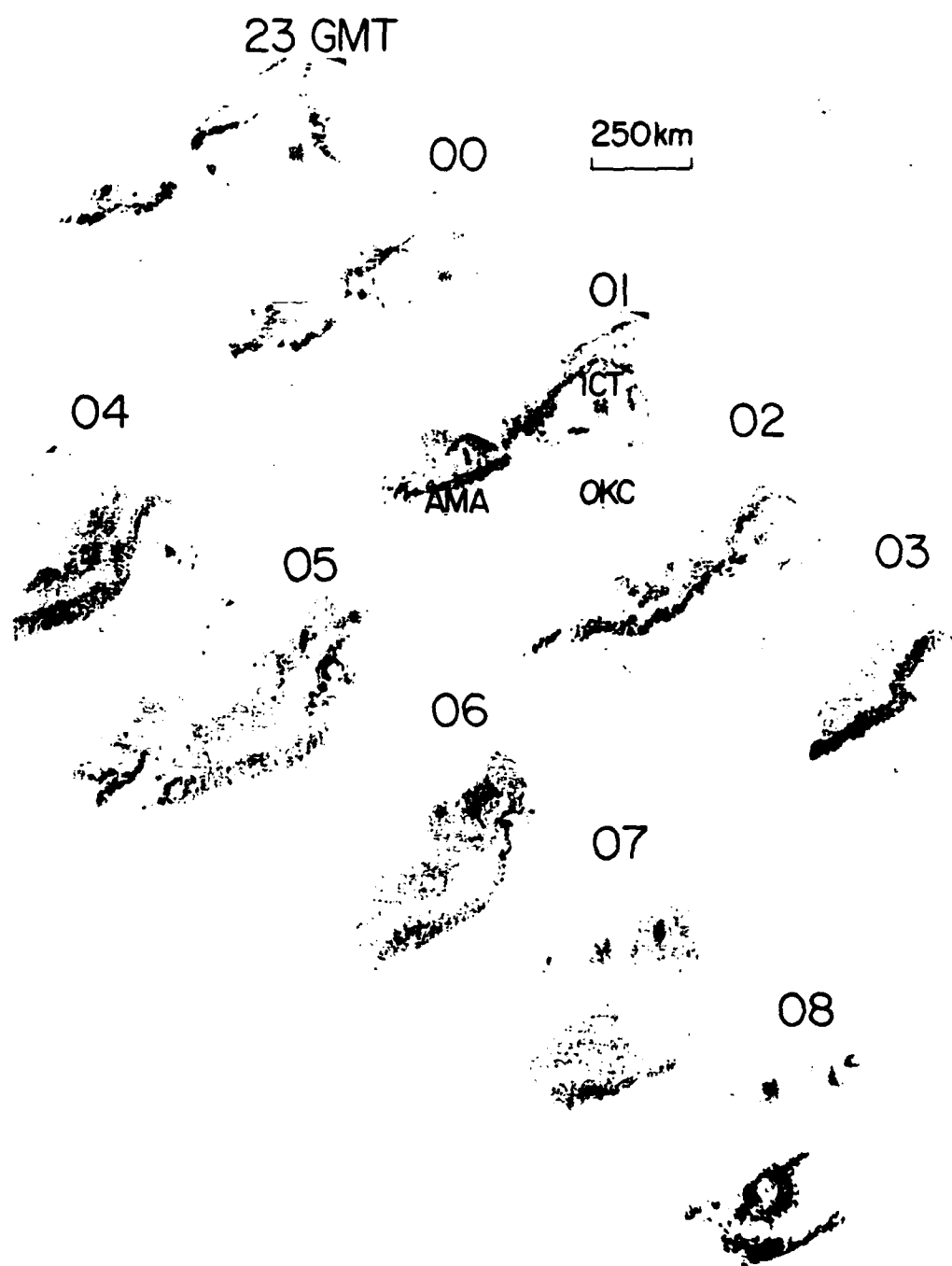
Fig. 13. Diagonal displays of composited low-level reflectivity at hourly intervals. Upper diagonal from 2300-0300 GMT and lower diagonal from 0400-0800 GMT. Reflectivity values from lightest to darkest shading are 15, 25, 35 and 50 dB(z). Locations of Amarillo, TX (AMA); Wichita, KS (ICT) and Oklahoma City, OK (OKC) are given
