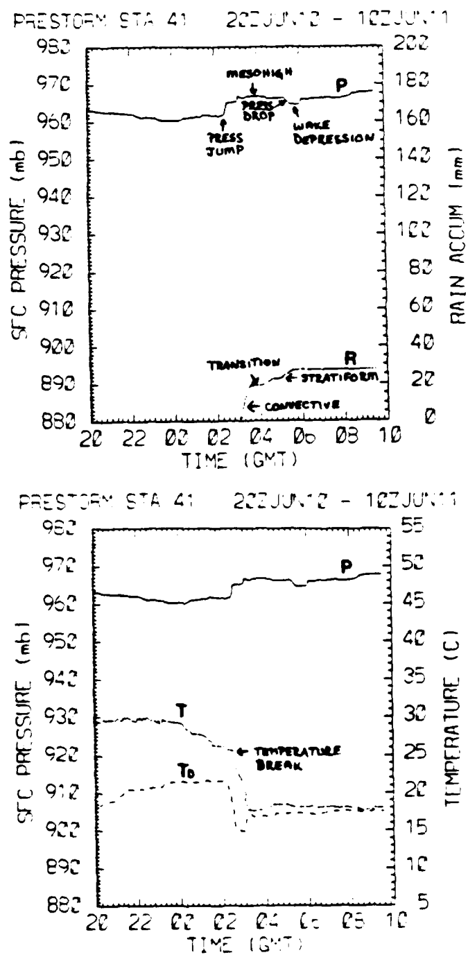
Fig. 35. As in Fig. 34 except for PAM station 41.
