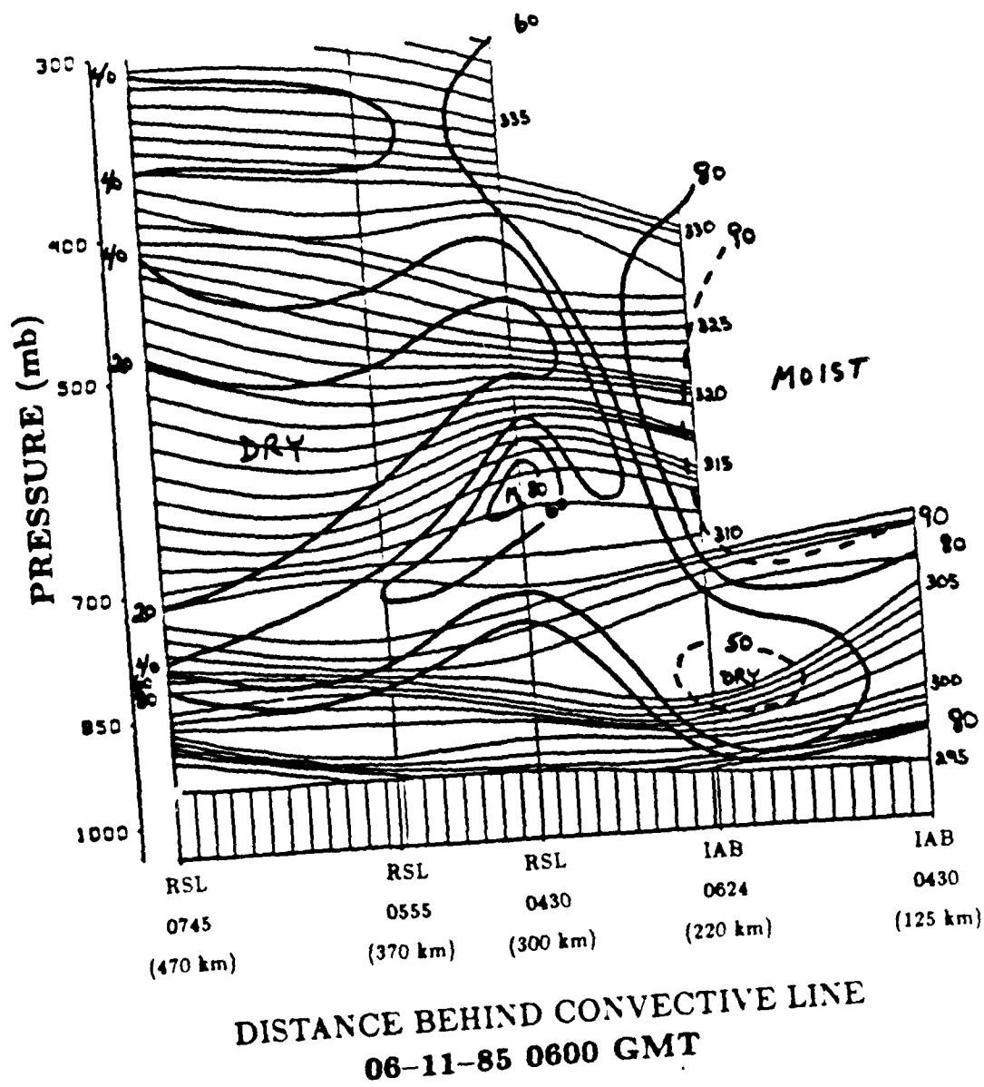
Fig. 43. Composite cross section of potential temperature (K) and relative humidity (%) at 0600 GMT, 11 June 1985. Isentropes are thin lines and isohumes are bold lines. Moist and dry regions labeled.
