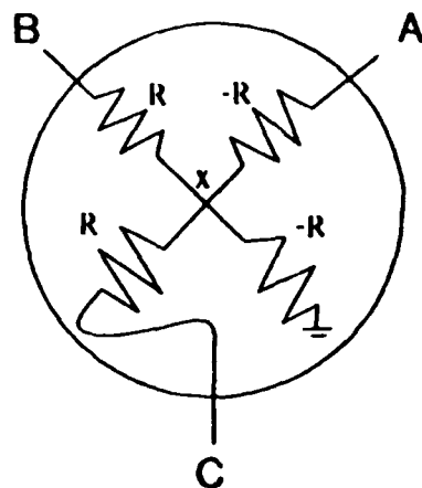
Figure 5-2. Negative resistance implementation.
