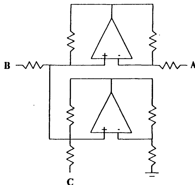
Figure 5-5. Negative impedance converter implementation.
