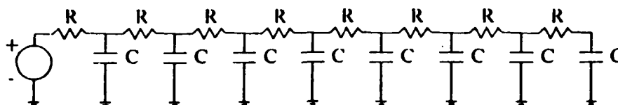
Figure 4-10. Simple RC line model of computation
