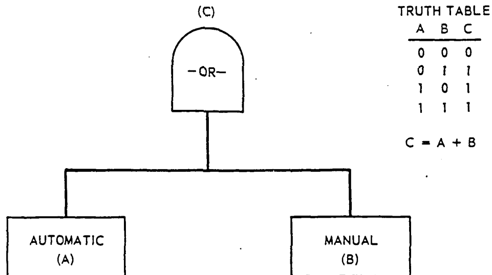
Figure 11 Logical -or- Truth Table
