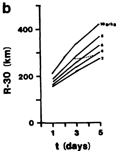
Figure 15 Effect of mid-level moisture (MLM) on the (a) minimum surface pressure (SLP) with time and on the (b) radius of 30-knot winds in layer 0 ( R_{30} ) with time.
