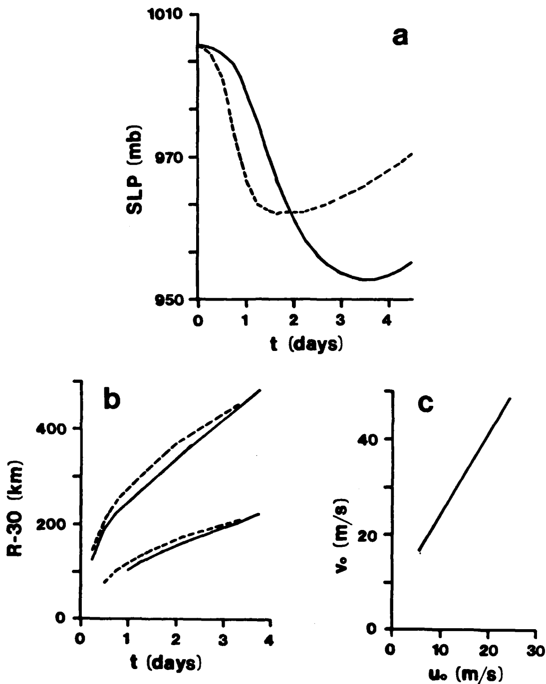
Figure 10 Comparison of results from the study numerical model (solid) and Ooyama's (1969) numerical model (dashed): (a) minimum surface pressure (SLP) with time, (b) radius of 30- and 50-knot surface winds ( R-30 & R-50 ) with time, and (c) maximum radial versus tangential winds (both model results are identical).
