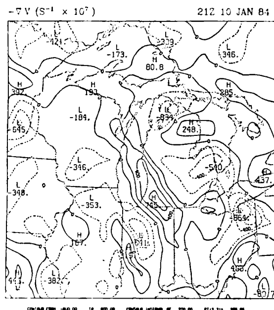
Figure 41. Surface convergence analysis for 2100 GMT 10 January 1984.
