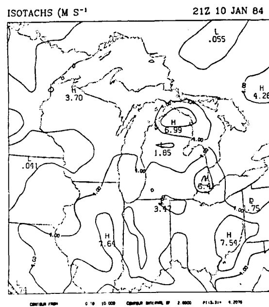
Figure 40. Surface specific humidity and isotach analyses for 2100 GMT 10 January 1984.
