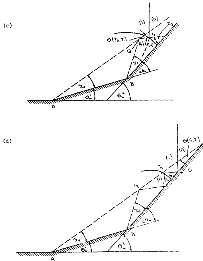
Figure 20: Schematic illustration of the shock wave reflection process for region 7. (a) Mach reflection over the first wedge. (b) Mach reflection over the second wedge. Q is the intersection of the triple point trajectories. (c) Inverse-Mach reflection over the second wedge after the incident shock has passed Q. (d) Regular reflection over the second wedge after the third triple point T_3 has reached with the wedge surface.
