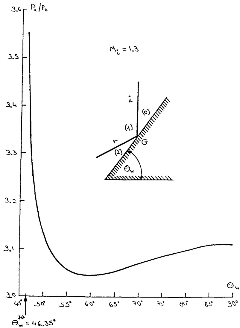
Figure 8: The ratio, P_2/P_0 , of the pressures behind and ahead of the reflection point of a regular reflection as a function of the reflecting wedge angle, \theta_w , for an incident shock wave Mach number M_1 = 1.3 , calculated using two-shock theory.
