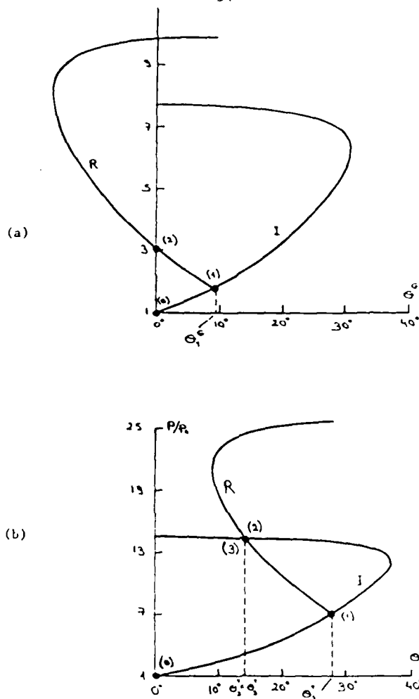
Figure 2: (P, \theta) shock polar solutions of (a) regular reflection ( M_1 = 1.3 , \theta_w = 60^\circ ) and (b) Mach reflection ( M_1 = 2.5 , \theta_w = 40^\circ , \lambda = 5.29^\circ ). The flow states are labelled (0) ahead of the incident shock wave, (1) behind the incident shock wave, (2) behind the reflected shock wave and (3) behind the Mach stem. R is the reflected shock polar, and I the polar for both the incident and Mach stem shocks which encounter the same incident flow in a pseudo-steady frame of reference.
