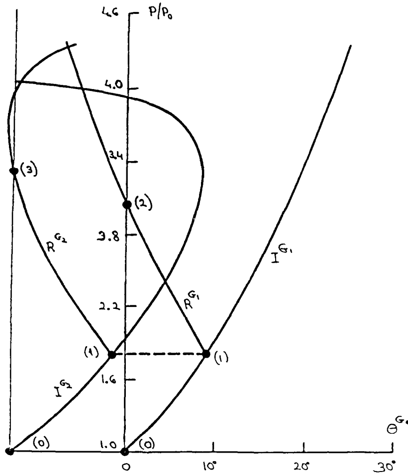
Figure 10: The shock polar solution of the shock wave reflection process for region 2. The polars are drawn accurately for an incident shock with Mach number M_1 = 1.3 , and a double convex wedge with inclinations \theta_w^1 = 60^\circ and \theta_w^2 = 47^\circ . I_G^1 , R_G^1 and I_G^2 , R_G^2 are the incident and reflected shock polars for the pseudo-steady regular reflections over the first and second wedges, respectively.
