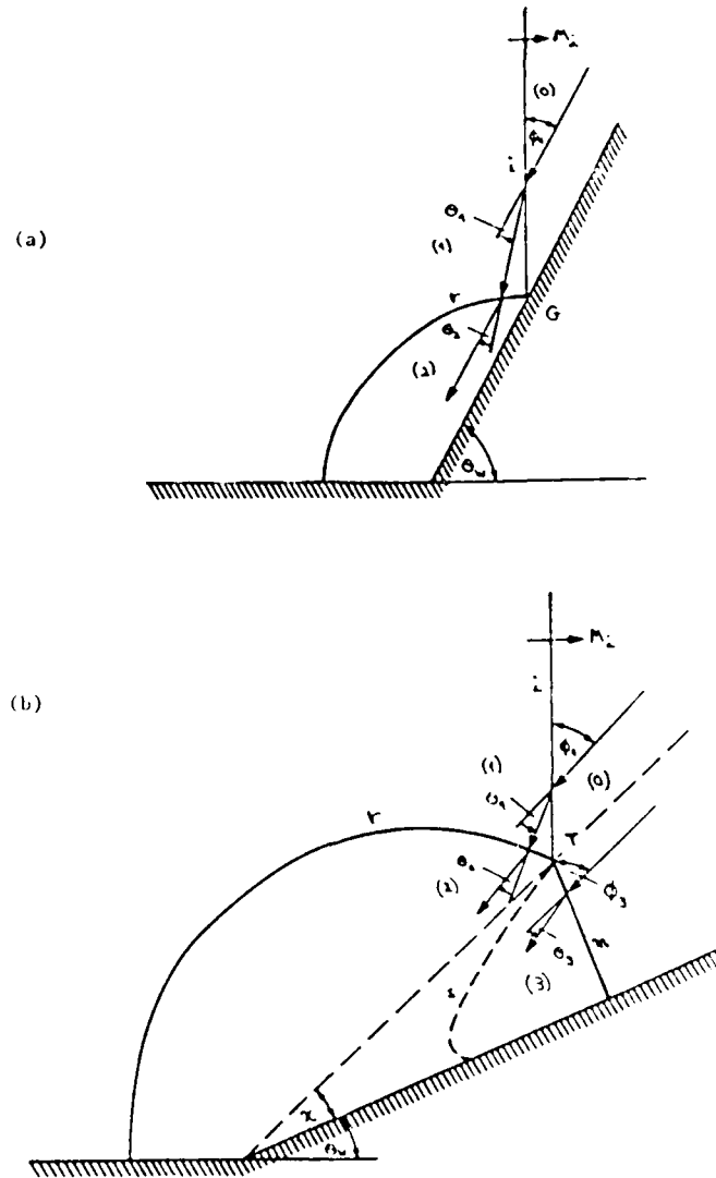
Figure 1: Schematic illustration of (a) regular reflection, and (b) Mach reflection. i -incident shock wave, r -reflected shock wave, m -Mach stem, s -slipstream, G -reflection point, T -triple point, \theta_w -reflecting wedge angle, \chi -triple point trajectory angle, \phi -angle of incidence, \theta -angle of deflection, (0)-(3) thermodynamic states.
