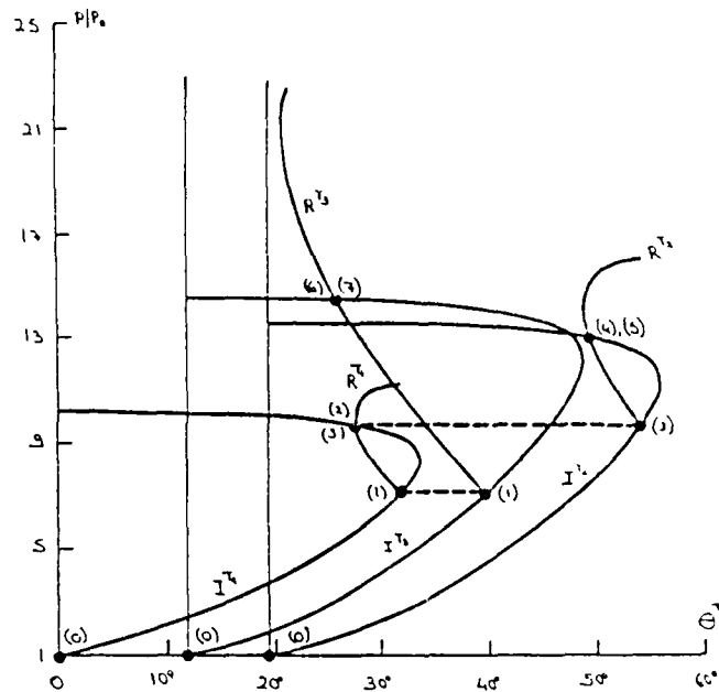
Figure 19: The shock-polar solution of the shock wave reflection process in region 6. The polars are drawn accurately for an incident shock with Mach number M_1 = 2.5 , and for a double concave wedge with inclinations \theta_w^1 = 20^\circ and \theta_w^2 = -40^\circ . The Mach number of the Mach stem shock over the first wedge is M_m = 2.9 , and the triple point trajectory angles are \chi_1 = 12.85^\circ , \chi_2 = 12.49^\circ and \chi_3 = 5.29^\circ . I_1^T and R_1^T are the incident and reflected shock polars of the pseudo-steady Mach reflection over the first wedge. I_2^T , R_2^T and I_3^T , R_3^T are the incident and reflected shock polars of the pseudo-steady Mach reflections over the second wedge, before and after the intersection of the triple point trajectories, respectively. The polars are linked by the dashed lines representing the constant pressures in states (3) and (1) of figure 18.
