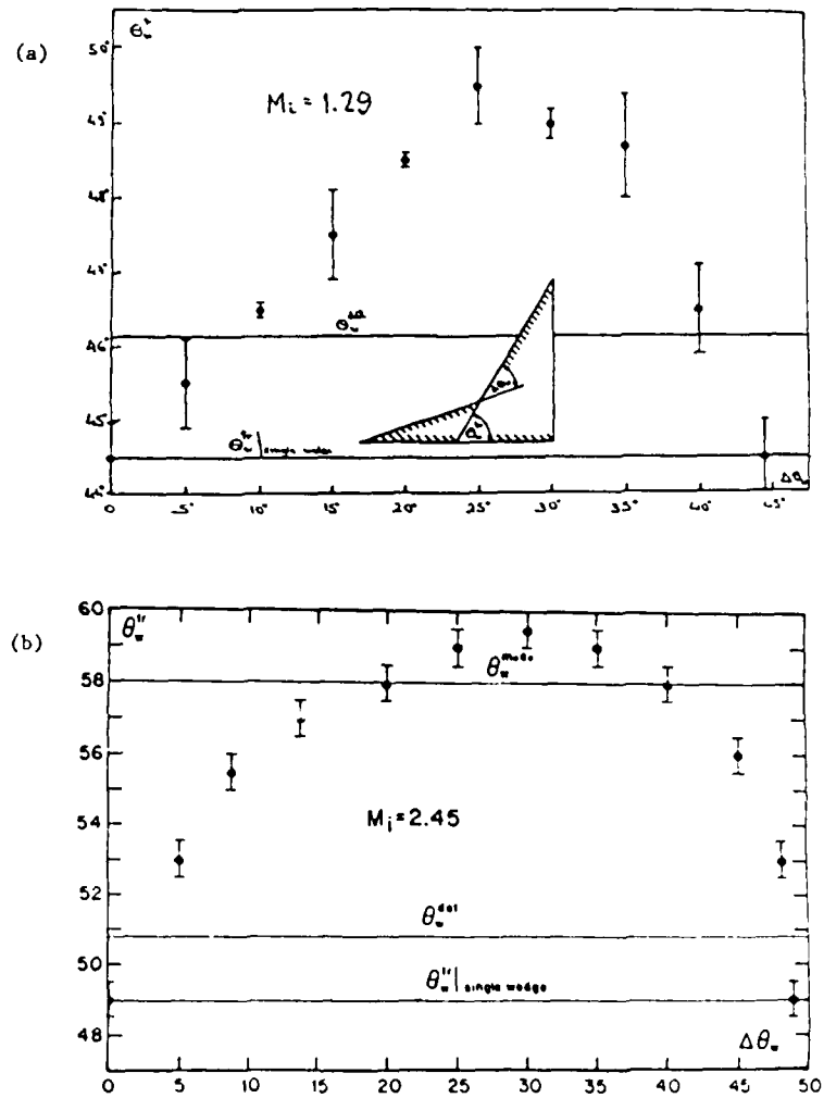
Figure 22: The angle of the second wedge at which transition from regular to Mach reflection was observed, \theta_w^{tr} , as a function of \Delta\theta_w for a concave double wedge:
