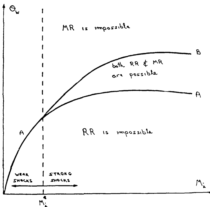
Figure 3: Regions of possible types of reflection in the (M_1, \theta_w) plane. M_1 is the incident shock wave Mach number, \theta_w the reflecting wedge angle, and M_1^* the limiting Mach number separating weak and strong shocks. For \gamma = 7/5 , M_1^* = 1.4565 .
