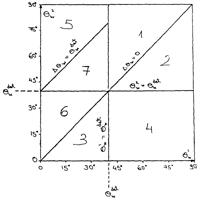
Figure 5: The seven regions in the (\theta_w^1, \theta_w^2) plane which identify the different reflection processes of a shock wave over a double wedge. \theta_w^1 is the first wedge angle, \Delta\theta_w the second wedge angle with respect to the first wedge, \theta_w^2 the second wedge angle, and \theta_w^{\det} the detachment wedge angle corresponding to the incident shock wave Mach number, M_1 . The reflection processes in each region are given in Table 1.
