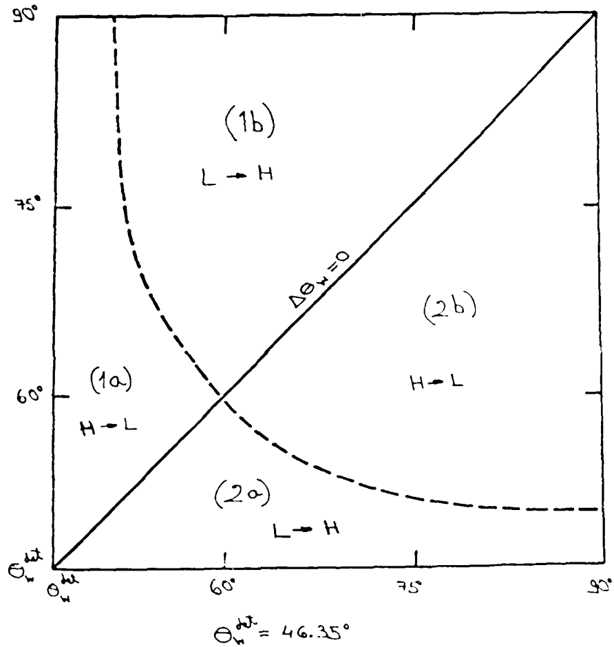
Figure 11: Subregions of the different regular to regular reflection processes in regions 1 and 2. In subregions 1a and 2b there will a transition from high to low pressure behind the reflected shock (H \rightarrow L), and in subregions 1b and 2a, a transition from low to high pressure (L \rightarrow H).
