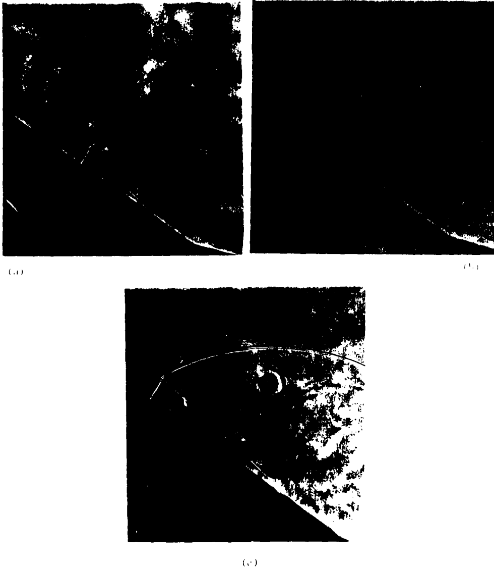
Figure 30: Shadowgraphs illustrating the reflection process over a double wedge in region 6. \theta_w^1 = 15^\circ and \theta_w^2 = 35^\circ . (a) The reflection of the Mach stem from the first wedge over the second surface as a Mach reflection. (b) The interaction of the two triple points. (c) The final Mach reflection over the second wedge surface.
