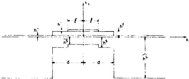
FIG. 7. Cross section of a composite resonator with the layer notched under the electrodes to cause trapping in the fundamental mode when it does not trap in the flat-plate configuration.
