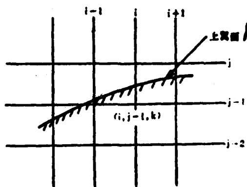
Fig. 2 The Relationship Between the Form of the Wing Cross Section and the Grid Network (Upper Surface) 1. Upper Surface
