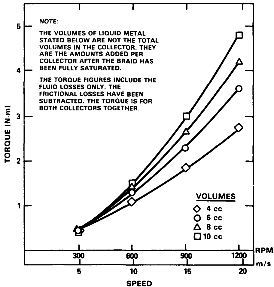
Fig. 6. Effect of speed and liquid metal volume on fluid losses.
