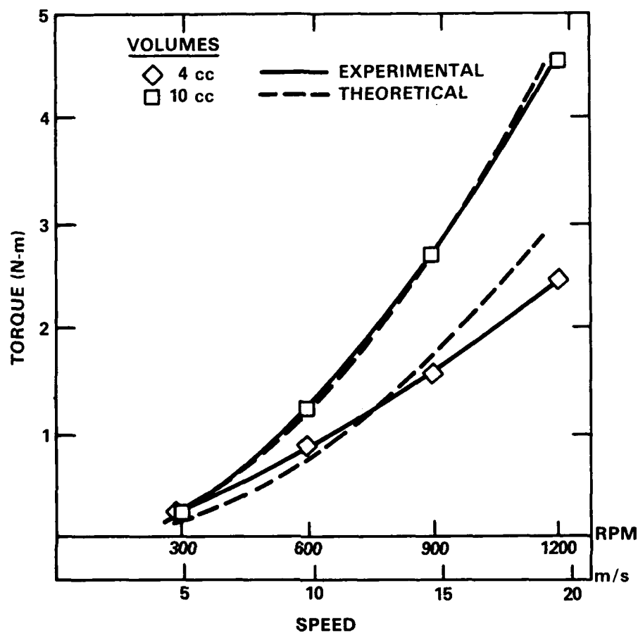
Fig. 7. Comparison of experimental and theoretical results.
