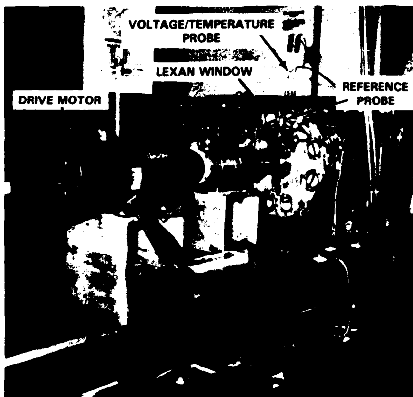
Fig. 1. Photo of test rig.
