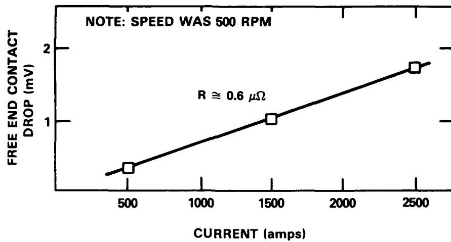
Fig. 5. Effect of current on contact drop.
