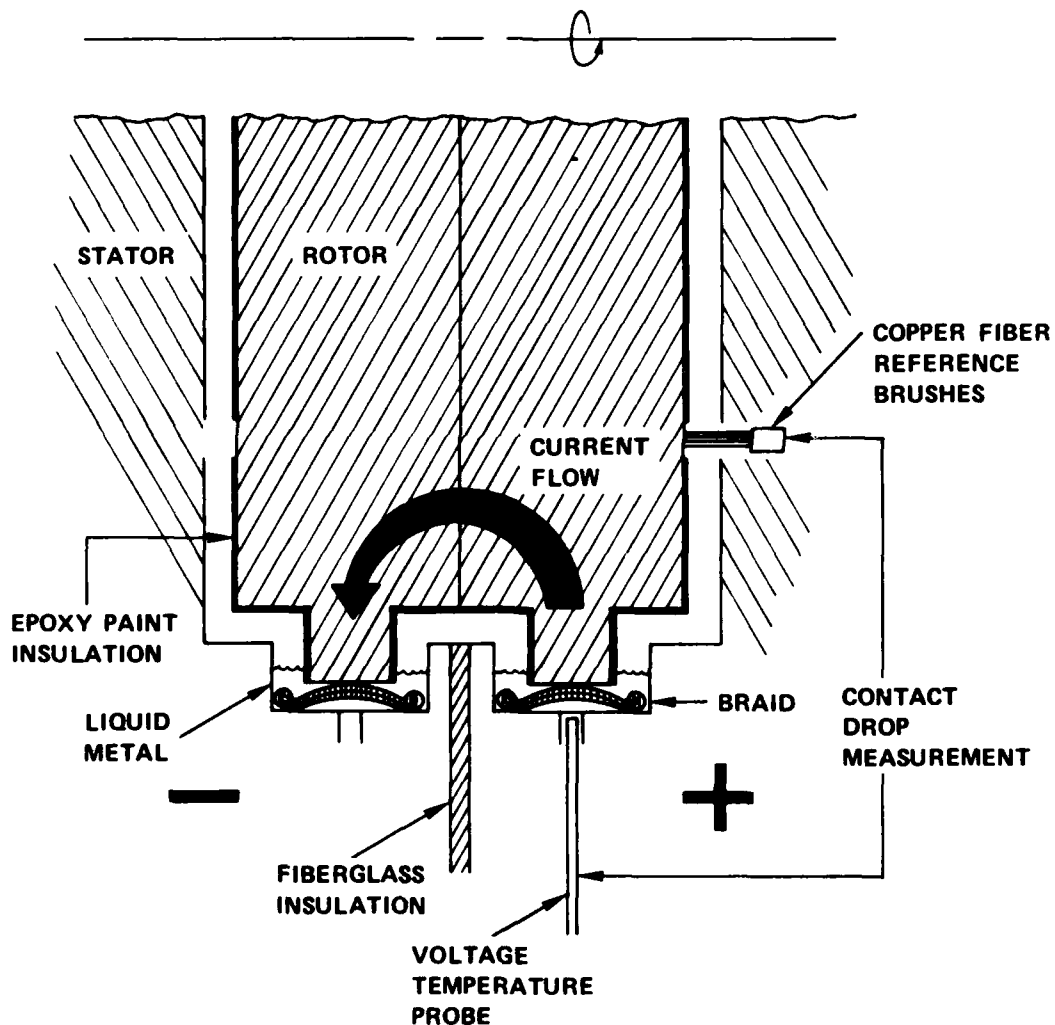
Fig. 2. Cross section of DTNSRDC liquid metal braid narrow gap collector.
