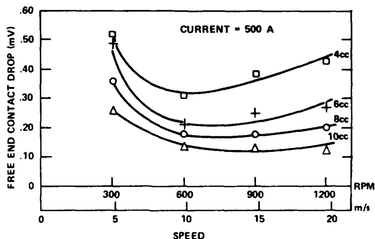
Fig. 4. Effect of speed and fill volume on contact drop.
