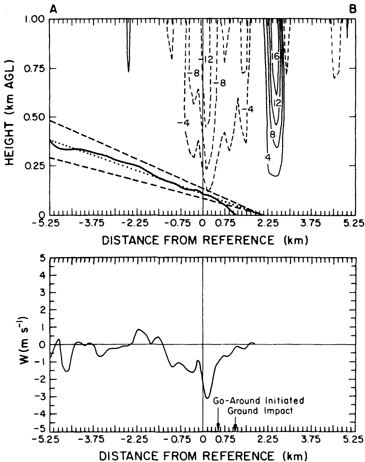
FIGURE 9B. Similar to 9a, but for vertical wind, contoured in 4 \text{ m s}^{-1} intervals. Graph at bottom shows vertical wind that would be experienced by model if it remained on the three degree approach path shown.
