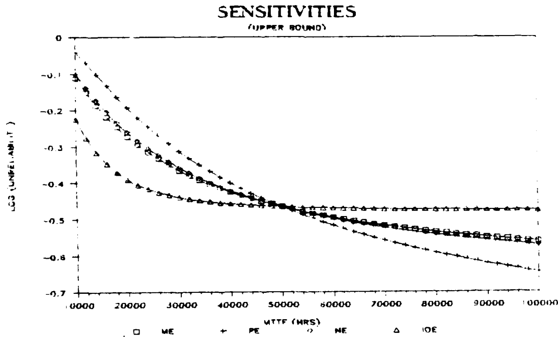
Figure 3.2-2: Cluster Reliability Sensitivities (Upper Bound Assumptions).
