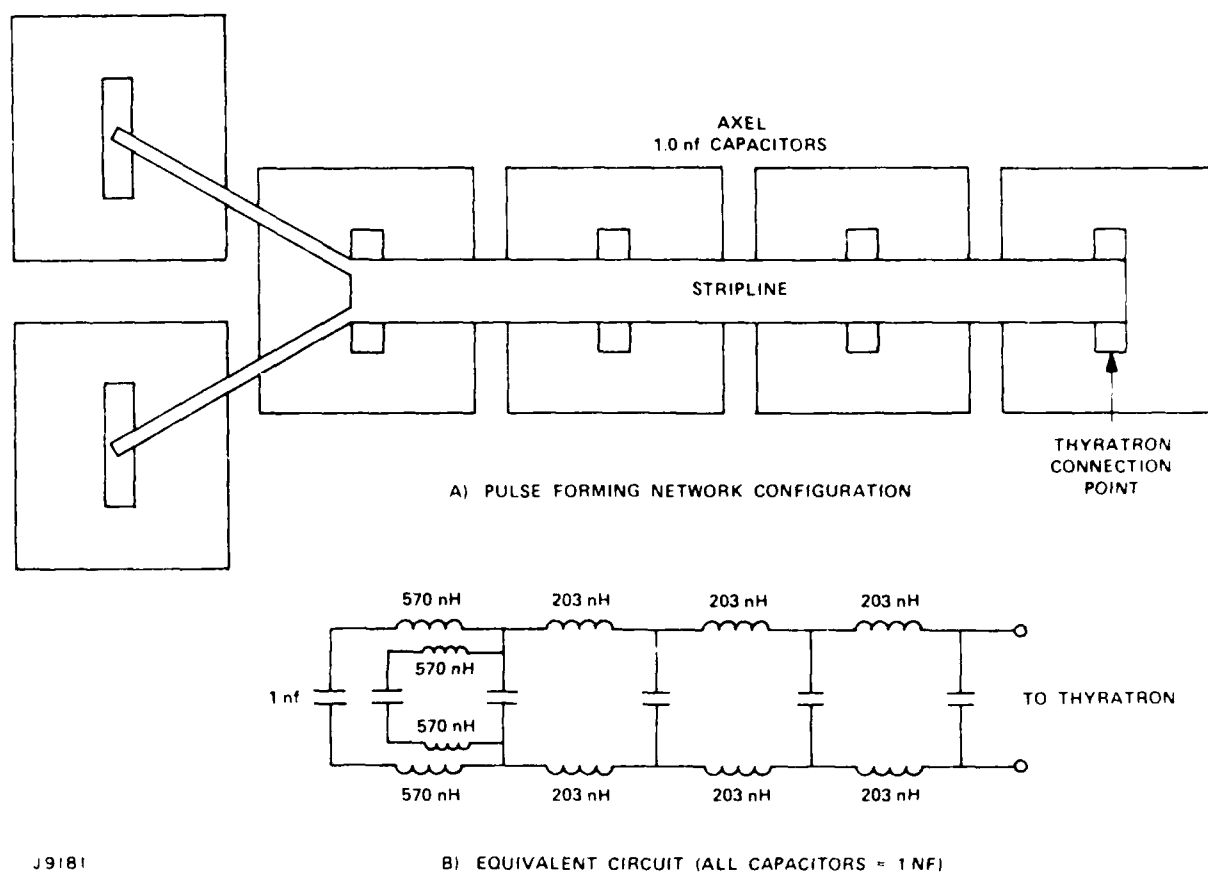
Figure 81. Conceptual Drawing of Pulse Forming Network Configuration
