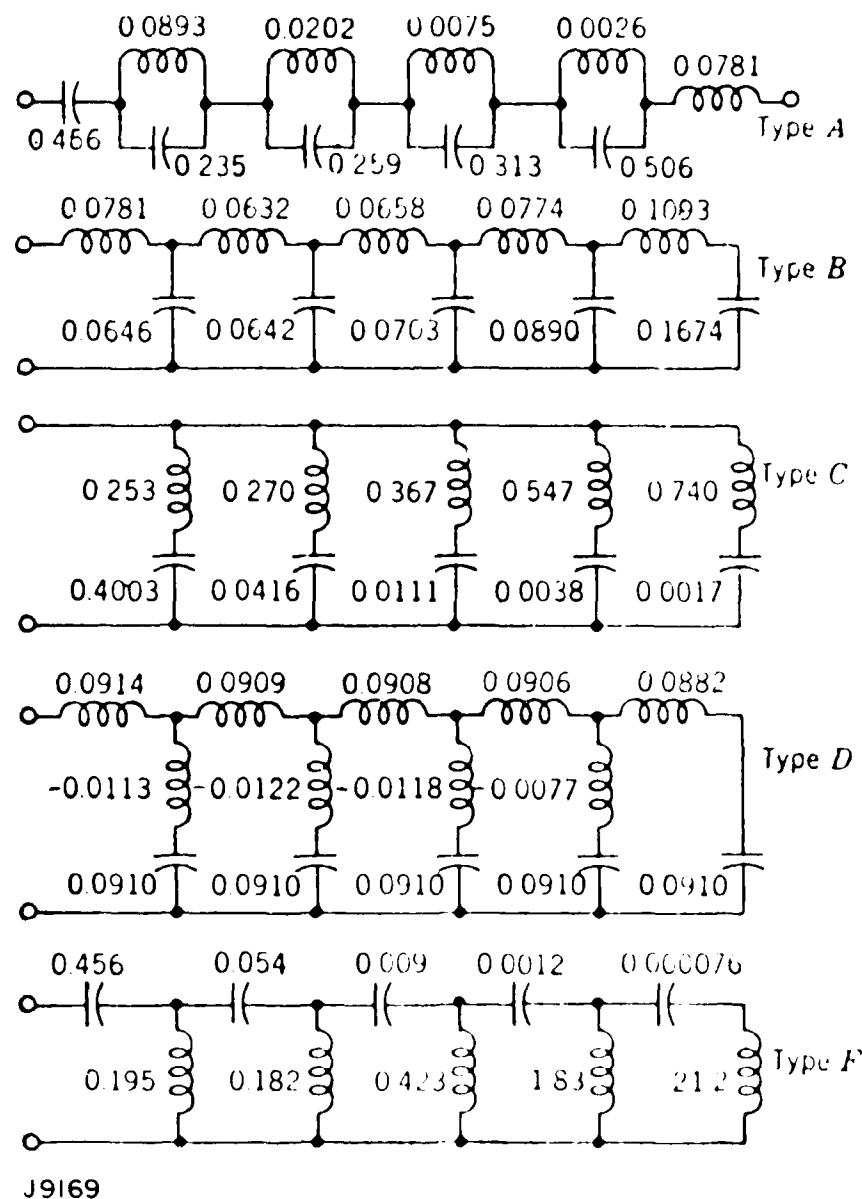
Figure 76. Equivalent Forms for Five-Section Guillemin Voltage-Fed Network. Multiply the values of the inductances by Z_N \tau and the values of the capacitances by \tau / Z_N . The inductances are in henrys and the capacitances in farads if pulse duration \tau is expressed in seconds and network impedance Z_N in ohms. (Adapted from "Pulse Generators," G.N. Glasoe and J.V. Lebacqz, Boston Technical Publishers, Lexington, MA 1964.)
