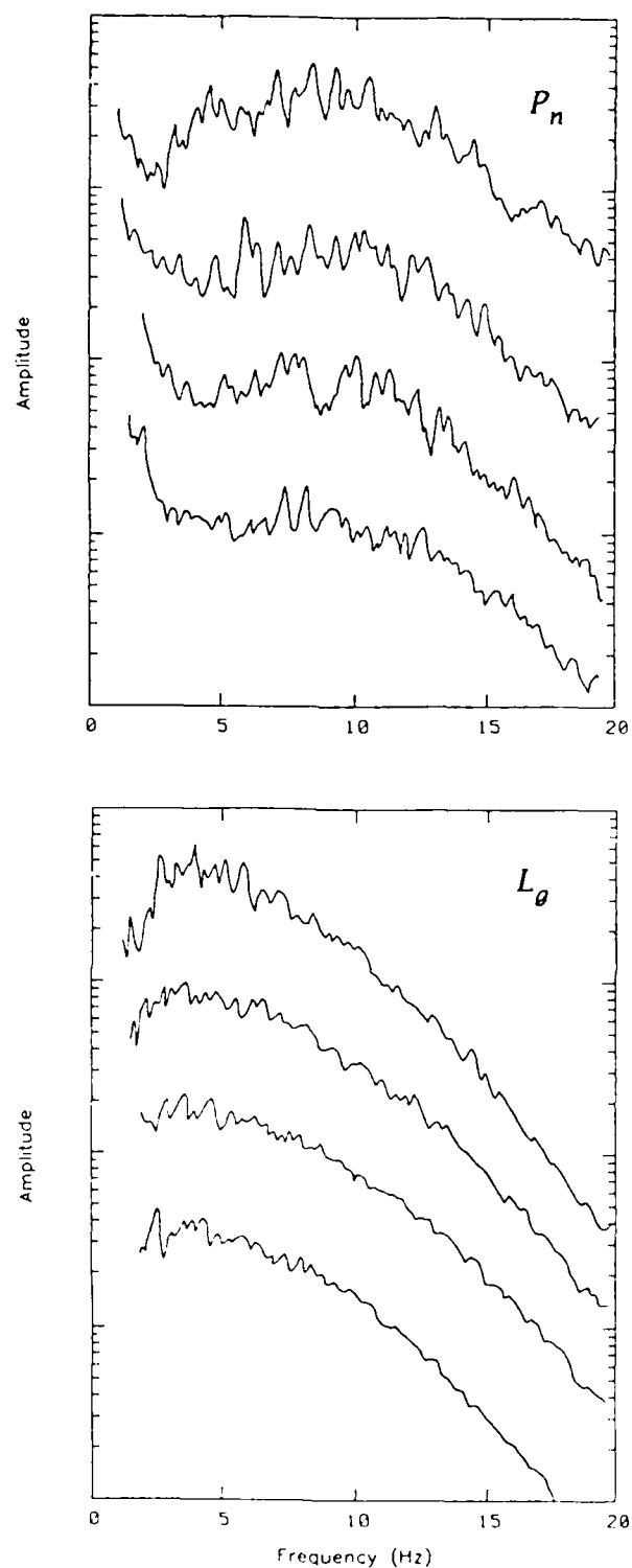
Figure 6. P_n and L_\theta spectra from four earthquakes off the west coast of Norway. Note the simplicity and similarity of the spectra for these four events, even though they are not located at the same source area.
