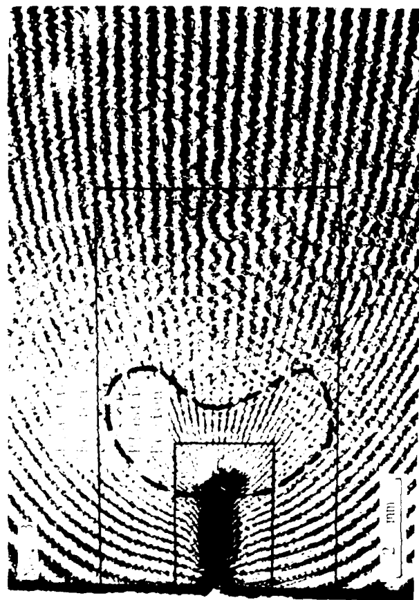
Applied Load: 1.78 kN Crack Extension: 0.18 mm
