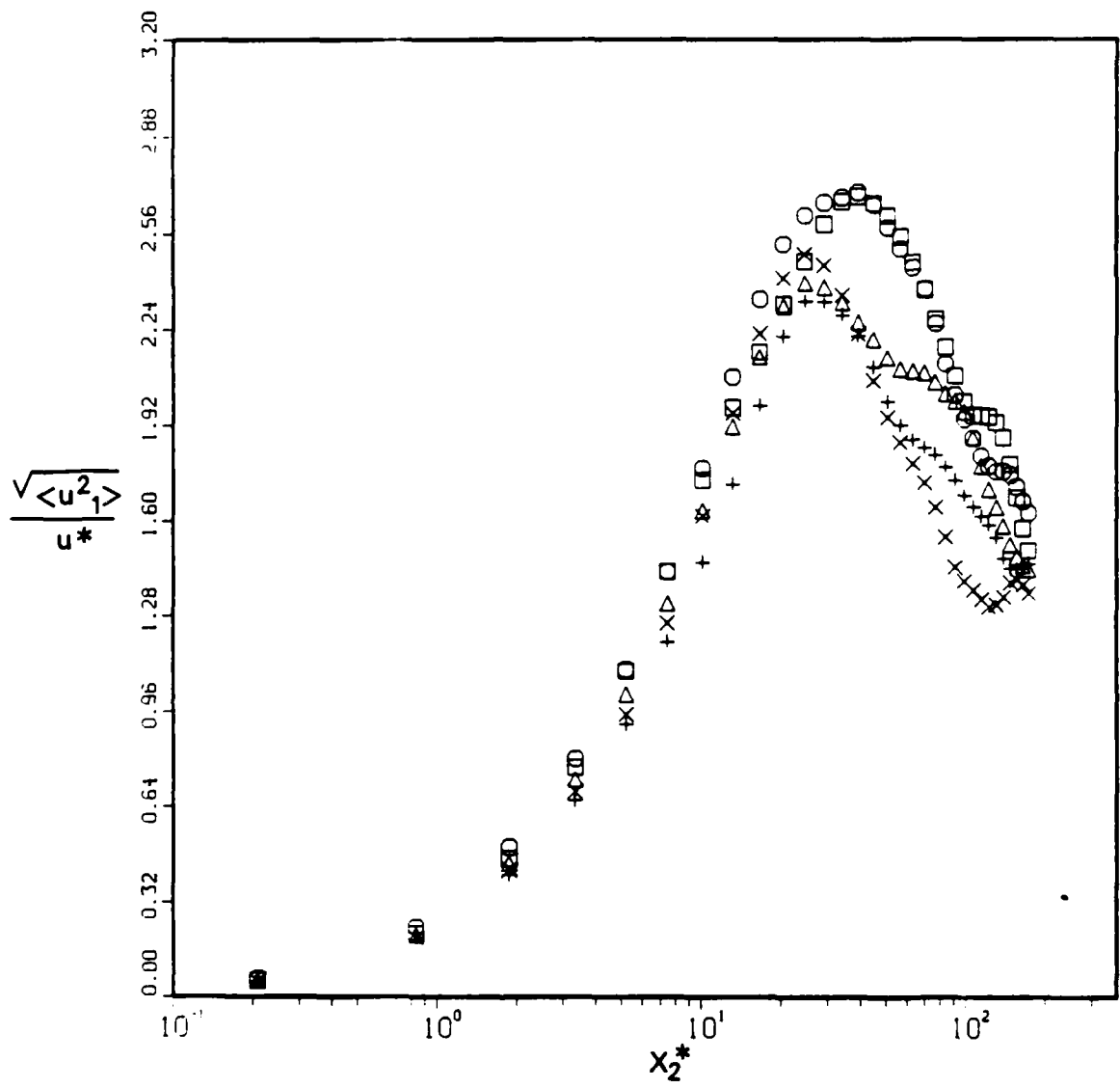
Fig. A2 — Root mean square streamwise velocity versus distance from the wall.
