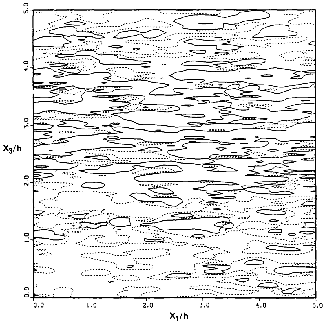
Fig. 8(a) — Contour plots of constant streamwise velocity at x_2^* = 1.86 . Contour levels for figures 8 (a-d) are: Solid line (u_1 - \langle u_1 \rangle) - (1/4)u_1' , -----, (u_1 - \langle u_1 \rangle) - u_1' .
