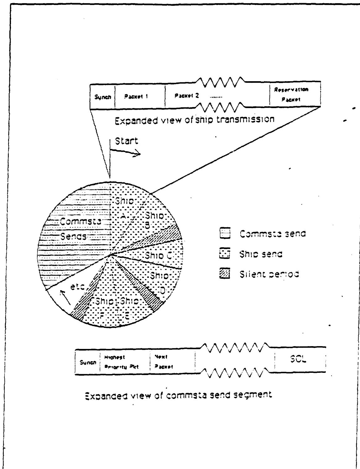
Figure 4.7 Revised Simplex Polling Circle.
