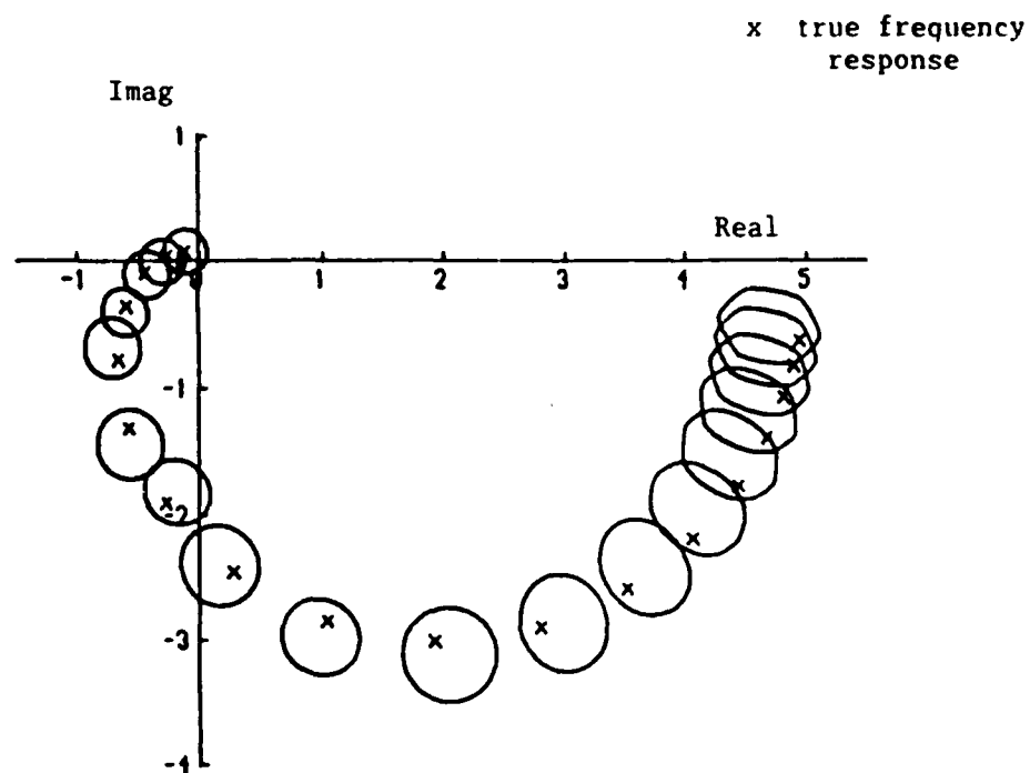
Figure 6.3: Frequency Response Uncertainty Bounds (Model Order q_{opt} = 18 ; Frequency-Dependent Bias Bounds)
