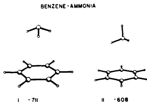
FIG. 10. Minimum energy configurations and binding energies for benzene ( \text{NH}_3 ) 3 , as obtained using a LJ potential calculation.
