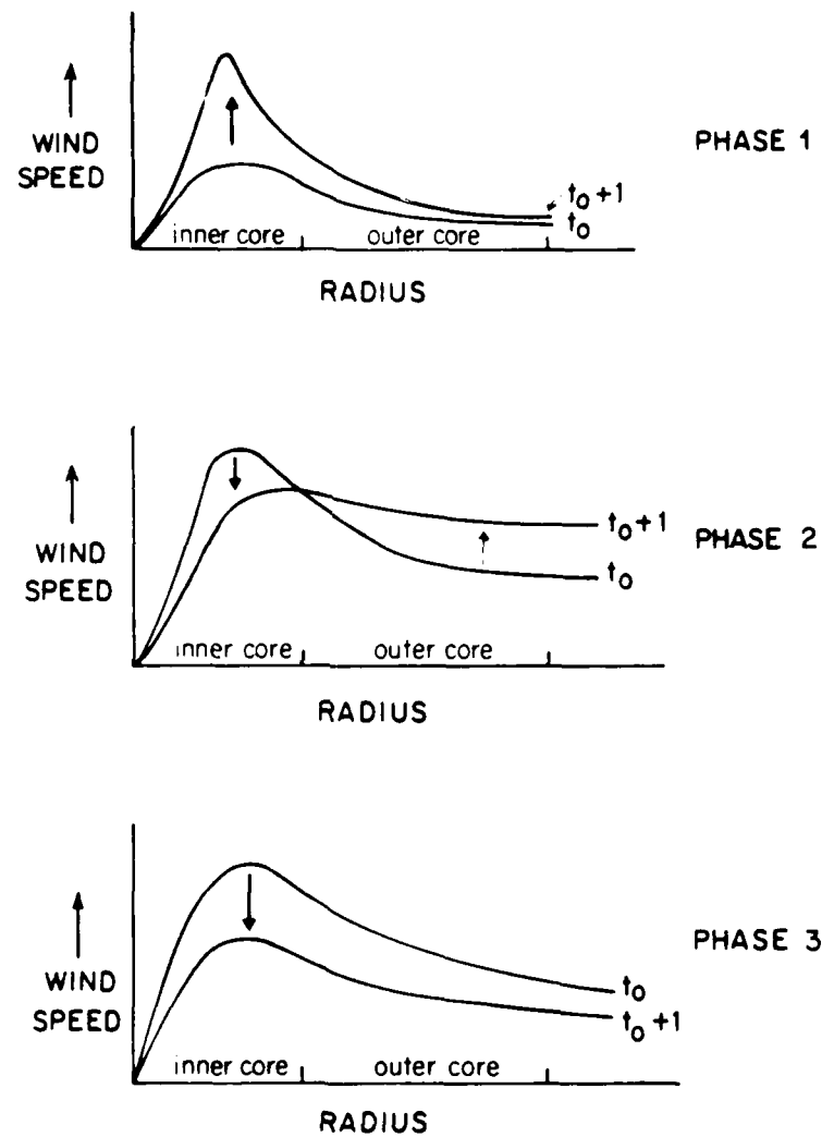
Figure 5.8: Schematic of the three possible wind profile phases where in phase 1 the inner core intensifies as the outer core strengthens, phase 2 depicts inner core filling and outer core strengthening, and in phase 3 the inner core fills as the outer core weakens.
