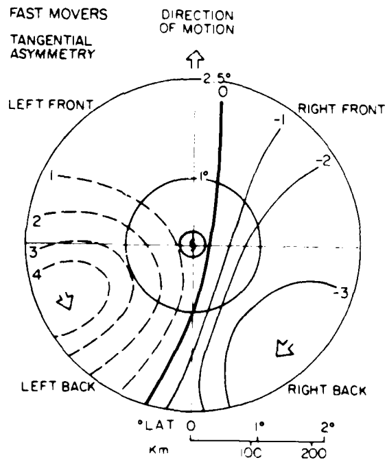
Figure 4.19: a-b. Plan-view depictions of the tangential asymmetry pattern in \text{ms}^{-1} and in MOTROT-VORT for the classes of slow moving cyclones (less than 2.5 \text{ ms}^{-1} ) and fast moving cyclones (speed greater than 7.5 \text{ ms}^{-1} ).
