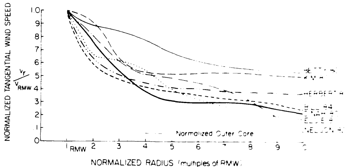
Figure 2.16: Normalized tangential wind profiles in which radius varies as multiples of RMW and wind speed values are a fraction of the maximum wind value. A comparable outer core extends from 4 to 10 times the RMW.
