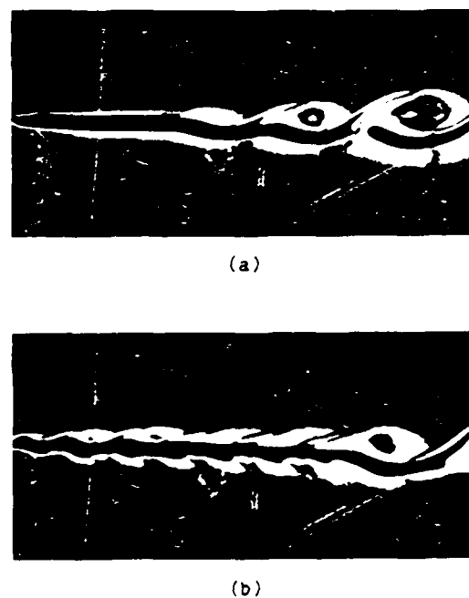
Fig. 10 Schlieren photographs of the shear layer mode (a) and the wake mode (b). Flow is from left to right with high-speed stream on top ( U_2/U_1 = 0.38 , \rho_2/\rho_1 = 10 ).
