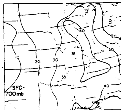
Fig. 31. VAS-estimated precipitable water for three layers--surface-700 mb, 700-500 mb, and 500-300 mb. The value 13 represents 1.3 cm.
