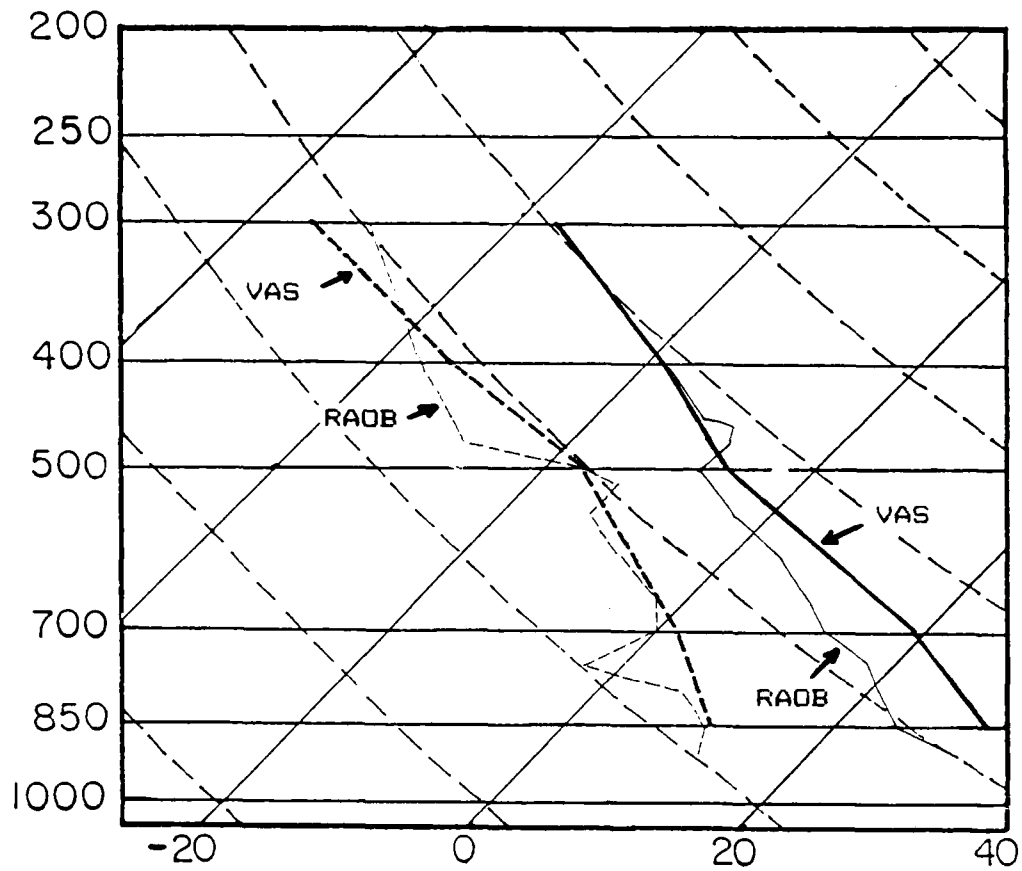
Fig. 11. Skew T-log P diagram of the VAS profile having the worst temperature agreement with its nearby radiosonde profile. It also had the best agreement with the point temperatures. The location was Rapid City at 0500 GMT. Solid lines represent VAS - RAQB profiles.
