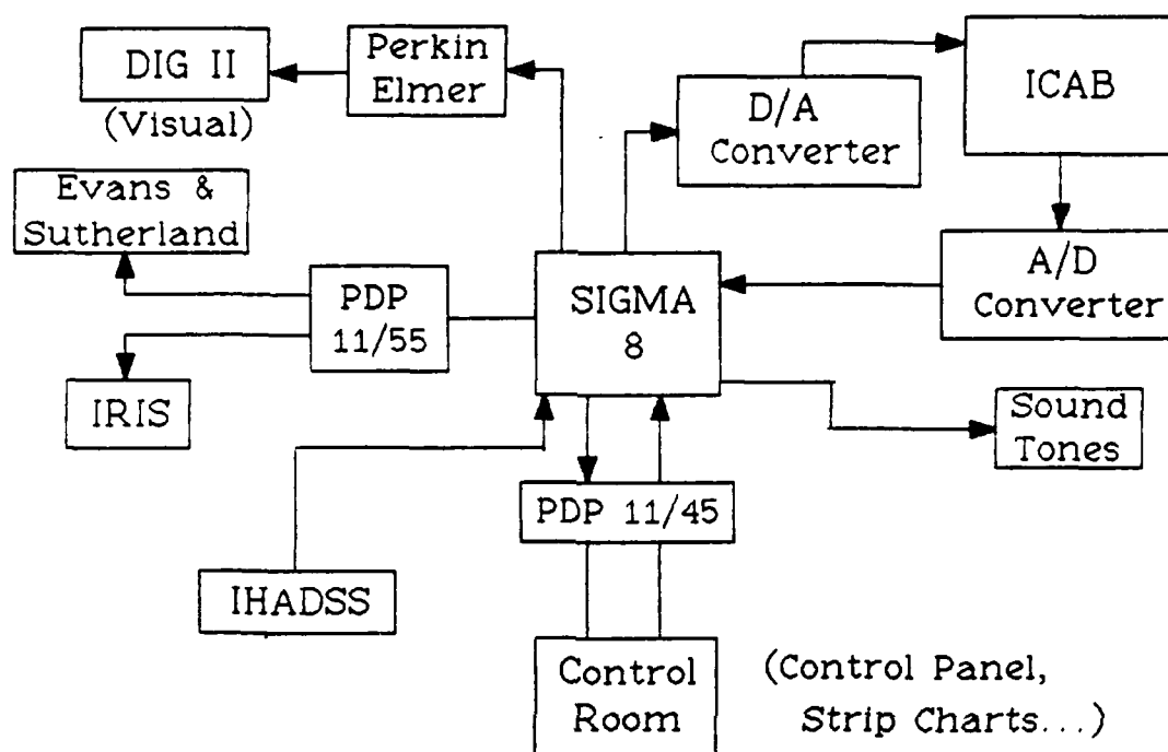
Figure 9.4 OATS Hardware
