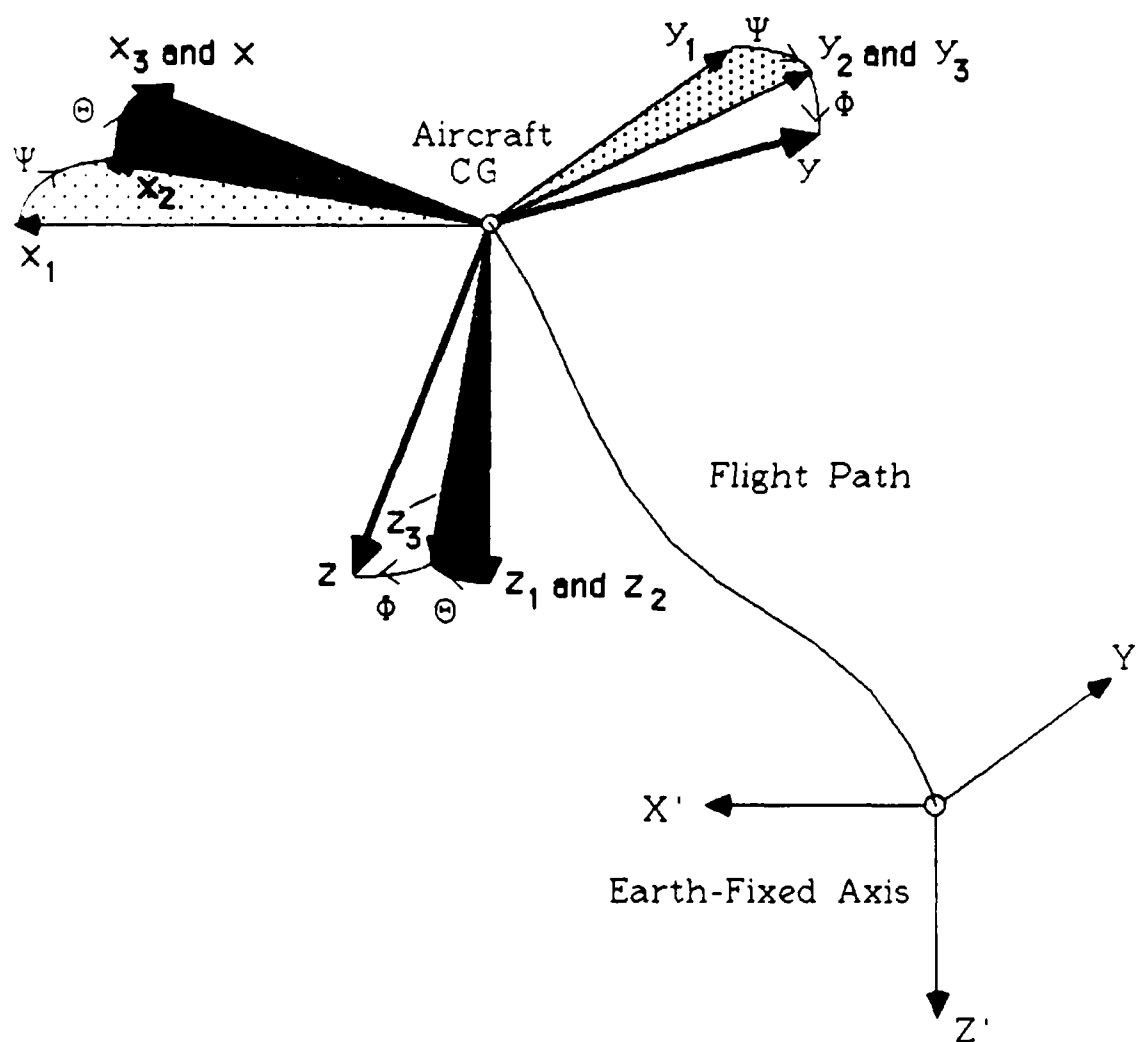
Figure 8.3 Euler Angles
