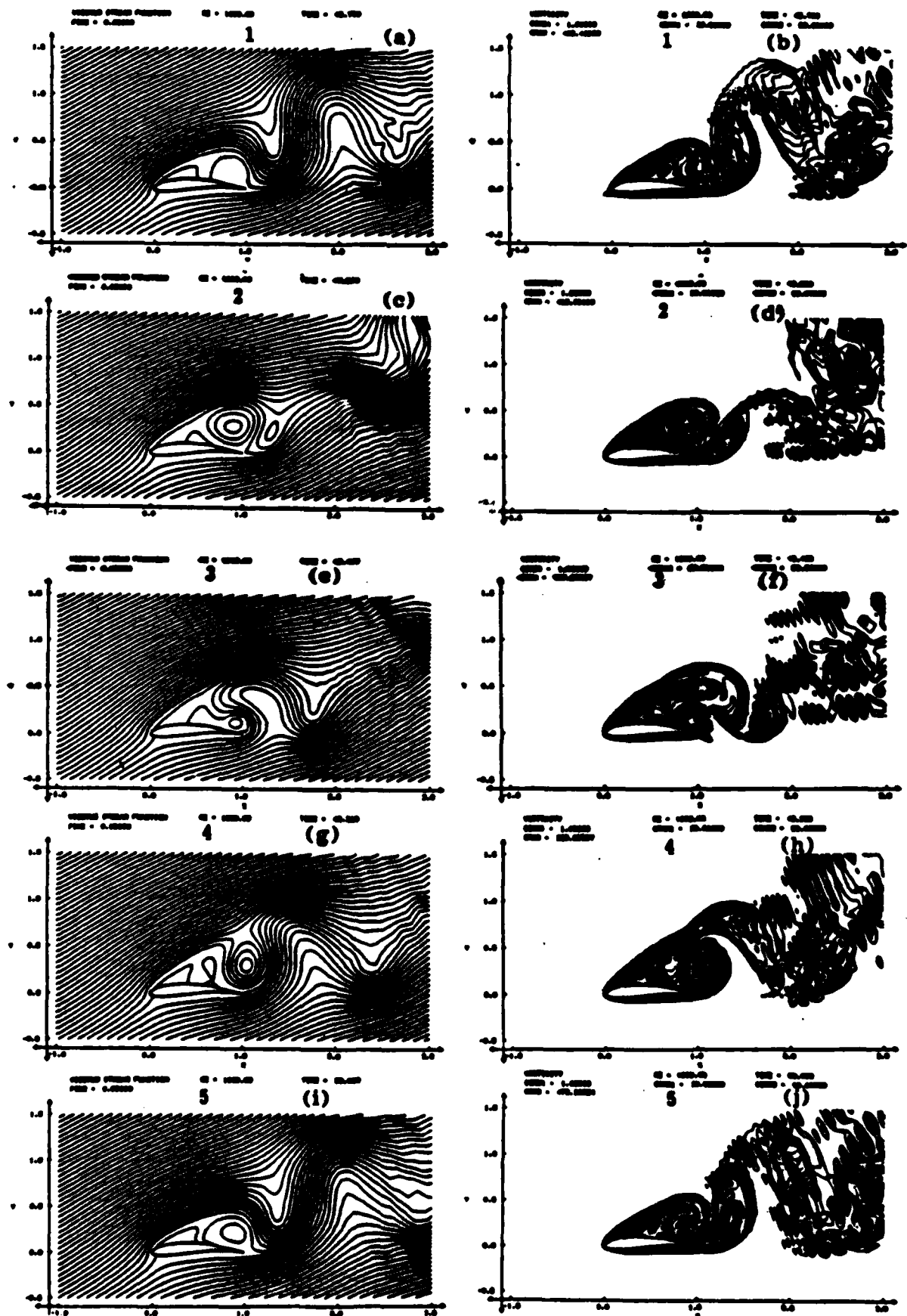
Fig. 16. TE-LE-TE Vortex-Shedding Cycle for Göttingen 580 Airfoil at Re = 1000 , \alpha_0 = 30^\circ .
