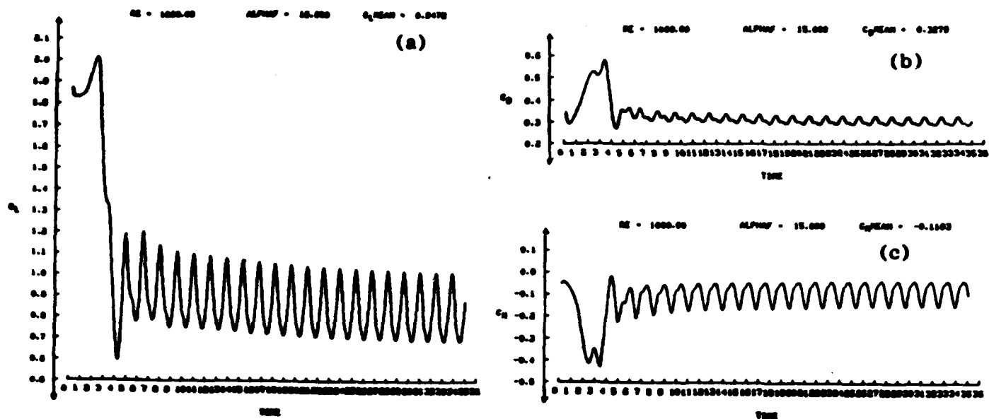
Fig. 9. Instantaneous Aerodynamic Coefficients at Re = 1,000 , \alpha_f = 15^\circ .
