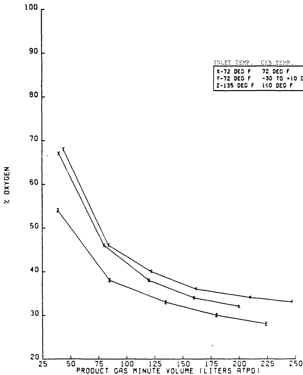
Figure 13. The B-1B MSOGS oxygen output at ground level with inlet air pressure at 25 psig, and temperatures as noted in figure.
