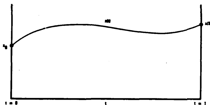
FIG. 1. Homotopic Continuation
