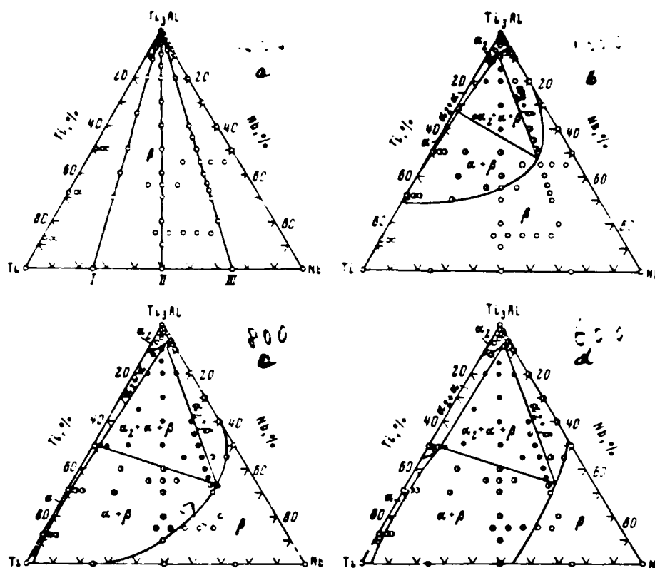
Fig. 1. Composition of investigated alloys (a) and isothermic cross sections of system Ti-Ti 3 Al-Nb (a-d). T, °C: a - 1200, b - 1000, c - 800, d - 600.
