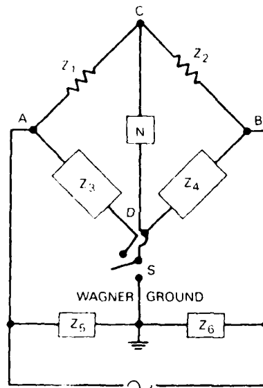
Figure 6. Wagner Ground in an AC Bridge Circuit. It consists of impedances Z_5 and Z_6 and the switch S .
