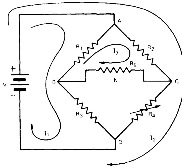
Figure 4. Wheatstone Bridge Circuit. Source V energizes the bridge. The null detector is represented by R_5 . Ratio arms are R_1 and R_2 . R_3 is an unknown resistance inserted for measurement. Loop currents for analysis of the circuit are also shown.
