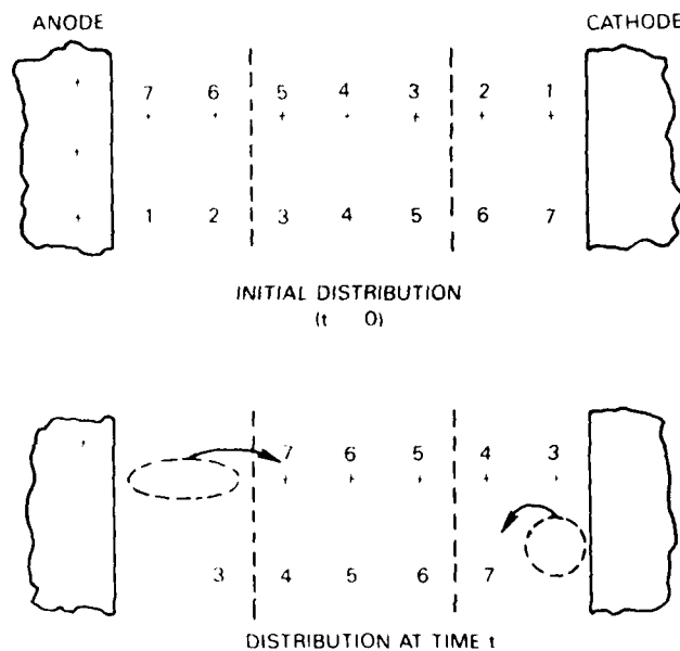
Figure 1. Transport of Charge by Migration. Electrical double layers at electrode surfaces are omitted. At t = 0 , there are equal numbers of positive and negative ions throughout the bulk solution. In time t , two cations and two anions are discharged by electrolysis. If the cations are assumed to have a mobility twice that of the anions, both cations are replaced at the cathode but only one anion is replaced at the anode. Any ionic species not electrolyzed simply tends to accumulate at the electrodes.
