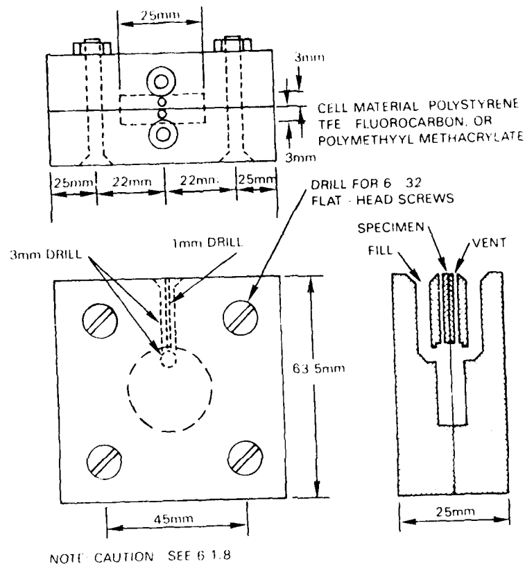
Figure 13b. Mercury Cell for Thin Sheet Material.
