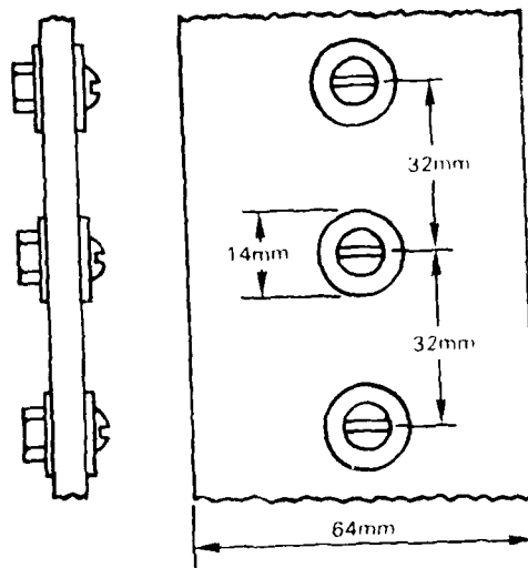
Figure 7. Binding-Post Electrodes for Flat, Solid Specimens.
