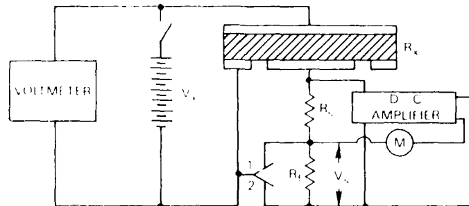
Figure 16. Voltmeter-Ammeter Method Using DC Amplification. Normal use of amplifier and indicating meter.
