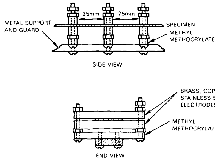
Figure 9. Strip Electrodes for Tapes and Flat, Solid Specimens.
