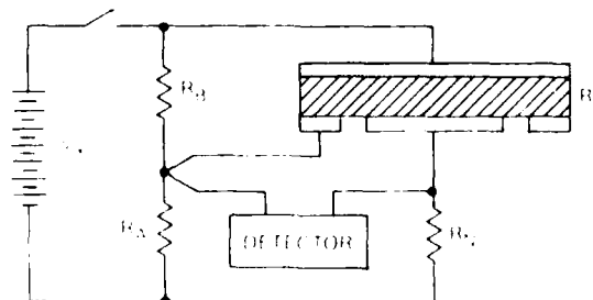
Figure 18. Comparison Method Using a Wheatstone Bridge.
