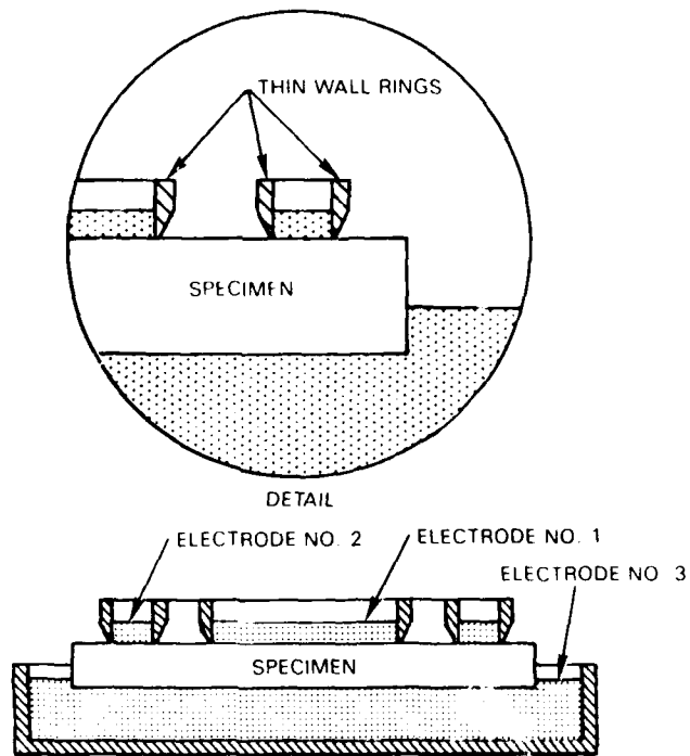
Figure 13a. Mercury Electrodes for Flat, Solid Specimens.
