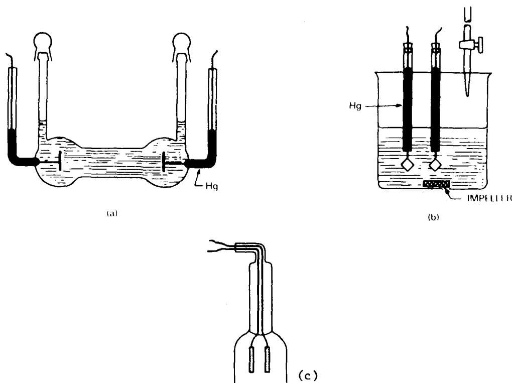
Figure 3. Some Types of Conductance Cells. (a) Jones and Bollinger precision cell, (b) Titration cell, and (c) Dip-type cell.
