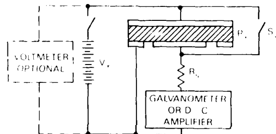
Figure 17. Comparison Method Using a Galvanometer.
