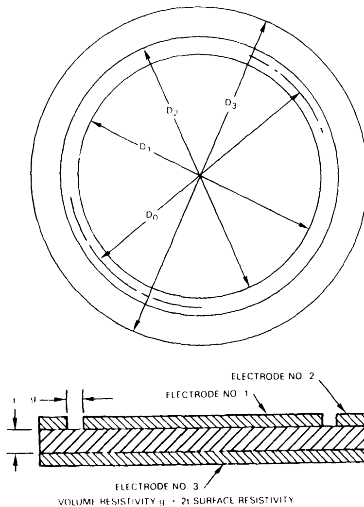
Figure 10. Flat Specimen for Measuring Volume and Surface Resistances or Conductances.
