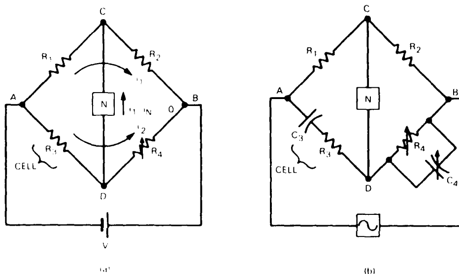
Figure 5. Wheatstone Bridge Circuit in Two Versions. In each, R_1 and R_2 are ratio arms and N is a Suitable Null Detector. (a) Simple bridge. (b) Alternating-current conductance bridge. The C_4 - R_4 combination provides adequate compensation for both resistance and capacitance of the conductivity cell under most conditions.
