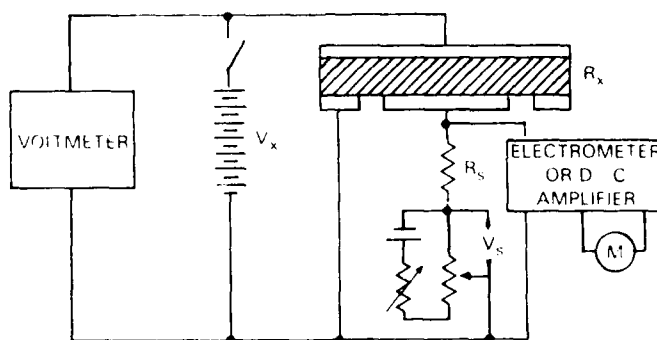
Figure 14. Voltmeter-Ammeter Method Using DC Amplification. Amplifier and indicating meter as null detector.
