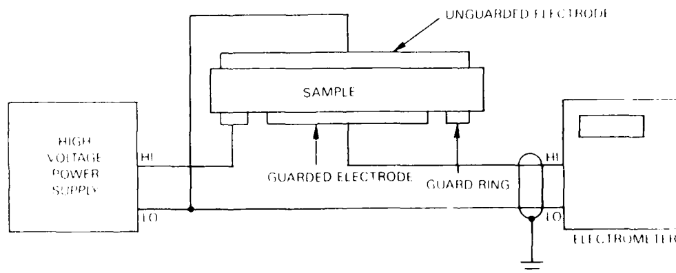
Figure 19. Surface Resistivity Electrical Diagram.
