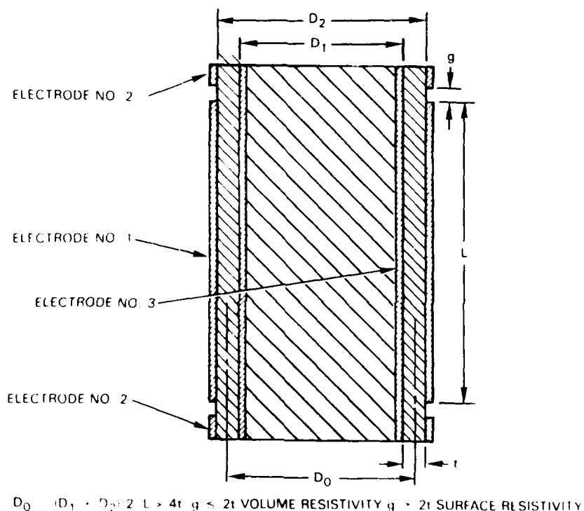
Figure 11. Tubular Specimen for Measuring Volume and Surface Resistances or Conductances.
