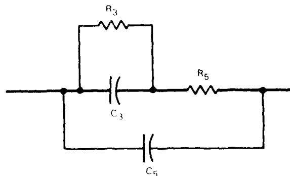
Figure 2. Schematic Representation of an AC Conductance Cell in Terms of its Equivalent Circuit. The simplest equivalent circuit is shown in bold lines. R_3 is the resistance of the bulk solution, C_3 represents the double-layer capacitance at the electrodes, R_5 is the faradaic resistance across the electrode double layer, and C_5 represents the capacitances of the cell electrodes, leads, etc.
