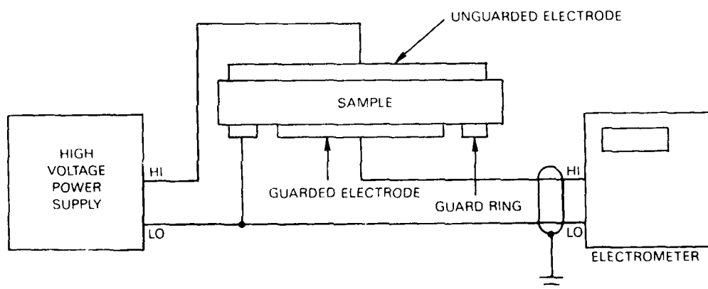
Figure 20. Volume Resistivity Electrical Diagram.
