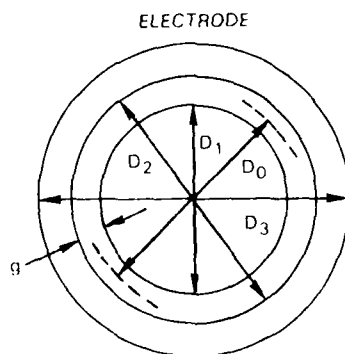
Figure 21. Electrode Configurations and Parameters Needed for the Geometric Calculations for Surface and Volume Resistivity.
