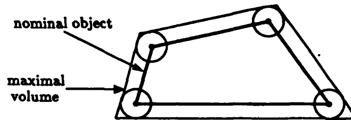
Figure 7.2: An object and its maximal volume under vertex uncertainty.
