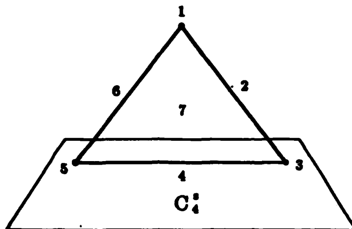
Figure 6.4: The set C_4^* of commanded positions which might cause the robot to stick in atom 4 if it reaches it.
