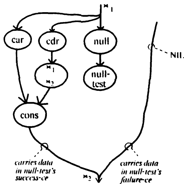
Figure 3.2: COPYLIST Program and Flow Graph
