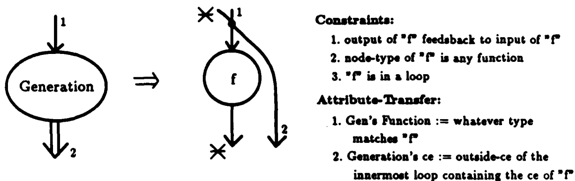
Figure 2.45: Rule for Generation Plan
