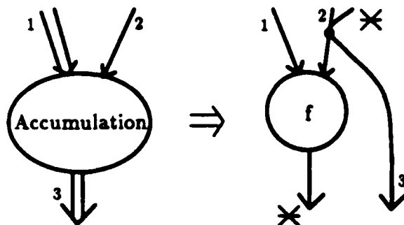
Figure 2.48: Rule for Accumulation
