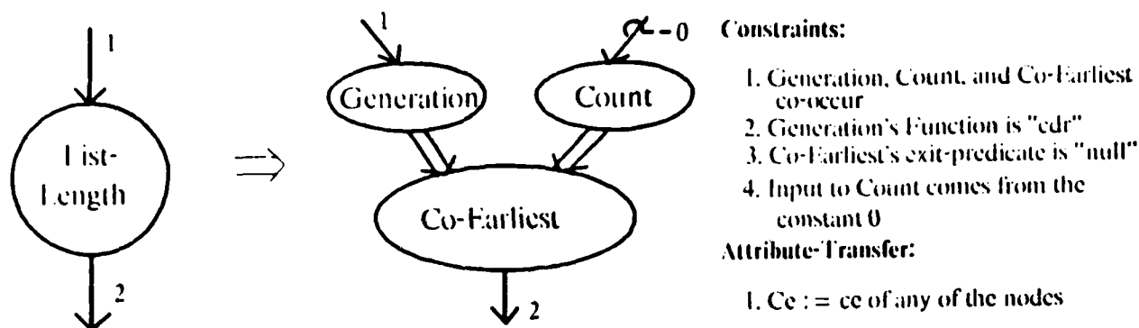
Figure 2.65: The Rule for List-Length
