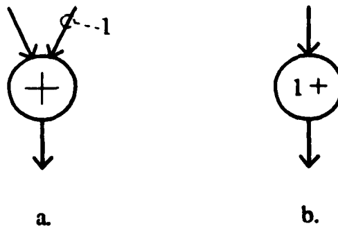
Figure 2.33: Two Graphs for Incrementing an Integer
