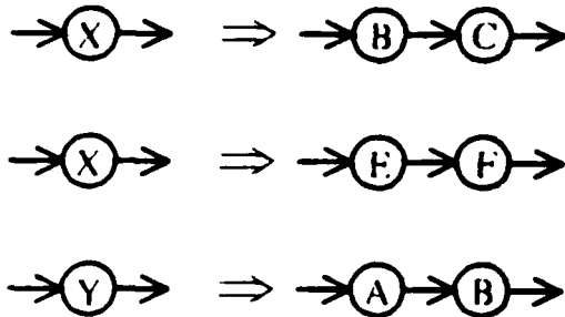
Figure 3.6: Grammar and Program Graph
