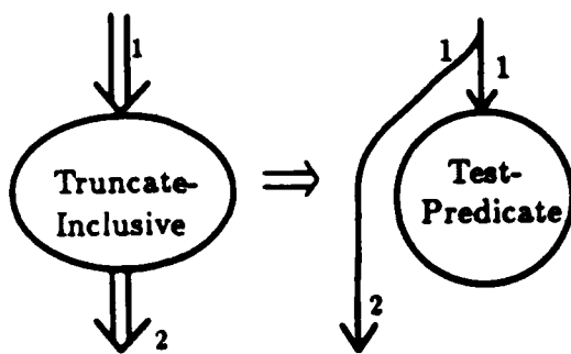
Figure 2.50: Rule for Truncate-Inclusive
