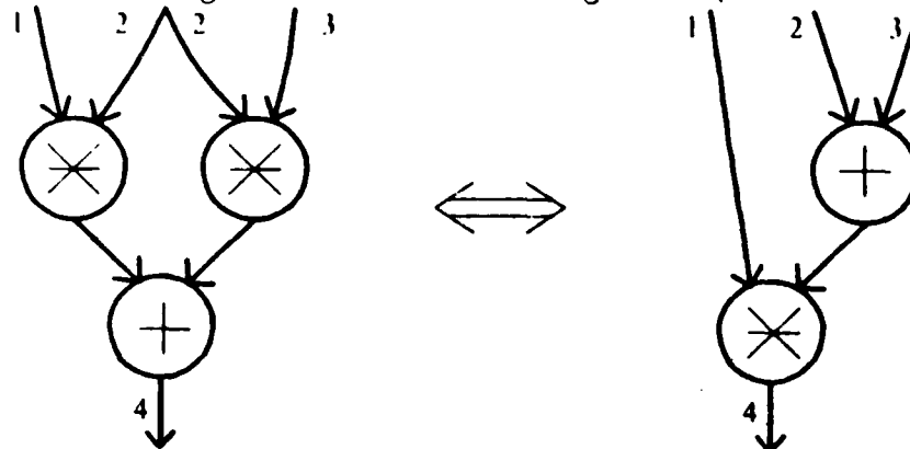
Figure 3.7: Transformation for the Distributive Law
