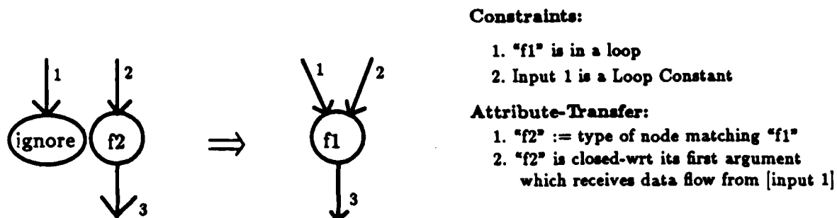
Figure 2.56: Rule for Dealing with a Loop Constant
