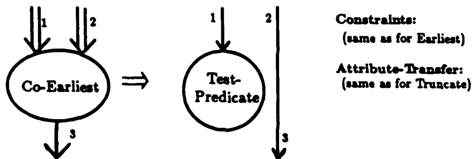
Figure 2.54: Rule for Co-Earliest
