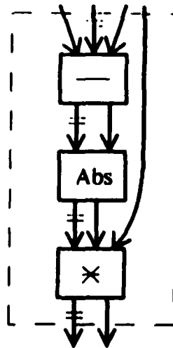
Figure 2.22: The Plan for MULTI-LENGTH
