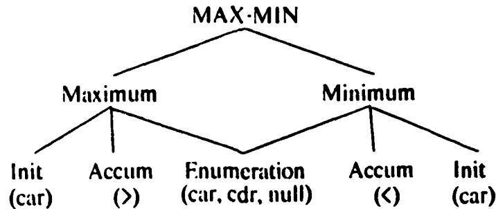
Figure 2.5: Parse Tree for the MAX-MIN program
