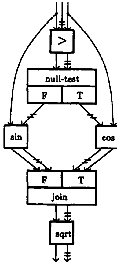
Figure 2.27: A Sample Plan Containing a Join
