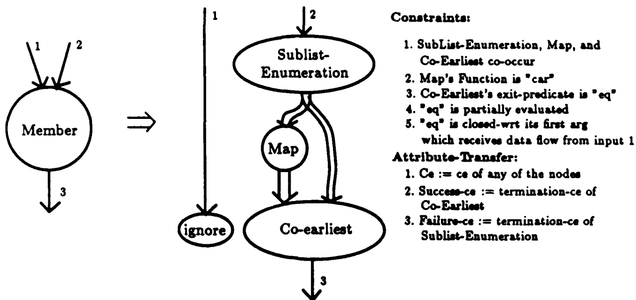
Figure 2.69: Rule for Member
