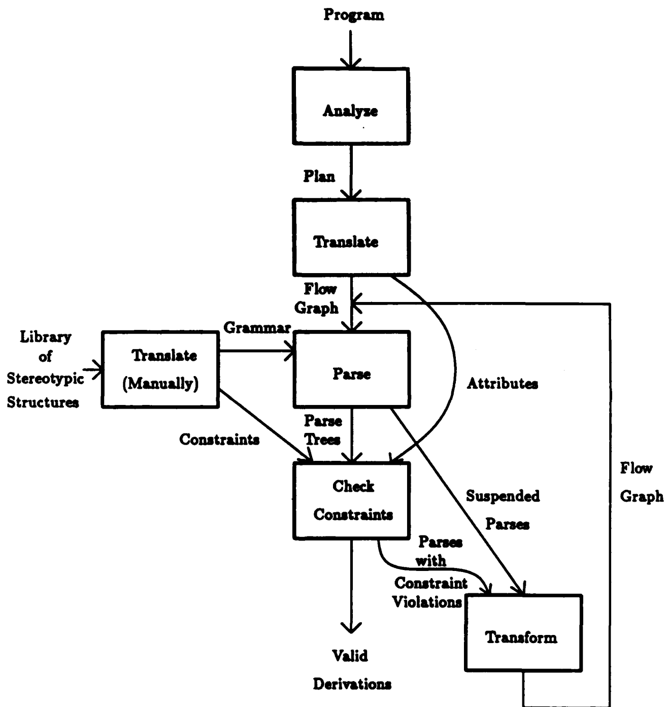
Figure 1.1: The Logical Structure of the Recognizer
