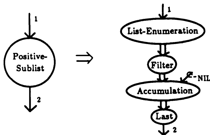
Figure 2.67: The Rule for Positive-Sublist
