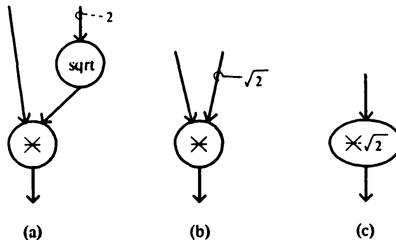
Figure 2.38: Recursively Incorporating a Constant into Operations
