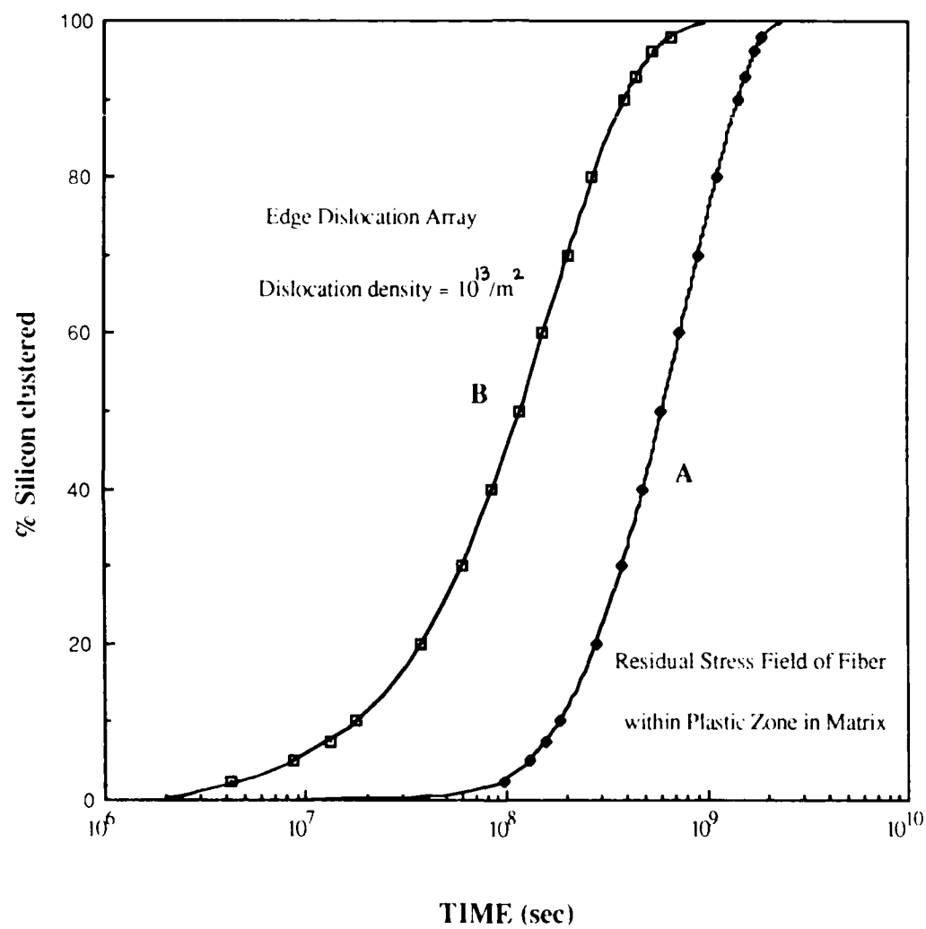
Figure 7: Comparative Si clustering rates on an edge dislocation array of density 10^{13}/m^2 and the residual stress field of the fiber in the composite at 100^\circ C .
