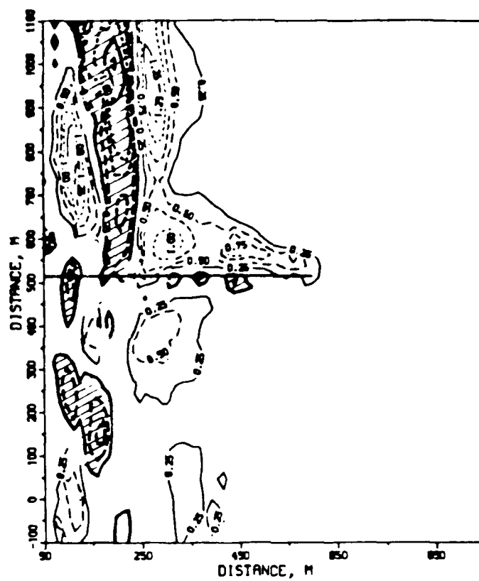
Figure A11. 28 September to 19 December change diagram
