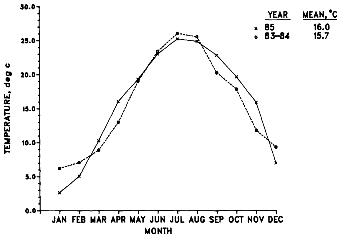
Figure 3. 1985 mean monthly air temperatures
