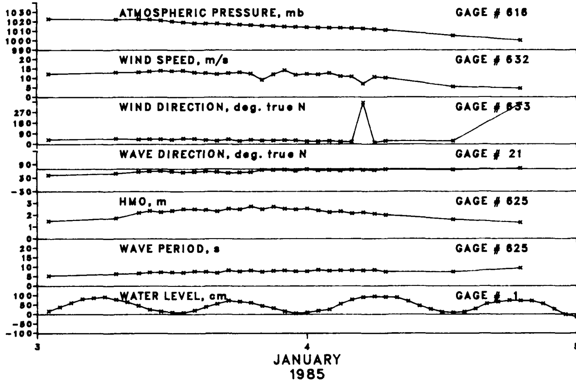
Figure B1. Storm data for 3-4 January 1985
