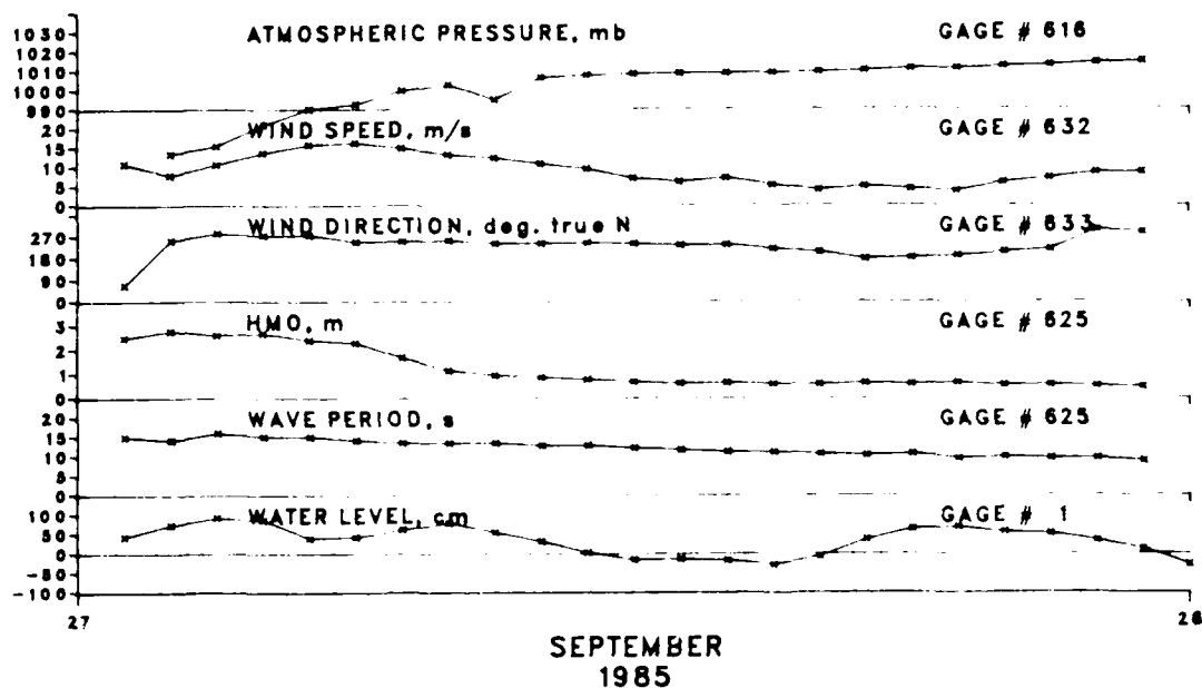
Figure B8. Storm data for 27 September 1985
