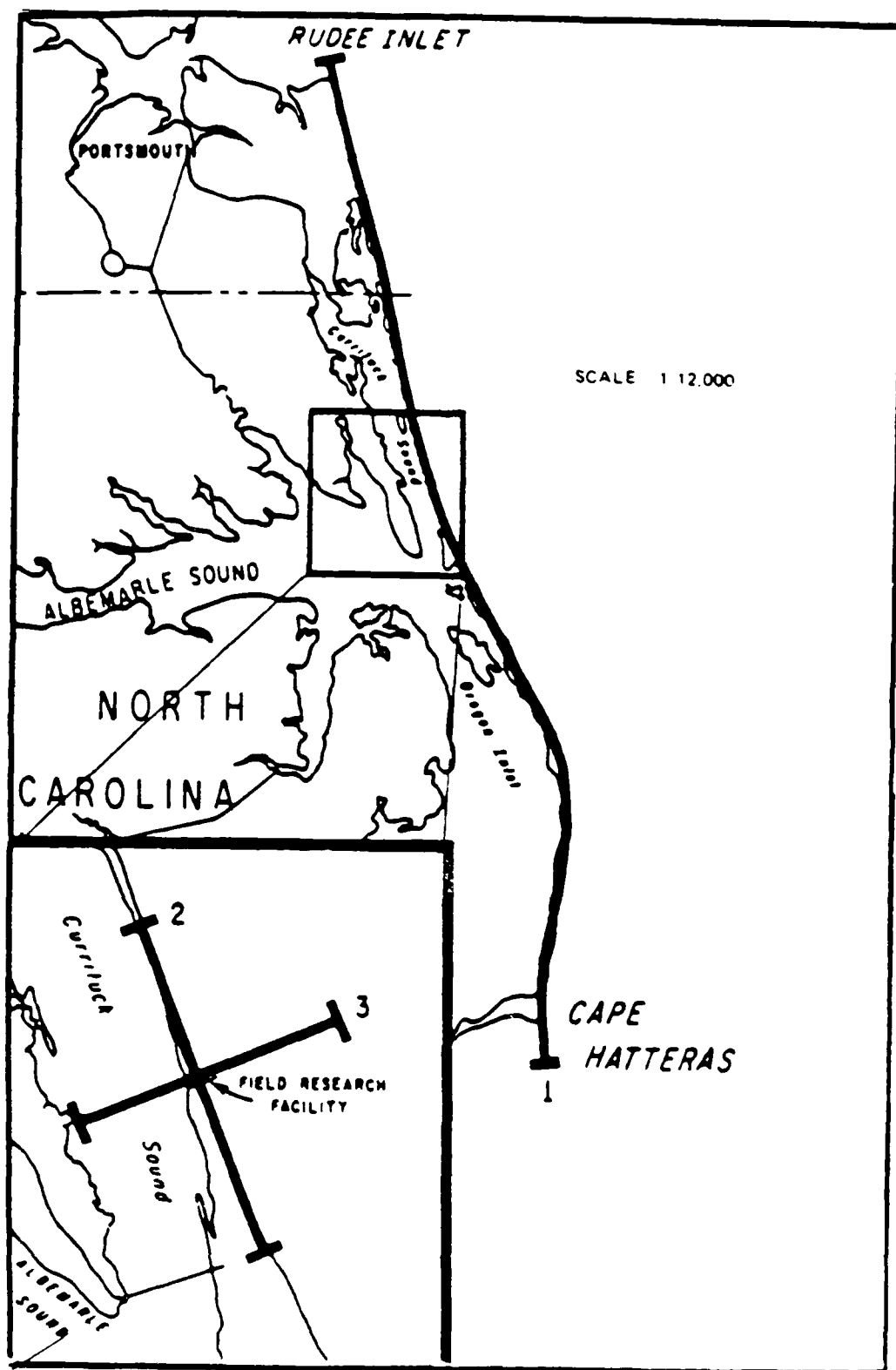
Figure 46. Aerial photography flight lines
