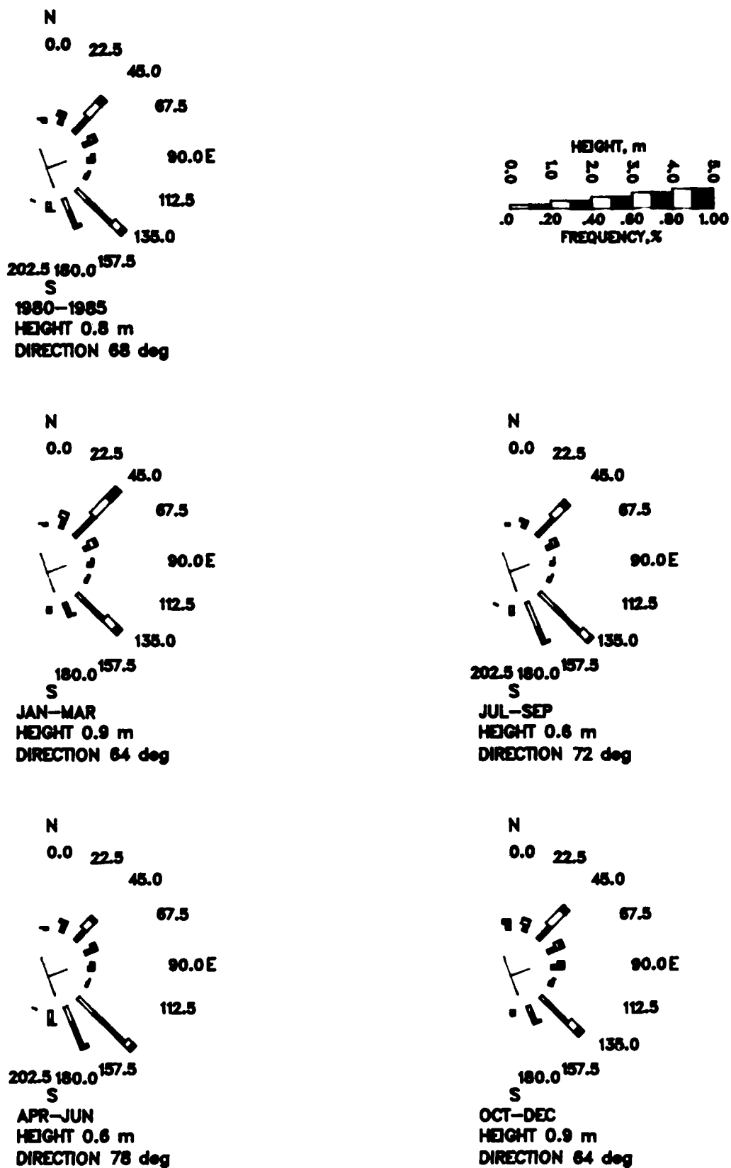
Figure 25. Annual and seasonal wave roses, 1980-1985
