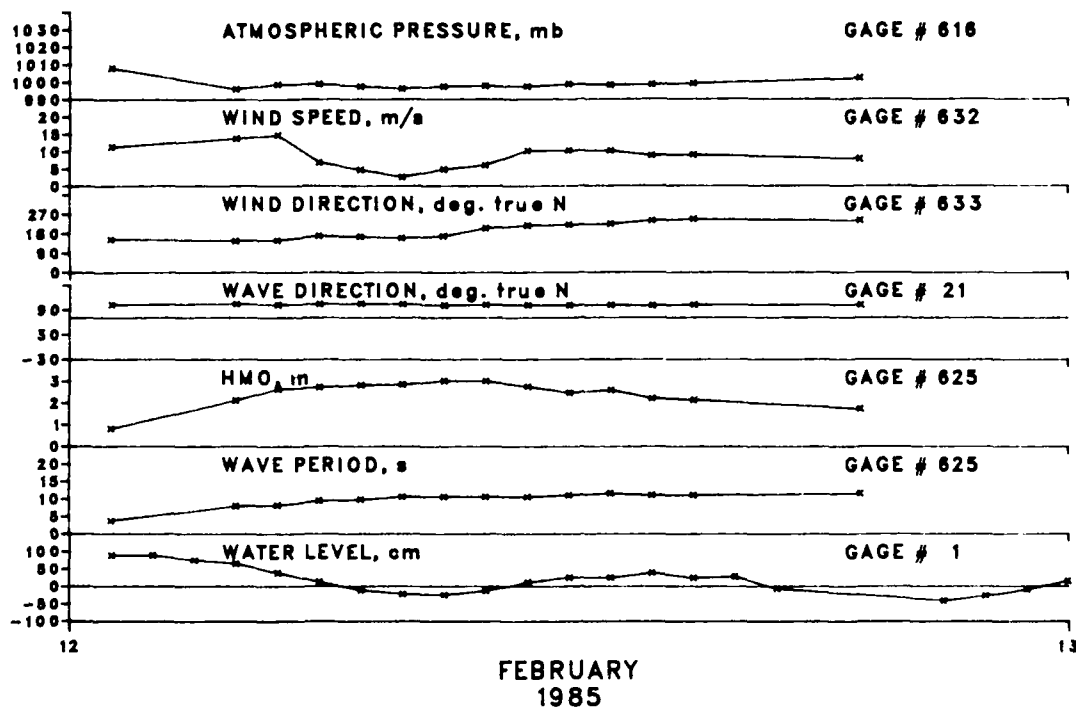
Figure B2. Storm data for 12 February 1985
