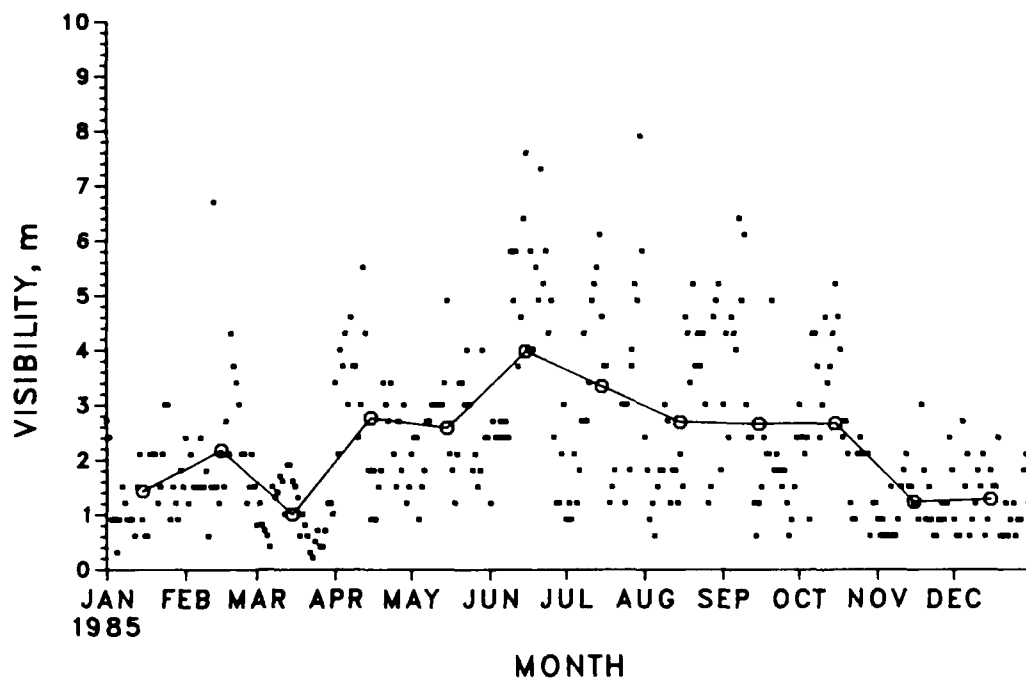
Figure 38. Daily sea surface water visibility, 1985
