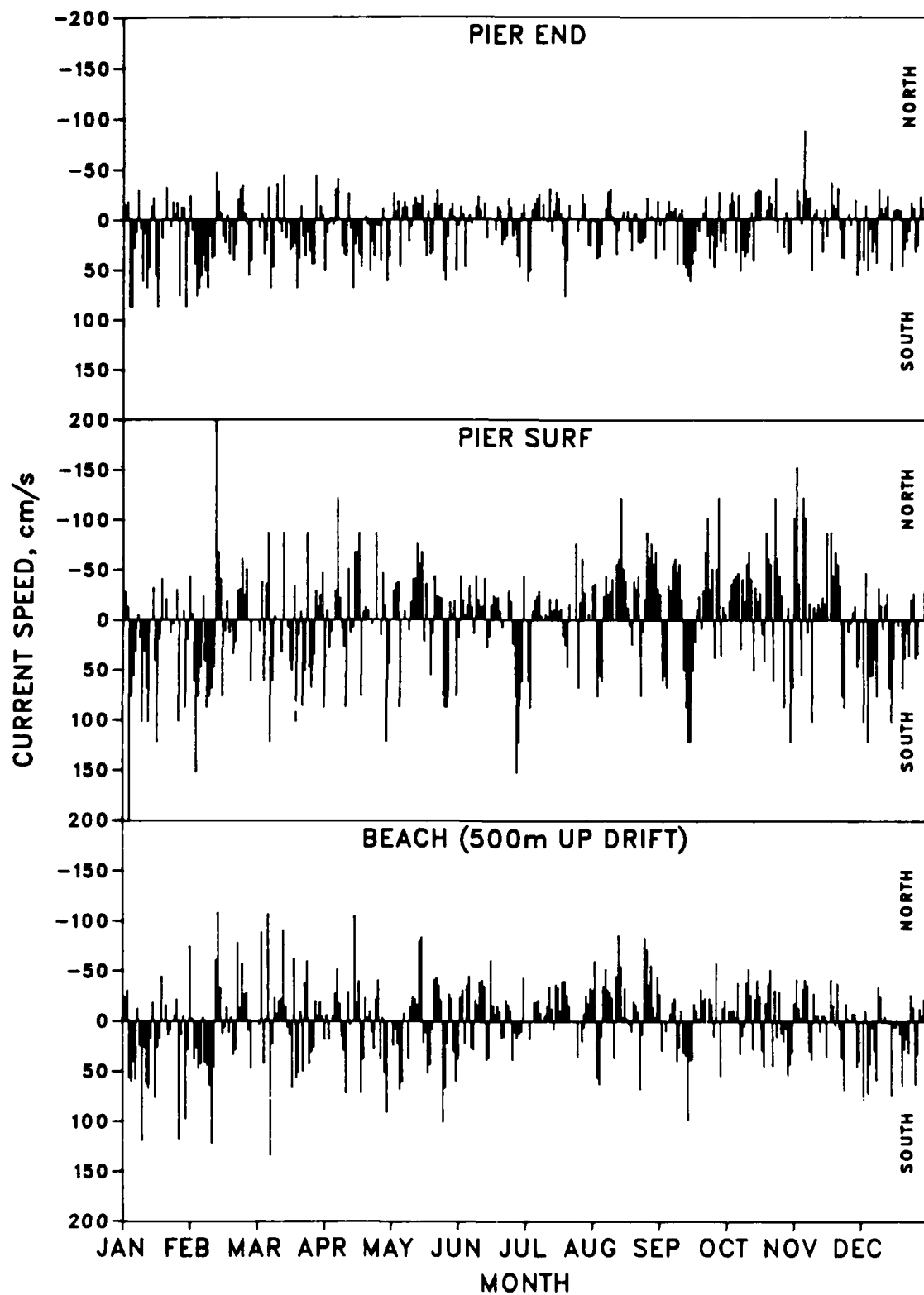
Figure 26. Daily surface currents, 1985
