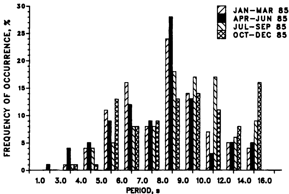
Figure 16. Seasonal wave period distributions for Gage 625, 1985
