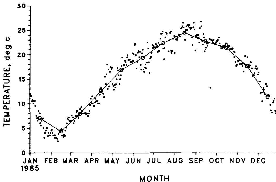
Figure 35. Daily sea surface water temperatures, 1985
