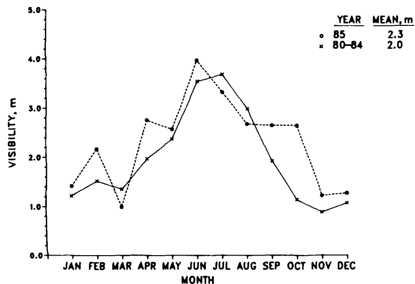
Figure 39. Comparison of mean surface water visibility
