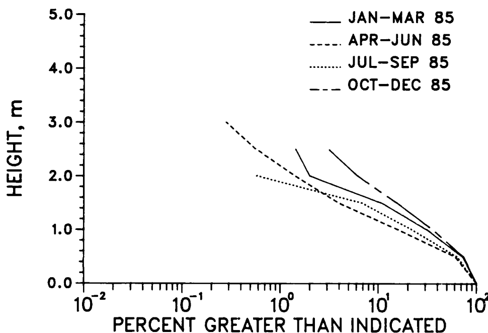
Figure 15. Seasonal wave height distributions for Gage 625, 1985
