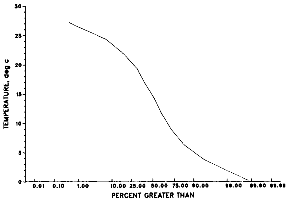
Figure 37. Distribution of surface water temperatures, 1980-1985
