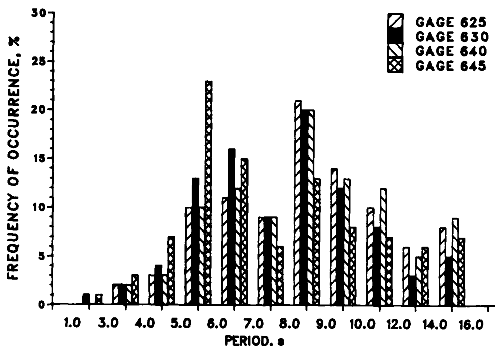
Figure 12. Annual wave period distributions, 1985
