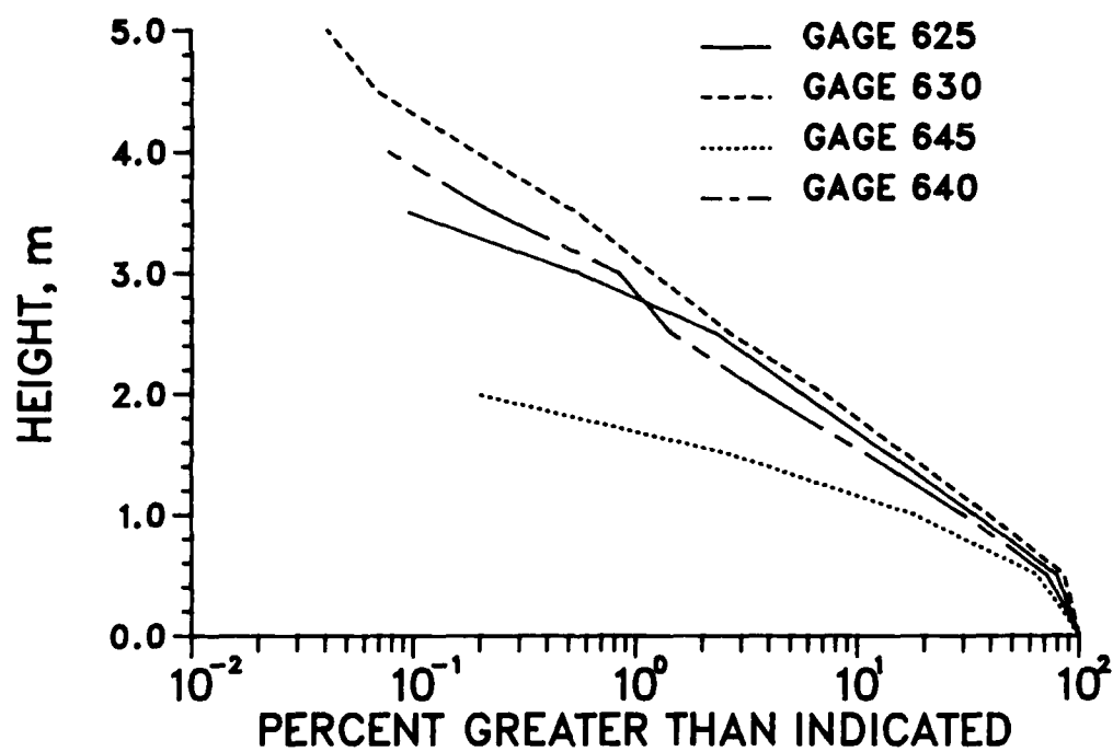
Figure 21. Annual wave height distributions, 1980-1985
