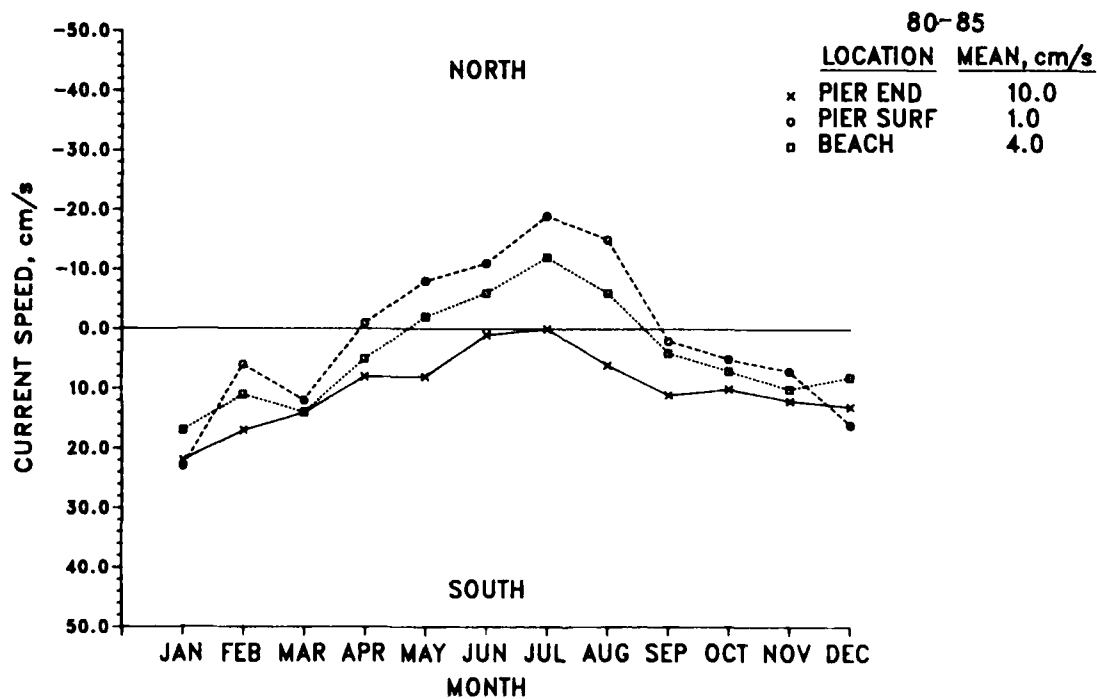
Figure 31. Mean surface currents, 1980-1985
