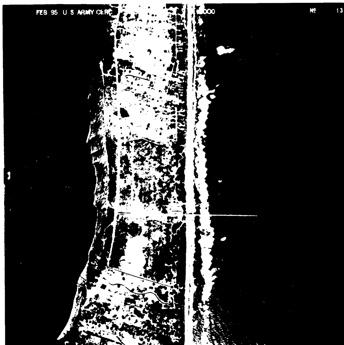
Figure 47. Sample aerial photograph taken 9 February 1985
