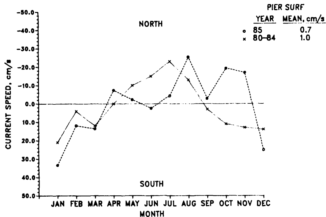
Figure 29. Comparison of surface currents at the midsurf
