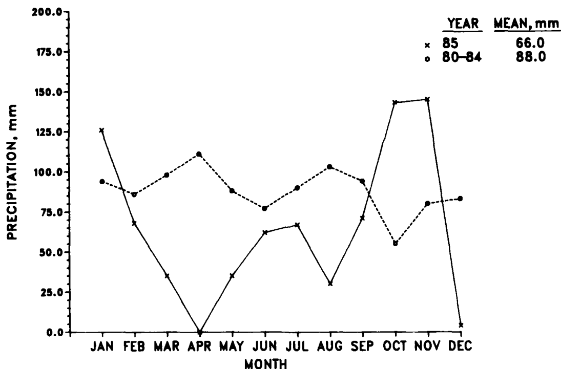
Figure 5. Mean monthly precipitation
