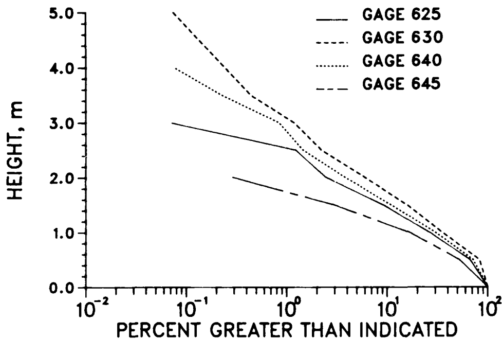
Figure 11. Annual wave height distributions, 1985
