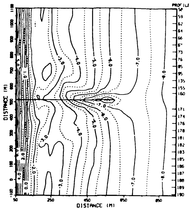
Figure A1. 14 February bathymetry
