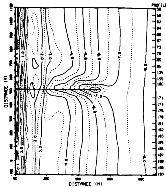
Figure A4. 15 July bathymetry
