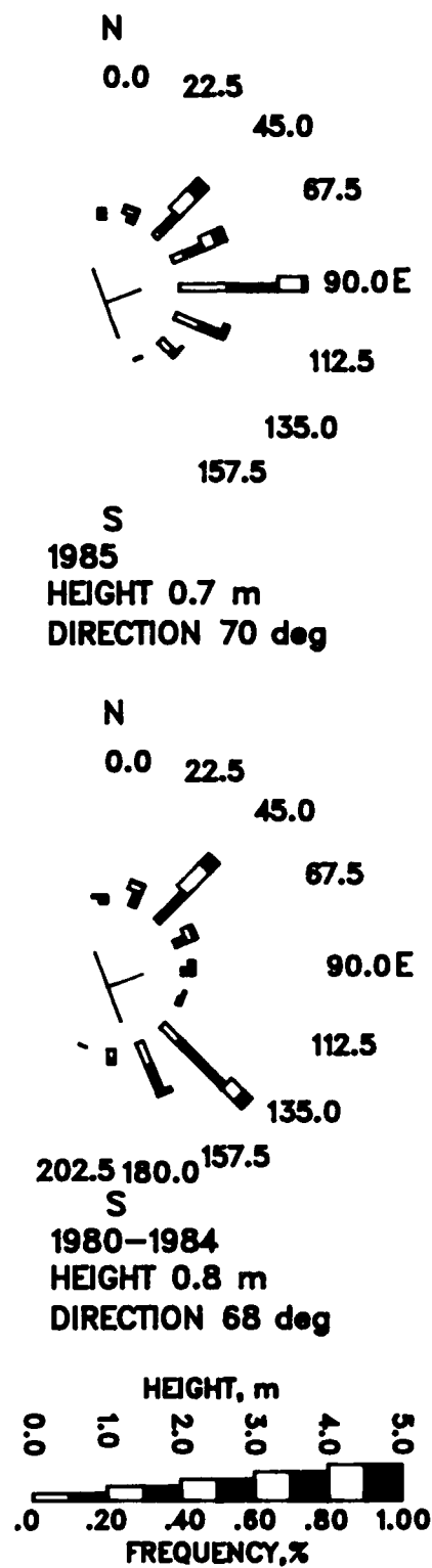
Figure 17. Comparison of annual wave roses, 1985 versus 1980-1984
