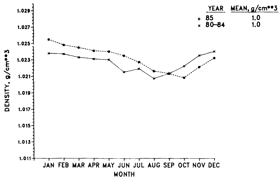
Figure 42. Comparison of mean sea surface water density
