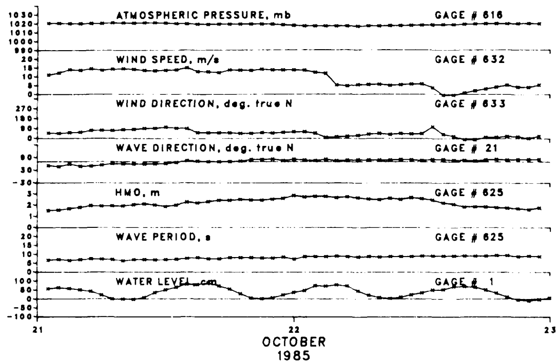
Figure B9. Storm data for 21-22 October 1985
