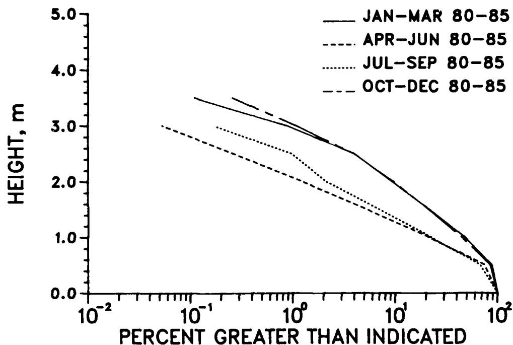
Figure 23. Seasonal wave height distribution for Gage 625, 1980-1985
