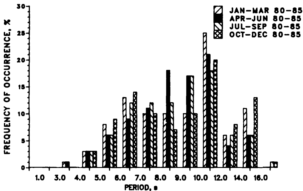
Figure 24. Seasonal wave period distributions for Gage 625, 1980-1985
