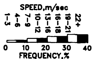
Figure 7. Seasonal wind roses, 1985
