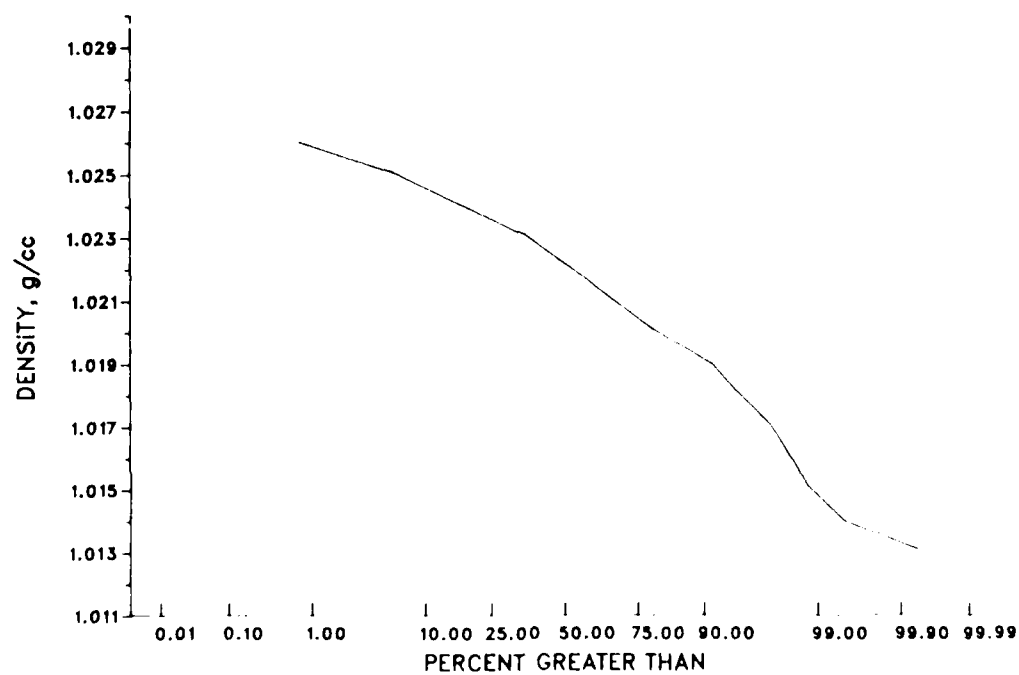
Figure 43. Distribution of surface water density, 1981-1985
