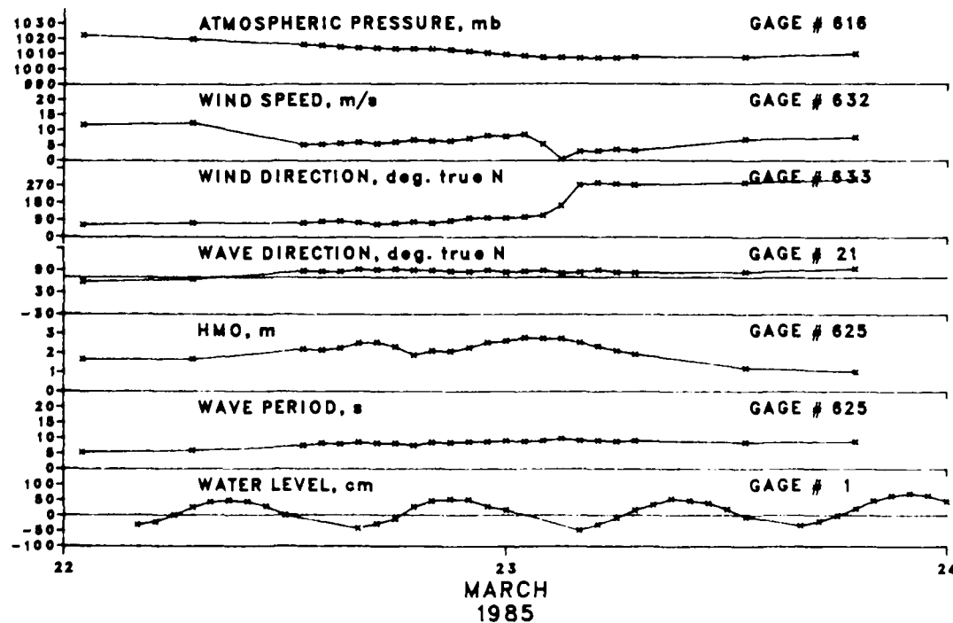
Figure B3. Storm data for 22-23 March 1985
