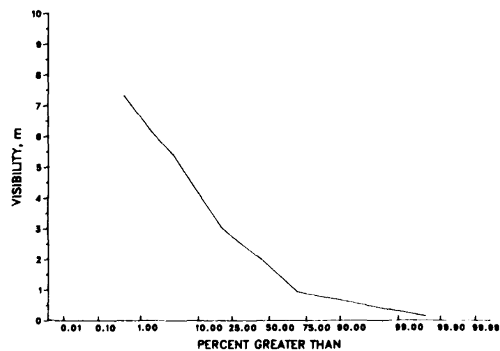
Figure 40. Distribution of surface water visibility, 1980-1985
