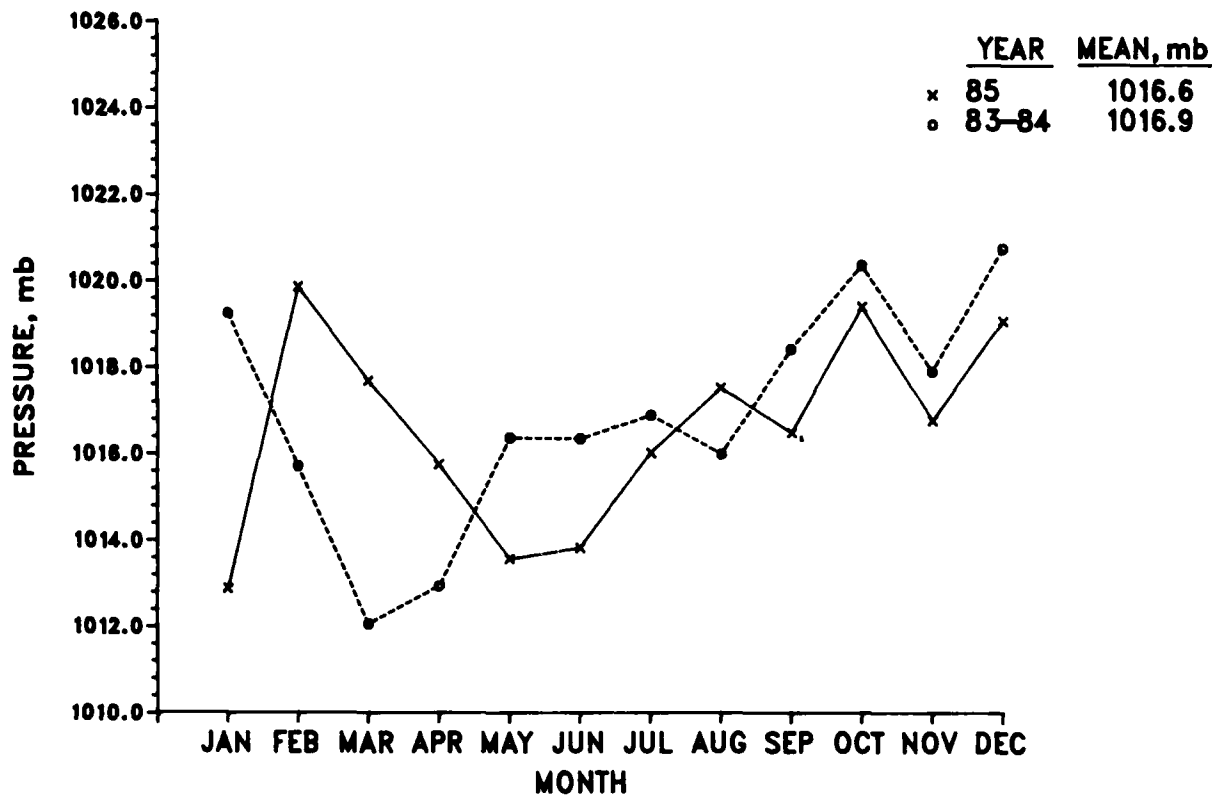
Figure 4. Mean monthly atmospheric pressure
