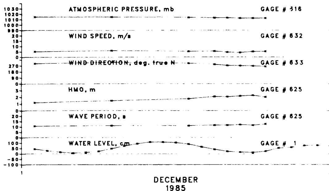
Figure B12. Storm data for 1 December 1985
