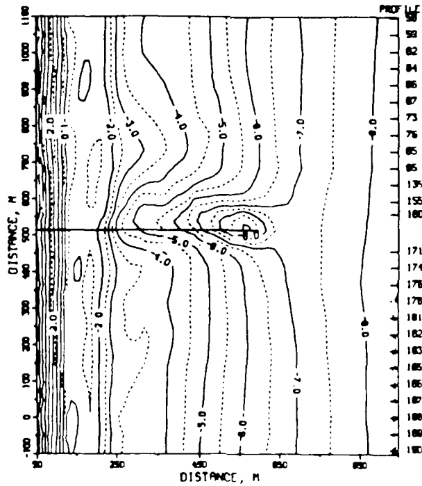
Figure A8. 28 September bathymetry
