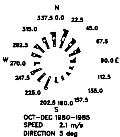
Figure 8. Annual and seasonal wind roses for 1980-1985
