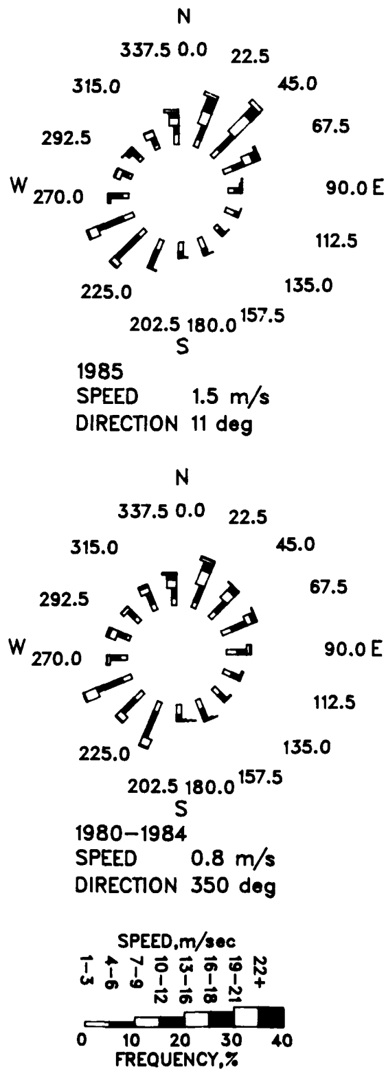
Figure 6. Comparison of annual wind roses, 1985 versus 1980-1984
