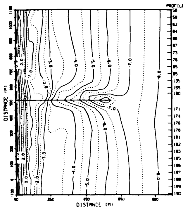
Figure A6. 21 August bathymetry
