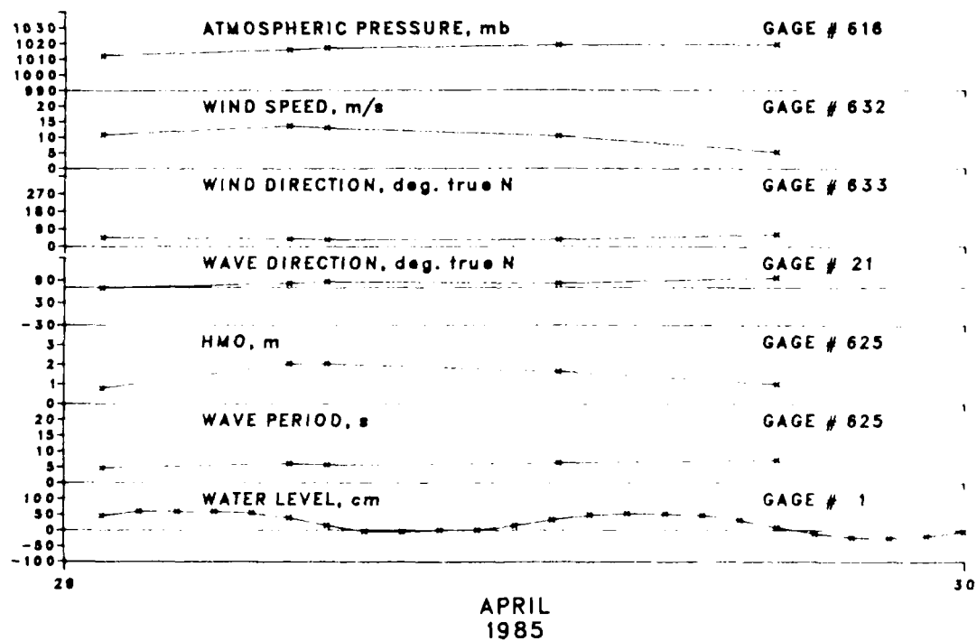
Figure B5. Storm data for 29 April 1985
