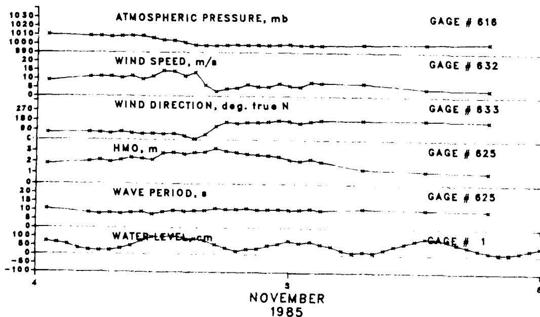
Figure B11. Storm data for 4-5 November 1985
