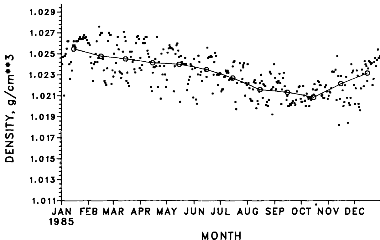
Figure 41. Daily sea surface water density, 1985
