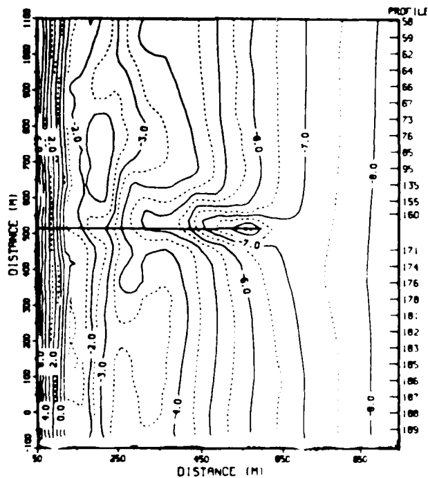
Figure A2. 23 April bathymetry
