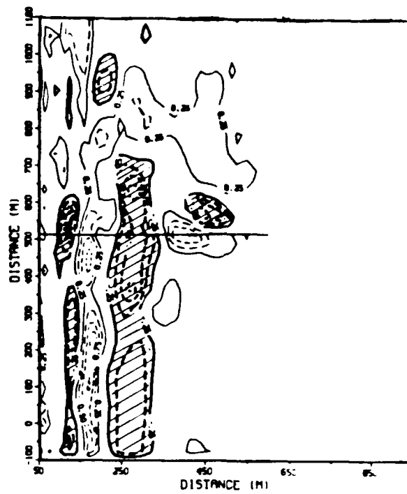
Figure A3. 14 February to 23 April change diagram
