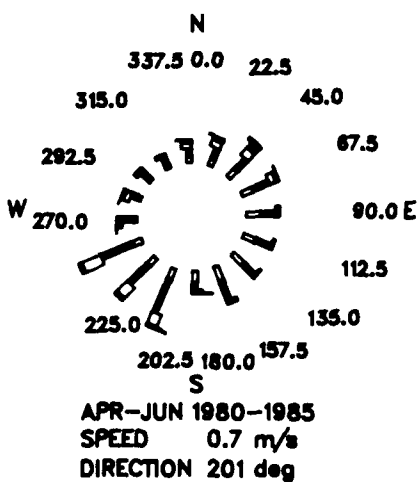
Figure 8. Annual and seasonal wind roses for 1980-1985
