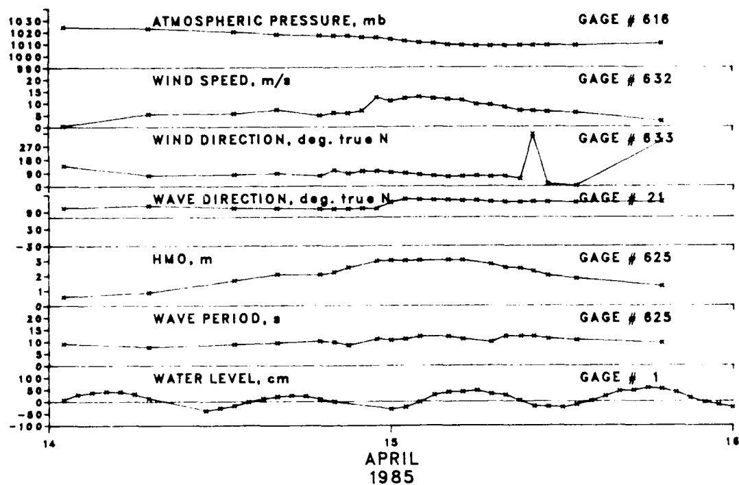
Figure B4. Storm data for 14-15 April 1985
