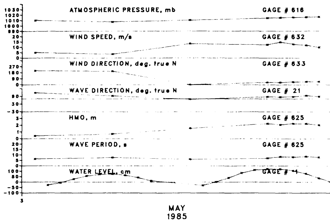
Figure B6. Storm data for 3 May 1985
