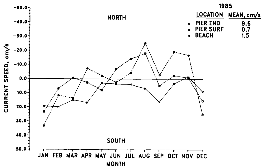
Figure 27. Monthly mean currents, 1985
