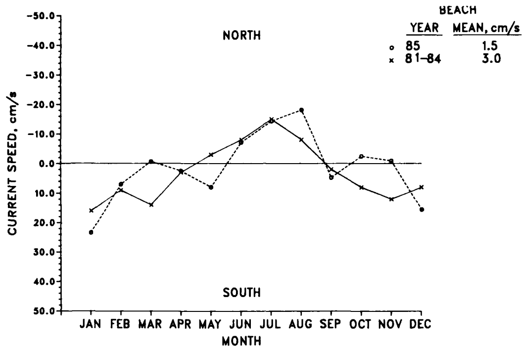
Figure 30. Comparison of surface currents at the beach
