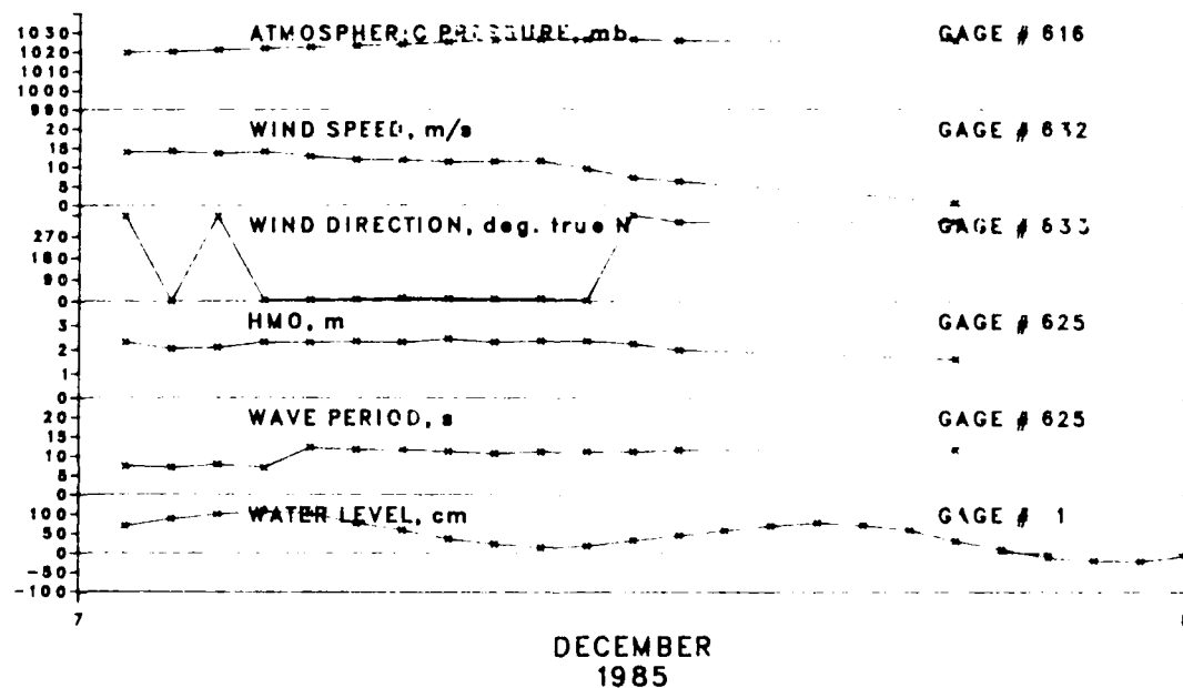
Figure B13. Storm data for 7 December 1985
