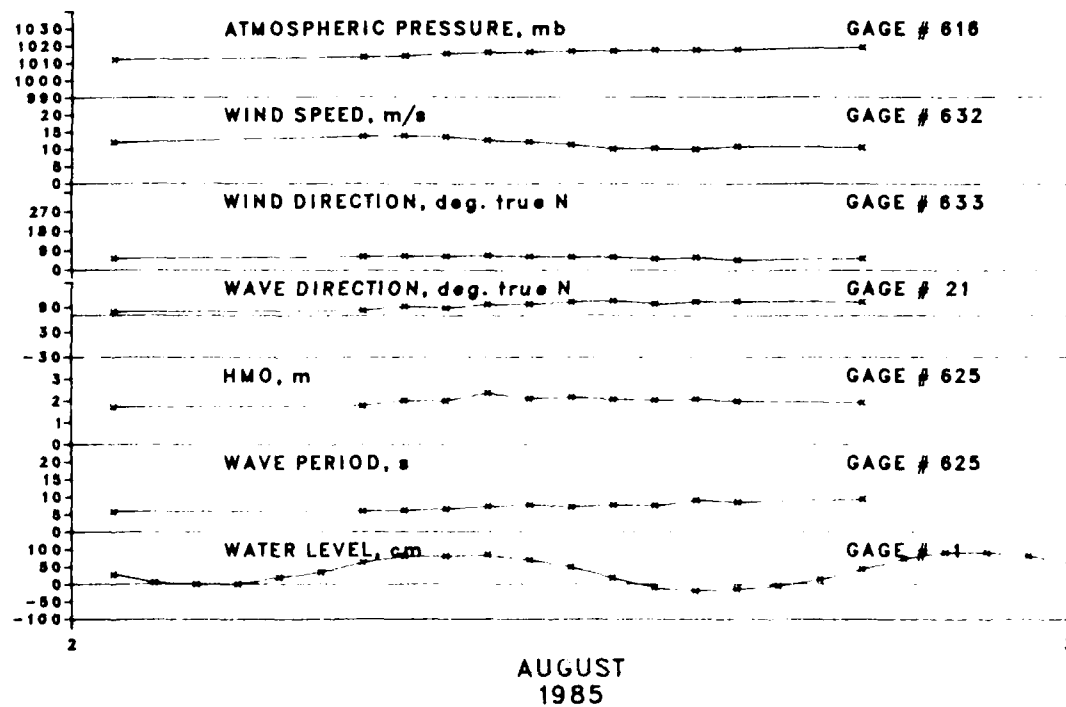
Figure B7. Storm data for 2 August 1985
