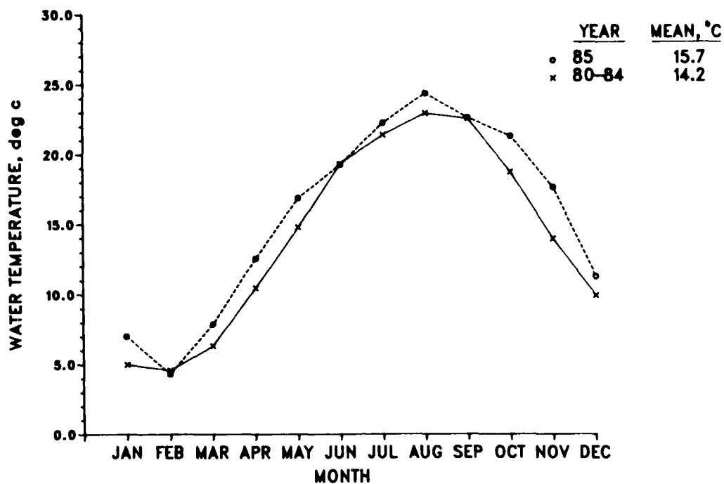
Figure 36. Comparison of mean surface water temperatures
