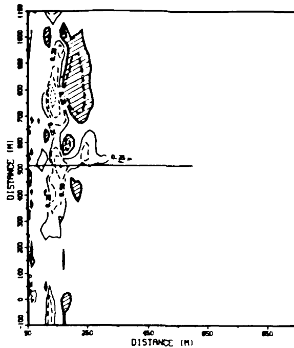
Figure A7. 15 July to 21 August change diagram
