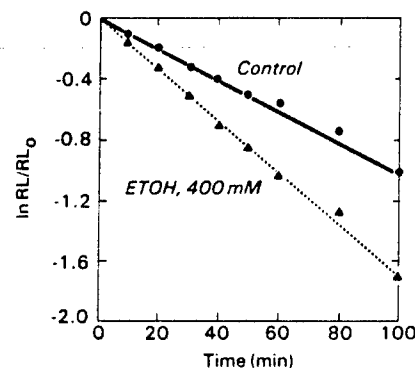
Fig. 5. Effect of ethanol on the dissociation of the [^3\text{H}]\text{BTX-B} /receptor complex. Duplicate samples of forebrain synaptosomes were incubated with 10 nM [^3\text{H}]\text{BTX-B} (scorpion venom concentration was 150 \mu\text{g}/\text{ml} ) for 30 min. At zero time, veratridine (300 \mu\text{M} ) in the absence or presence of ethanol (400 mM) was added and at the indicated times, samples were filtered and binding was measured as described under "Methods." Values are the means from four separate experiments. The standard errors ranged from 4 to 10% of the mean.
