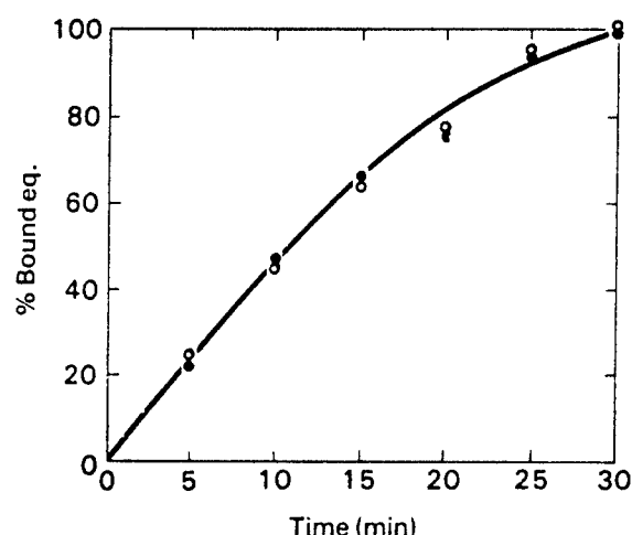
Fig. 4. Time course of formation of the [^3\text{H}]\text{BTX-B} receptor complex. Synaptosomes were incubated for the indicated times with 10 nM [^3\text{H}]\text{BTX-B} (scorpion venom concentration was 150 \mu\text{g}/\text{ml} ) in the absence ( \circ ) and presence ( \bullet ) of 200 mM ethanol. At each time point, binding was measured as described under "Methods." Values are the means from three experiments. The data are expressed as the percentage of specifically bound [^3\text{H}]\text{BTX-B} at equilibrium (eq) (30 min).
