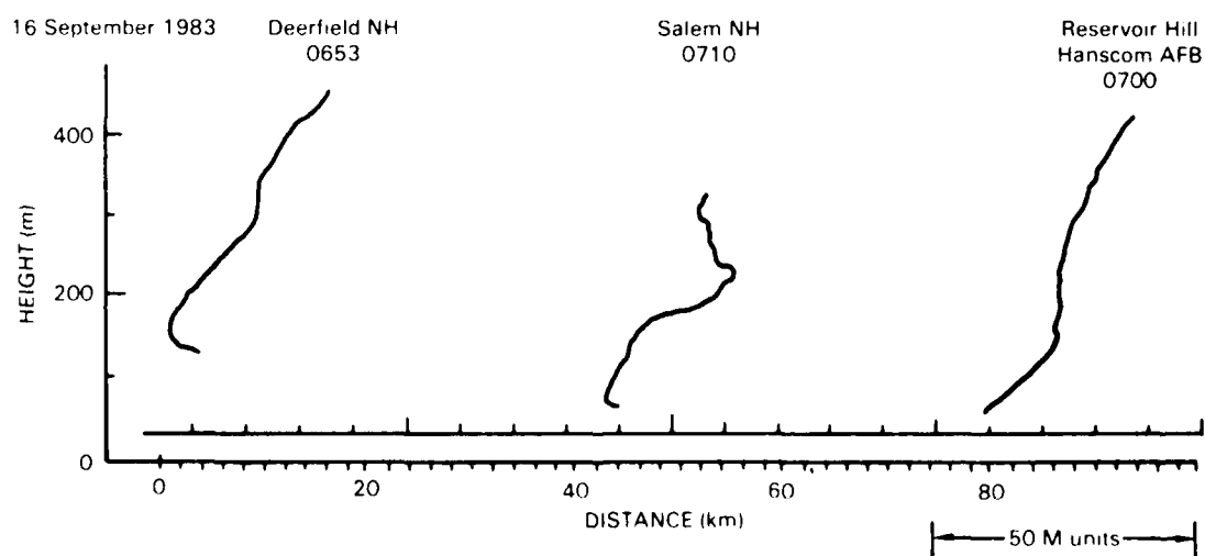
Figure 7. M-unit versus height profiles, 16 September, 1985, for stations of Deerfield, Salem and Hanscom AFB, NH.
