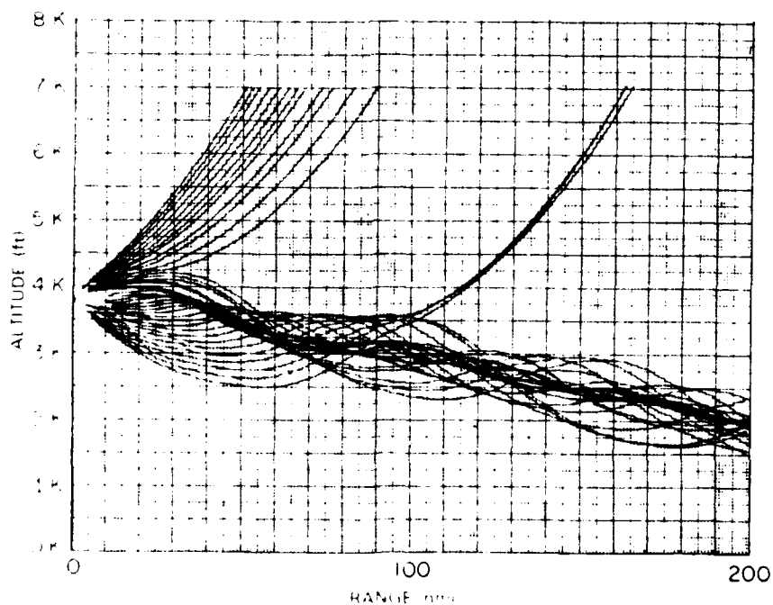
Figure 15 Family of ray paths calculated for a 500 ft thick interface with a slope of 1.89 \times 10^{-3} , a gradient in the interface of 0.1 N-units per ft, and a gradient above and below the interface of 0.01 N-units per ft.
