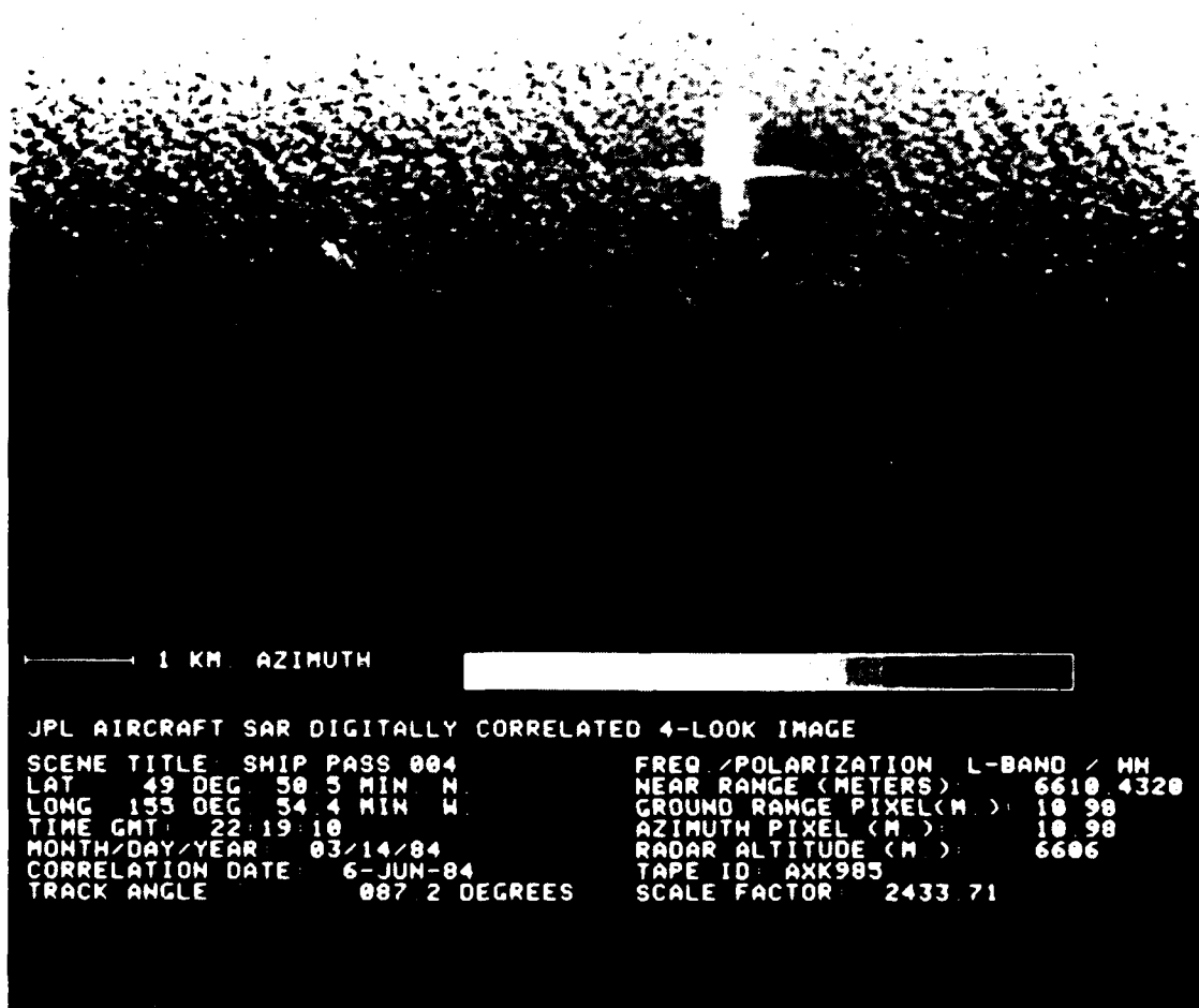
Figure 22. SAR Image of Unidentified Ship on 14 March 1984 in Sea State 3. Ship is Traveling in Same Direction as Aircraft and is Located in SAR Image at 46^{\circ} Incidence Angle.
