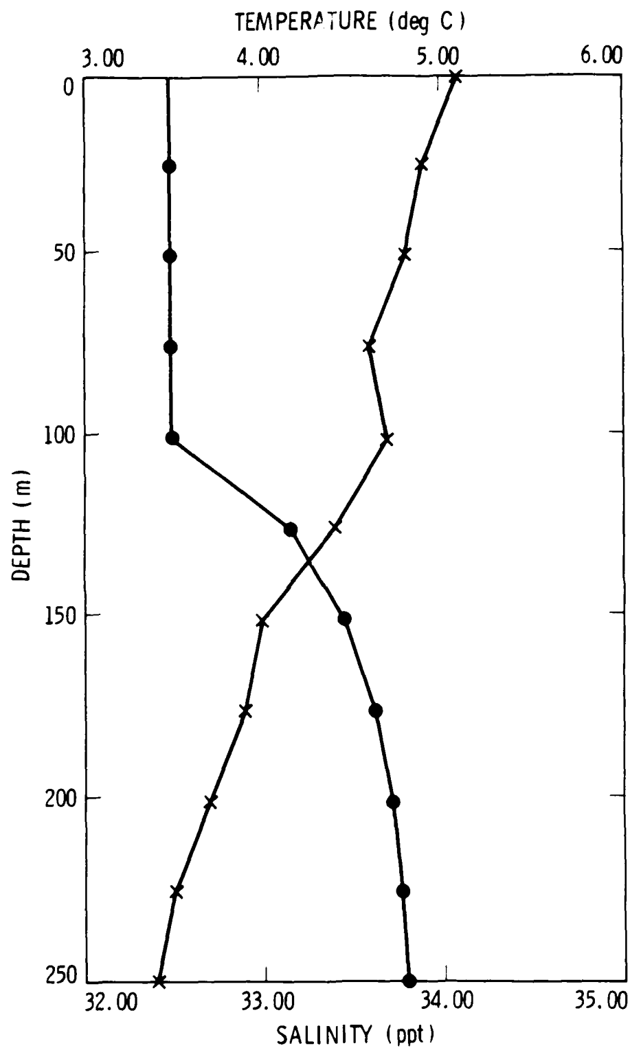
Figure 11. Temperature Profile From Drop No. 15 and Salinity Profile Obtained From Model Fit to Historical Data at Station 36^{\circ} 17' \text{ N} , 143^{\circ} 42' \text{ W} .
