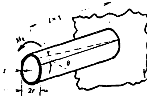
Figure 2.3. Scheme of structures loaded in torsion
