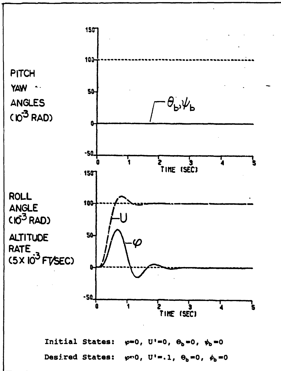
Figure 3.11 (b) Nonlinear System Tracker Response Altitude Rate Command, U'
