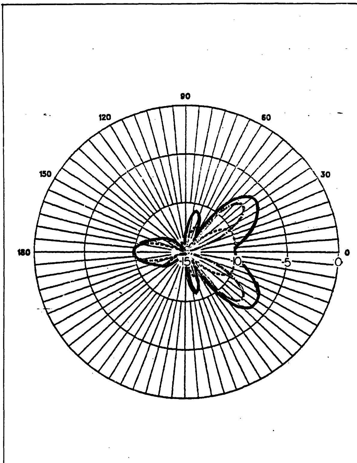
Figure 4.12 (c) Vertical Far Field ( \varphi=45^\circ ) One Loop - One Feed
