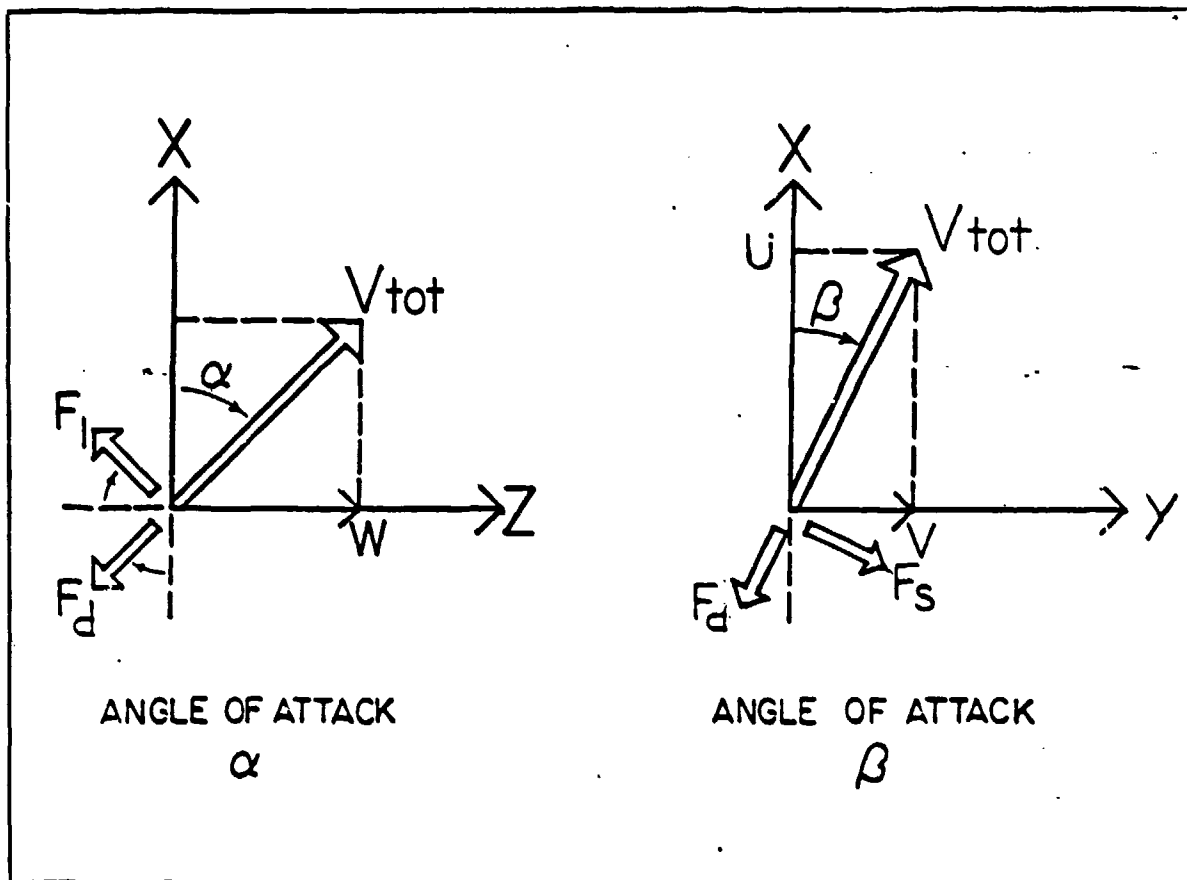
Figure 2.5 Angle of Attack Illustration
