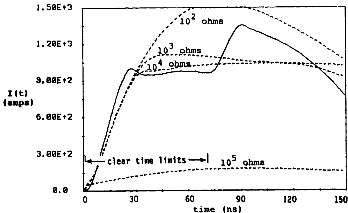
Figure 70. Comparison of Measured (—) and Kudyan/Shih Model (---) Results: E_C = 5 MV/m; R_1, R_2 as Indicated; C_1, C_2 = 5 \times 10^{-11} F
