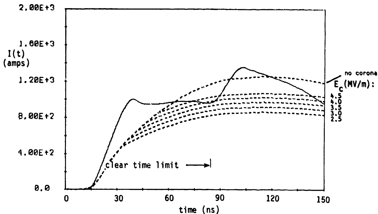
Figure 19. Comparison of Measured (—) and Baum Corona Model (---) Results;
