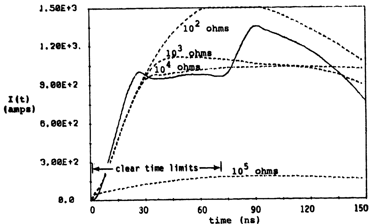
Figure 69. Comparison of Measured (—) and Kudyan/Shih Model (---) Results: E_C = 5 MV/m; R_1, R_2 as Indicated; C_1, C_2 = 10^{-10} F
