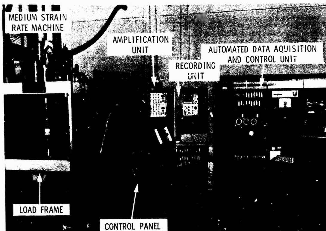
Figure 5 — Automated Materials Characterization Facility
