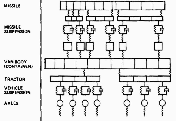
Figure 4 — Analysis Model
