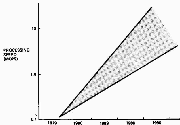
Figure 10 — Projected Microprocessor Speeds
