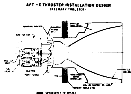
Figure 4. Non-Scarf Primary Engine
