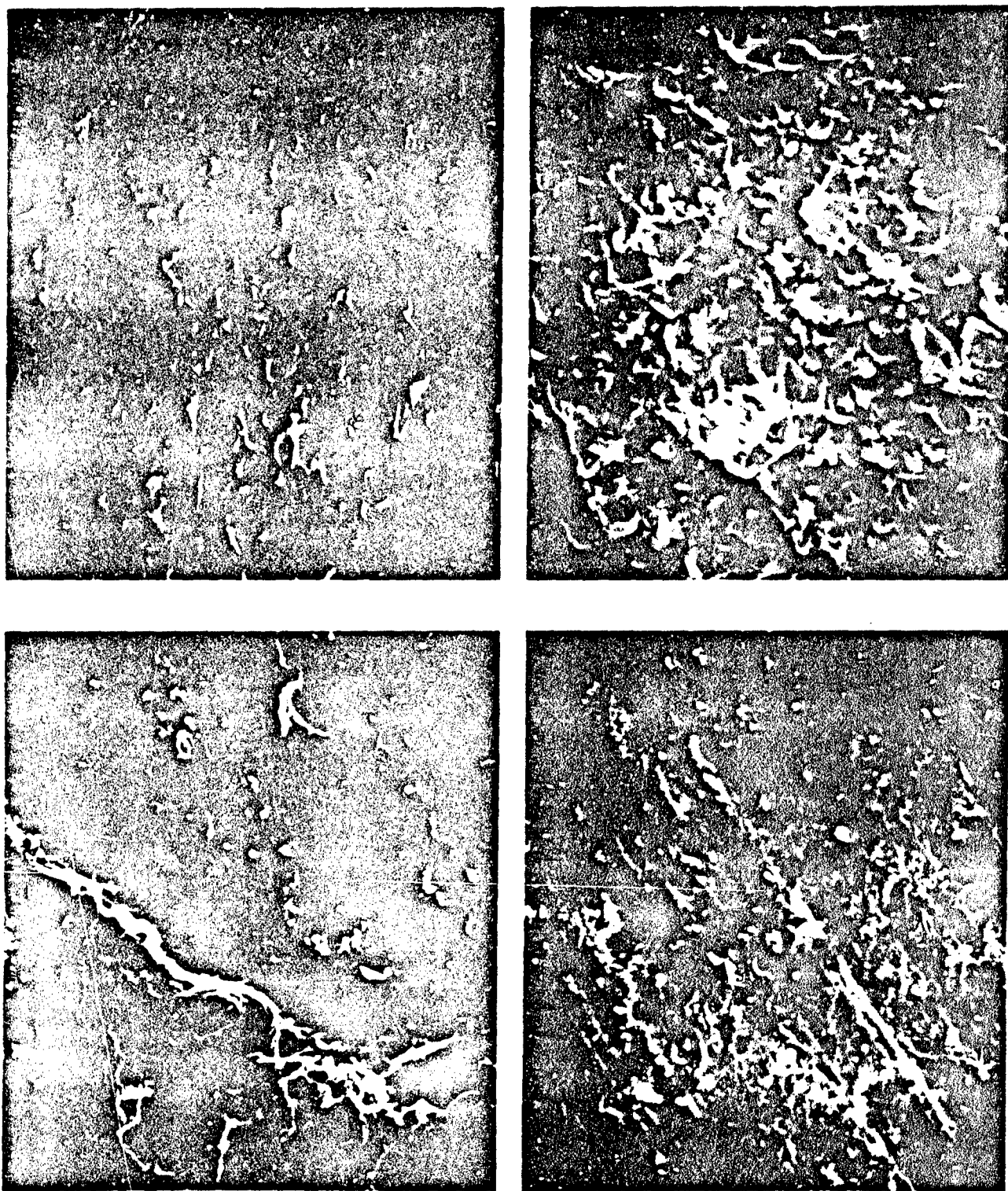
Figure 10. SEM photographs of the TiB 2 coating taken progressively closer to the cutting edge of drill B (Mag. 1U00X).
