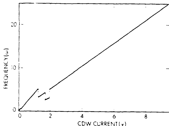
FIG. 2. Frequency vs velocity for the Frenkel-Kontorova model. The segments satisfy v/\omega = (H/2\pi)^n where n=2 for the largest segment and cascades through n=1, 2, 3, 4 as the velocity is decreased further.
