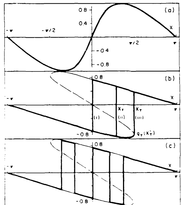
FIG. 1. Stationary states g(x) : (a) P=0.5 , (b) P=3 , ground states for t=0 , (ii) 0 < t < t_p , (iii) t = t_p , v \rightarrow v_T , (iii) t = t_p , v \rightarrow v_T , (iv) t = t_p , v \rightarrow v_T , (iv) t = t_p , v \rightarrow v_T , (v) t = t_p , v \rightarrow v_T , (v) t = t_p , v \rightarrow v_T , (vi) t = t_p , v \rightarrow v_T , (vi) t = t_p , v \rightarrow v_T , (vii) t = t_p , v \rightarrow v_T , (vii) t = t_p , v \rightarrow v_T , (viii) t = t_p , v \rightarrow v_T , (viii) t = t_p , v \rightarrow v_T , (ix) t = t_p , v \rightarrow v_T , (ix) t = t_p , v \rightarrow v_T , (x) t = t_p , v \rightarrow v_T , (x) t = t_p , v \rightarrow v_T , (xi) t = t_p , v \rightarrow v_T , (xi) t = t_p , v \rightarrow v_T , (xii) t = t_p , v \rightarrow v_T , (xii) t = t_p , v \rightarrow v_T , (xiii) t = t_p , v \rightarrow v_T , (xiii) t = t_p , v \rightarrow v_T , (xiv) t = t_p , v \rightarrow v_T , (xiv) t = t_p , v \rightarrow v_T , (xv) t = t_p , v \rightarrow v_T , (xv) t = t_p , v \rightarrow v_T , (xvi) t = t_p , v \rightarrow v_T , (xvi) t = t_p , v \rightarrow v_T , (xvii) t = t_p , v \rightarrow v_T , (xvii) t = t_p , v \rightarrow v_T , (xviii) t = t_p , v \rightarrow v_T , (xviii) t = t_p , v \rightarrow v_T , (xix) t = t_p , v \rightarrow v_T , (xix) t = t_p , v \rightarrow v_T , (xx) t = t_p , v \rightarrow v_T , (xx) t = t_p , v \rightarrow v_T , (xxi) t = t_p , v \rightarrow v_T , (xxi) t = t_p , v \rightarrow v_T , (xxii) t = t_p , v \rightarrow v_T , (xxii) t = t_p , v \rightarrow v_T , (xxiii) t = t_p , v \rightarrow v_T , (xxiii) t = t_p , v \rightarrow v_T , (xxiv) t = t_p , v \rightarrow v_T , (xxiv) t = t_p , v \rightarrow v_T , (xxv) t = t_p , v \rightarrow v_T , (xxv) t = t_p , v \rightarrow v_T , (xxvi) t = t_p , v \rightarrow v_T , (xxvi) t = t_p , v \rightarrow v_T , (xxvii) t = t_p , v \rightarrow v_T , (xxvii) t = t_p , v \rightarrow v_T , (xxviii) t = t_p , v \rightarrow v_T , (xxviii) t = t_p , v \rightarrow v_T , (xxix) t = t_p , v \rightarrow v_T , (xxix) t = t_p , v \rightarrow v_T , (xxx) t = t_p , v \rightarrow v_T , (xxx) t = t_p , v \rightarrow v_T , (xxxi) t = t_p , v \rightarrow v_T , (xxxi) t = t_p , v \rightarrow v_T , (xxxx) t = t_p , v \rightarrow v_T , (xxxx) t = t_p , v \rightarrow v_T , (xxxxi) t = t_p , v \rightarrow v_T , (xxxxi) t = t_p , v \rightarrow v_T , (xxxxii) t = t_p , v \rightarrow v_T , (xxxxii) t = t_p , v \rightarrow v_T , (xxxxiii) t = t_p , v \rightarrow v_T , (xxxxiii) t = t_p , v \rightarrow v_T , (xxxxiv) t = t_p , v \rightarrow v_T , (xxxxiv) t = t_p , v \rightarrow v_T , (xxxxv) t = t_p , v \rightarrow v_T , (xxxxv) t = t_p , v \rightarrow v_T , (xxxxvi) t = t_p , v \rightarrow v_T , (xxxxvi) t = t_p , v \rightarrow v_T , (xxxxvii) t = t_p , v \rightarrow v_T , (xxxxvii) t = t_p , v \rightarrow v_T , (xxxxviii) t = t_p , v \rightarrow v_T , (xxxxviii) t = t_p , v \rightarrow v_T , (xxxxix) t = t_p , v \rightarrow v_T , (xxxxix) t = t_p , v \rightarrow v_T , (xxxxx) t = t_p , v \rightarrow v_T , (xxxxx) t = t_p , v \rightarrow v_T , (xxxxxi) t = t_p , v \rightarrow v_T , (xxxxxi) t = t_p , v \rightarrow v_T , (xxxxxii) t = t_p , v \rightarrow v_T , (xxxxxii) t = t_p , v \rightarrow v_T , (xxxxxiii) t = t_p , v \rightarrow v_T , (xxxxxiii) t = t_p , v \rightarrow v_T , (xxxxxiv) t = t_p , v \rightarrow v_T , (xxxxxiv) t = t_p , v \rightarrow v_T , (xxxxxv) t = t_p , v \rightarrow v_T , (xxxxxv) t = t_p , v \rightarrow v_T , (xxxxxvi) t = t_p , v \rightarrow v_T , (xxxxxvi) t = t_p , v \rightarrow v_T , (xxxxxvii) t = t_p , v \rightarrow v_T , (xxxxxvii) t = t_p , v \rightarrow v_T , (xxxxxviii) t = t_p , v \rightarrow v_T , (xxxxxviii) t = t_p , v \rightarrow v_T , (xxxxxix) t = t_p , v \rightarrow v_T , (xxxxxix) t = t_p , v \rightarrow v_T , (xxxxxx) t = t_p , v \rightarrow v_T , (xxxxxx) t = t_p , v \rightarrow v_T , (xxxxxxi) t = t_p , v \rightarrow v_T , (xxxxxxi) t = t_p , v \rightarrow v_T , (xxxxxxii) t = t_p , v \rightarrow v_T , (xxxxxxii) t = t_p , v \rightarrow v_T , (xxxxxxiii) t = t_p , v \rightarrow v_T , (xxxxxxiii) t = t_p , v \rightarrow v_T , (xxxxxxiv) t = t_p , v \rightarrow v_T , (xxxxxxiv) t = t_p , v \rightarrow v_T , (xxxxxxv) t = t_p , v \rightarrow v_T , (xxxxxxv) t = t_p , v \rightarrow v_T , (xxxxxxvi) t = t_p , v \rightarrow v_T , (xxxxxxvi) t = t_p , v \rightarrow v_T , (xxxxxxvii) t = t_p , v \rightarrow v_T , (xxxxxxvii) t = t_p , v \rightarrow v_T , (xxxxxxviii) t = t_p , v \rightarrow v_T , (xxxxxxviii) t = t_p , v \rightarrow v_T , (xxxxxxix) t = t_p , v \rightarrow v_T , (xxxxxxix) t = t_p , v \rightarrow v_T , (xxxxxxx) t = t_p , v \rightarrow v_T , (xxxxxxx) t = t_p , v \rightarrow v_T , (xxxxxxxi) t = t_p , v \rightarrow v_T , (xxxxxxxi) t = t_p , v \rightarrow v_T , (xxxxxxxii) t = t_p , v \rightarrow v_T , (xxxxxxxii) t = t_p , v \rightarrow v_T , (xxxxxxxiii) t = t_p , v \rightarrow v_T , (xxxxxxxiii) t = t_p , v \rightarrow v_T , (xxxxxxxiv) t = t_p , v \rightarrow v_T , (xxxxxxxiv) t = t_p , v \rightarrow v_T , (xxxxxxxv) t = t_p , v \rightarrow v_T , (xxxxxxxv) t = t_p , v \rightarrow v_T , (xxxxxxxvi) t = t_p , v \rightarrow v_T , (xxxxxxxvi) t = t_p , v \rightarrow v_T , (xxxxxxxvii) t = t_p , v \rightarrow v_T , (xxxxxxxvii) t = t_p , v \rightarrow v_T , (xxxxxxxviii) t = t_p , v \rightarrow v_T , (xxxxxxxviii) t = t_p , v \rightarrow v_T , (xxxxxxxix) t = t_p , v \rightarrow v_T , (xxxxxxxix) t = t_p , v \rightarrow v_T , (xxxxxxx) t = t_p , v \rightarrow v_T , (xxxxxxx) t = t_p , v \rightarrow v_T , (xxxxxxxi) t = t_p , v \rightarrow v_T , (xxxxxxxi) t = t_p , v \rightarrow v_T , (xxxxxxxii) t = t_p , v \rightarrow v_T , (xxxxxxxii) t = t_p , v \rightarrow v_T , (xxxxxxxiii) t = t_p , v \rightarrow v_T , (xxxxxxxiii) t = t_p , v \rightarrow v_T , (xxxxxxxiv) t = t_p , v \rightarrow v_T , (xxxxxxxiv) t = t_p , v \rightarrow v_T , (xxxxxxxv) t = t_p , v \rightarrow v_T , (xxxxxxxv) t = t_p , v \rightarrow v_T , (xxxxxxxvi) t = t_p , v \rightarrow v_T , (xxxxxxxvi) t = t_p , v \rightarrow v_T , (xxxxxxxvii) t = t_p , v \rightarrow v_T , (xxxxxxxvii) t = t_p , v \rightarrow v_T , (xxxxxxxviii) t = t_p , v \rightarrow v_T , (xxxxxxxviii) t = t_p , v \rightarrow v_T , (xxxxxxxix) t = t_p , v \rightarrow v_T , (xxxxxxxix) t = t_p , v \rightarrow v_T , (xxxxxxx) t = t_p , v \rightarrow v_T , (xxxxxxx) t = t_p , v \rightarrow v_T , (xxxxxxxi) t = t_p , v \rightarrow v_T , (xxxxxxxi) t = t_p , v \rightarrow v_T , (xxxxxxxii) t = t_p , v \rightarrow v_T , (xxxxxxxii) t = t_p , v \rightarrow v_T , (xxxxxxxiii) t = t_p , v \rightarrow v_T , (xxxxxxxiii) t = t_p , v \rightarrow v_T , (xxxxxxxiv) t = t_p , v \rightarrow v_T , (xxxxxxxiv) t = t_p , v \rightarrow v_T , (xxxxxxxv) t = t_p , v \rightarrow v_T , (xxxxxxxv) t = t_p , v \rightarrow v_T , (xxxxxxxvi) t = t_p , v \rightarrow v_T , (xxxxxxxvi) t = t_p , v \rightarrow v_T , (xxxxxxxvii) t = t_p , v \rightarrow v_T , (xxxxxxxvii) t = t_p , v \rightarrow v_T , (xxxxxxxviii) t = t_p , v \rightarrow v_T , (xxxxxxxviii) t = t_p , v \rightarrow v_T , (xxxxxxxix) t = t_p , v \rightarrow v_T , (xxxxxxxix) t = t_p , v \rightarrow v_T , (xxxxxxx) t = t_p , v \rightarrow v_T , (xxxxxxx) t = t_p , v \rightarrow v_T , (xxxxxxxi) t = t_p , v \rightarrow v_T , (xxxxxxxi) t = t_p , v \rightarrow v_T , (xxxxxxxii) t = t_p , v \rightarrow v_T , (xxxxxxxii) t = t_p , v \rightarrow v_T , (xxxxxxxiii) t = t_p , v \rightarrow v_T , (xxxxxxxiii) t = t_p , v \rightarrow v_T , (xxxxxxxiv) t = t_p , v \rightarrow v_T , (xxxxxxxiv) t = t_p , v \rightarrow v_T , (xxxxxxxv) t = t_p , v \rightarrow v_T , (xxxxxxxv) t = t_p , v \rightarrow v_T , (xxxxxxxvi) t = t_p , v \rightarrow v_T , (xxxxxxxvi) t = t_p , v \rightarrow v_T , (xxxxxxxvii) t = t_p , v \rightarrow v_T , (xxxxxxxvii) t = t_p , v \rightarrow v_T , (xxxxxxxviii) t = t_p , v \rightarrow v_T , (xxxxxxxviii) t = t_p , v \rightarrow v_T , (xxxxxxxix) t = t_p , v \rightarrow v_T , (xxxxxxxix) t = t_p , v \rightarrow v_T , (xxxxxxx) t = t_p , v \rightarrow v_T , (xxxxxxx) t = t_p , v \rightarrow v_T , (xxxxxxxi) t = t_p , v \rightarrow v_T , (xxxxxxxi) t = t_p , v \rightarrow v_T , (xxxxxxxii) t = t_p , v \rightarrow v_T , (xxxxxxxii) t = t_p , v \rightarrow v_T , (xxxxxxxiii) t = t_p , v \rightarrow v_T , (xxxxxxxiii) t = t_p , v \rightarrow v_T , (xxxxxxxiv) t = t_p , v \rightarrow v_T , (xxxxxxxiv) t = t_p , v \rightarrow v_T , (xxxxxxxv) t = t_p , v \rightarrow v_T , (xxxxxxxv) t = t_p , v \rightarrow v_T , (xxxxxxxvi) t = t_p , v \rightarrow v_T , (xxxxxxxvi) t = t_p , v \rightarrow v_T , (xxxxxxxvii) t = t_p , v \rightarrow v_T , (xxxxxxxvii) t = t_p , v \rightarrow v_T , (xxxxxxxviii) t = t_p , v \rightarrow v_T , (xxxxxxxviii) t = t_p , v \rightarrow v_T , (xxxxxxxix) t = t_p , v \rightarrow v_T , (xxxxxxxix) t = t_p , v \rightarrow v_T , (xxxxxxx) t = t_p , v \rightarrow v_T , (xxxxxxx) t = t_p , v \rightarrow v_T , (xxxxxxxi) t = t_p , v \rightarrow v_T , (xxxxxxxi) t = t_p , v \rightarrow v_T , (xxxxxxxii) t = t_p , v \rightarrow v_T , (xxxxxxxii) t = t_p , v \rightarrow v_T , (xxxxxxxiii) t = t_p , v \rightarrow v_T , (xxxxxxxiii) t = t_p , v \rightarrow v_T , (xxxxxxxiv) t = t_p , v \rightarrow v_T , (xxxxxxxiv) t = t_p , v \rightarrow v_T , (xxxxxxxv) t = t_p , v \rightarrow v_T , (xxxxxxxv) t = t_p , v \rightarrow v_T , (xxxxxxxvi) t = t_p , v \rightarrow v_T , (xxxxxxxvi) t = t_p , v \rightarrow v_T , (xxxxxxxvii) t = t_p , v \rightarrow v_T , (xxxxxxxvii) t = t_p , v \rightarrow v_T , (xxxxxxxviii) t = t_p , v \rightarrow v_T , (xxxxxxxviii) t = t_p , v \rightarrow v_T , (xxxxxxxix) t = t_p , v \rightarrow v_T , (xxxxxxxix) t = t_p , v \rightarrow v_T , (xxxxxxx) t = t_p , v \rightarrow v_T , (xxxxxxx) t = t_p , v \rightarrow v_T , (xxxxxxxi) t = t_p , v \rightarrow v_T , (xxxxxxxi) t = t_p , v \rightarrow v_T , (xxxxxxxii) t = t_p , v \rightarrow v_T , (xxxxxxxii) t = t_p , v \rightarrow v_T , (xxxxxxxiii) t = t_p , v \rightarrow v_T , (xxxxxxxiii) t = t_p , v \rightarrow v_T , (xxxxxxxiv) t = t_p , v \rightarrow v_T , (xxxxxxxiv) t = t_p , v \rightarrow v_T , (xxxxxxxv) t = t_p , v \rightarrow v_T , (xxxxxxxv) t = t_p , v \rightarrow v_T , (xxxxxxxvi) t = t_p , v \rightarrow v_T , (xxxxxxxvi) t = t_p , v \rightarrow v_T , (xxxxxxxvii) t = t_p , v \rightarrow v_T , (xxxxxxxvii) t = t_p , v \rightarrow v_T , (xxxxxxxviii) t = t_p , v \rightarrow v_T , (xxxxxxxviii) t = t_p , v \rightarrow v_T , (xxxxxxxix) t = t_p , v \rightarrow v_T , (xxxxxxxix) t = t_p , v \rightarrow v_T , (xxxxxxx) t = t_p , v \rightarrow v_T , (xxxxxxx) t = t_p , v \rightarrow v_T , (xxxxxxxi) t = t_p , v \rightarrow v_T , (xxxxxxxi) t = t_p , v \rightarrow v_T , (xxxxxxxii) t = t_p , v \rightarrow v_T , (xxxxxxxii) t = t_p , v \rightarrow v_T , (xxxxxxxiii) t = t_p , v \rightarrow v_T , (xxxxxxxiii) t = t_p , v \rightarrow v_T , (xxxxxxxiv) t = t_p , v \rightarrow v_T , (xxxxxxxiv) t = t_p , v \rightarrow v_T , (xxxxxxxv) t = t_p , v \rightarrow v_T , (xxxxxxxv) t = t_p , v \rightarrow v_T , (xxxxxxxvi) t = t_p , v \rightarrow v_T , (xxxxxxxvi) t = t_p , v \rightarrow v_T , (xxxxxxxvii) t = t_p , v \rightarrow v_T , (xxxxxxxvii) t = t_p , v \rightarrow v_T , (xxxxxxxviii) t = t_p , v \rightarrow v_T , (xxxxxxxviii) t = t_p , v \rightarrow v_T , (xxxxxxxix) t = t_p , v \rightarrow v_T , (xxxxxxxix) t = t_p , v \rightarrow v_T , (xxxxxxx) t = t_p , v \rightarrow v_T , (xxxxxxx) t = t_p , v \rightarrow v_T , (xxxxxxxi) t = t_p , v \rightarrow v_T , (xxxxxxxi) t = t_p , v \rightarrow v_T , (xxxxxxxii) t = t_p , v \rightarrow v_T , (xxxxxxxii) t = t_p , v \rightarrow v_T , (xxxxxxxiii) t = t_p , v \rightarrow v_T , (xxxxxxxiii) t = t_p , v \rightarrow v_T , (xxxxxxxiv) t = t_p , v \rightarrow v_T , (xxxxxxxiv) t = t_p , v \rightarrow v_T , (xxxxxxxv) t = t_p , v \rightarrow v_T , (xxxxxxxv) t = t_p , v \rightarrow v_T , (xxxxxxxvi) t = t_p , v \rightarrow v_T , (xxxxxxxvi) t = t_p , v \rightarrow v_T , (xxxxxxxvii) t = t_p , v \rightarrow v_T , (xxxxxxxvii) t = t_p , v \rightarrow v_T , (xxxxxxxviii) t = t_p , v \rightarrow v_T , (xxxxxxxviii) t = t_p , v \rightarrow v_T , (xxxxxxxix) t = t_p , v \rightarrow v_T , (xxxxxxxix) t = t_p , v \rightarrow v_T , (xxxxxxx) t = t_p , v \rightarrow v_T , (xxxxxxx) t = t_p , v \rightarrow v_T , (xxxxxxxi) t = t_p , v \rightarrow v_T , (xxxxxxxi) t = t_p , v \rightarrow v_T , (xxxxxxxii) t = t_p , v \rightarrow v_T , (xxxxxxxii) t = t_p , v \rightarrow v_T , (xxxxxxxiii) t = t_p , v \rightarrow v_T , (xxxxxxxiii) t = t_p , v \rightarrow v_T , (xxxxxxxiv) t = t_p , v \rightarrow v_T , (xxxxxxxiv) t = t_p , v \rightarrow v_T , (xxxxxxxv) t = t_p , v \rightarrow v_T , (xxxxxxxv) t = t_p , v \rightarrow v_T , (xxxxxxxvi) t = t_p , v \rightarrow v_T , (xxxxxxxvi) t = t_p , v \rightarrow v_T , (xxxxxxxvii) t = t_p , v \rightarrow v_T , (xxxxxxxvii) t = t_p , v \rightarrow v_T , (xxxxxxxviii) t = t_p , v \rightarrow v_T , (xxxxxxxviii) t = t_p , v \rightarrow v_T , (xxxxxxxix) t = t_p , v \rightarrow v_T , (xxxxxxxix) t = t_p , v \rightarrow v_T , (xxxxxxx) t = t_p , v \rightarrow v_T , (xxxxxxx) t = t_p , v \rightarrow v_T , (xxxxxxxi) t = t_p , v \rightarrow v_T , (xxxxxxxi) t = t_p , v \rightarrow v_T , (xxxxxxxii) t = t_p , v \rightarrow v_T , (xxxxxxxii) t = t_p , v \rightarrow v_T , (xxxxxxxiii) t = t_p , v \rightarrow v_T , (xxxxxxxiii) t = t_p , v \rightarrow v_T , (xxxxxxxiv) t = t_p , v \rightarrow v_T , (xxxxxxxiv) t = t_p , v \rightarrow v_T , (xxxxxxxv) t = t_p , v \rightarrow v_T , (xxxxxxxv) t = t_p , v \rightarrow v_T , (xxxxxxxvi) t = t_p , v \rightarrow v_T , (xxxxxxxvi) t = t_p , v \rightarrow v_T , (xxxxxxxvii) t = t_p , v \rightarrow v_T , (xxxxxxxvii) t = t_p , v \rightarrow v_T , (xxxxxxxviii) t = t_p , v \rightarrow v_T , (xxxxxxxviii) t = t_p , v \rightarrow v_T , (xxxxxxxix) t = t_p , v \rightarrow v_T , (xxxxxxxix) t = t_p , v \rightarrow v_T , (xxxxxxx) t = t_p , v \rightarrow v_T , (xxxxxxx) t = t_p , v \rightarrow v_T , (xxxxxxxi) t = t_p , v \rightarrow v_T , (xxxxxxxi) t = t_p , v \rightarrow v_T , (xxxxxxxii) t = t_p , v \rightarrow v_T , (xxxxxxxii) t = t_p , v \rightarrow v_T , (xxxxxxxiii) t = t_p , v \rightarrow v_T , (xxxxxxxiii) t = t_p , v \rightarrow v_T , (xxxxxxxiv) t = t_p , v \rightarrow v_T , (xxxxxxxiv) t = t_p , v \rightarrow v_T , (xxxxxxxv) t = t_p , v \rightarrow v_T , (xxxxxxxv) t = t_p , v \rightarrow v_T , (xxxxxxxvi) t = t_p , v \rightarrow v_T , (xxxxxxxvi) t = t_p , v \rightarrow v_T , (xxxxxxxvii) t = t_p , v \rightarrow v_T , (xxxxxxxvii) t = t_p , v \rightarrow v_T , (xxxxxxxviii) t = t_p , v \rightarrow v_T , (xxxxxxxviii) t = t_p , v \rightarrow v_T , (xxxxxxxix) t = t_p , v \rightarrow v_T , (xxxxxxxix) t = t_p , v \rightarrow v_T , (xxxxxxx) t = t_p , v \rightarrow v_T , (xxxxxxx) t = t_p , v \rightarrow v_T , (xxxxxxxi) t = t_p , v \rightarrow v_T , (xxxxxxxi) t = t_p , v \rightarrow v_T , (xxxxxxxii) t = t_p , v \rightarrow v_T , (xxxxxxxii) t = t_p , v \rightarrow v_T , (xxxxxxxiii) t = t_p , v \rightarrow v_T , (xxxxxxxiii) t = t_p , v \rightarrow v_T , (xxxxxxxiv) t = t_p , v \rightarrow v_T , (xxxxxxxiv) t = t_p , v \rightarrow v_T , (xxxxxxxv) t = t_p , v \rightarrow v_T , (xxxxxxxv) t = t_p , v \rightarrow v_T , (xxxxxxxvi) t = t_p , v \rightarrow v_T , (xxxxxxxvi) t = t_p , v \rightarrow v_T , (xxxxxxxvii) t = t_p , v \rightarrow v_T , (xxxxxxxvii) t = t_p , v \rightarrow v_T , (xxxxxxxviii) t = t_p , v \rightarrow v_T , (xxxxxxxviii) t = t_p , v \rightarrow v_T , (xxxxxxxix) t = t_p , v \rightarrow v_T , (xxxxxxxix) t = t_p , v \rightarrow v_T , (xxxxxxx) t = t_p , v \rightarrow v_T , (xxxxxxx) t = t_p , v \rightarrow v_T , (xxxxxxxi) t = t_p , v \rightarrow v_T , (xxxxxxxi) t = t_p , v \rightarrow v_T , (xxxxxxxii) t = t_p , v \rightarrow v_T , (xxxxxxxii) t = t_p , v \rightarrow v_T , (xxxxxxxiii) t = t_p , v \rightarrow v_T , (xxxxxxxiii) t = t_p , v \rightarrow v_T , (xxxxxxxiv) t = t_p , v \rightarrow v_T , (xxxxxxxiv) t = t_p , v \rightarrow v_T , (xxxxxxxv) t = t_p , v \rightarrow v_T , (xxxxxxxv) t = t_p , v \rightarrow v_T , (xxxxxxxvi) t = t_p , v \rightarrow v_T , (xxxxxxxvi) t = t_p , v \rightarrow v_T , (xxxxxxxvii) t = t_p , v \rightarrow v_T , (xxxxxxxvii) t = t_p , v \rightarrow v_T , (xxxxxxxviii) t = t_p , v \rightarrow v_T , (xxxxxxxviii) t = t_p , v \rightarrow v_T , (xxxxxxxix) t = t_p , v \rightarrow v_T , (xxxxxxxix) t = t_p , v \rightarrow v_T , (xxxxxxx) t = t_p , v \rightarrow v_T , (xxxxxxx) t = t_p , v \rightarrow v_T , (xxxxxxxi) t = t_p , v \rightarrow v_T , (xxxxxxxi) t = t_p , v \rightarrow v_T , (xxxxxxxii) t
