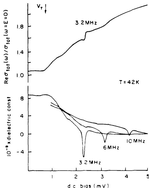
FIG. 2. ac response (Ref. 7) of NbSe 3 .
