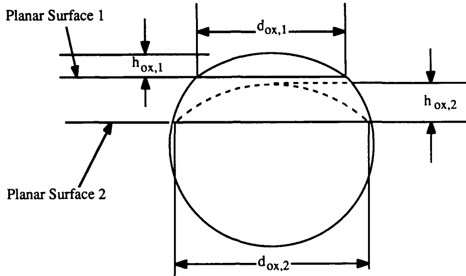
Figure A.21. Nomenclature for Average Nonplanar Oxidizer Surface Area Calculation
