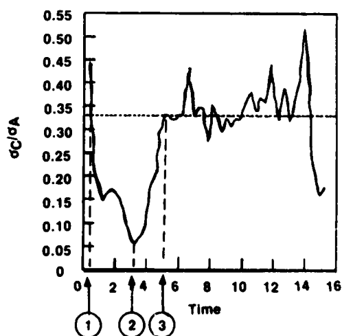
Fig. 4 — Time sequence of silo loading
