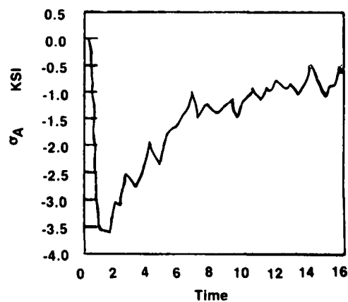
Fig. 4 — Time sequence of silo loading
