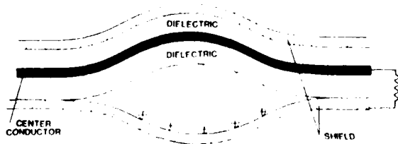
FIGURE 3 TRIBOELECTRIC EFFECT
