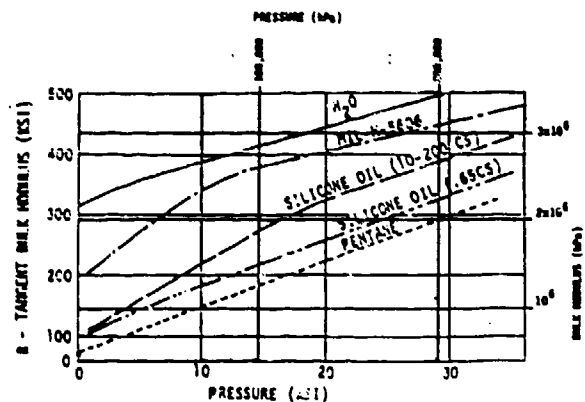
Figure 2. Bulk Modulus for Various Fluids
