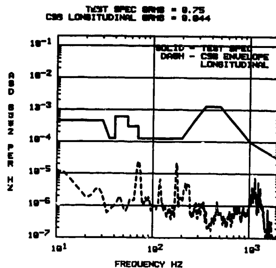
Figure 10. Comparison of Horizontal Axis Aircraft Cruise Test Specification and C98 Longitudinal Axis Random Vibration Envelope.
