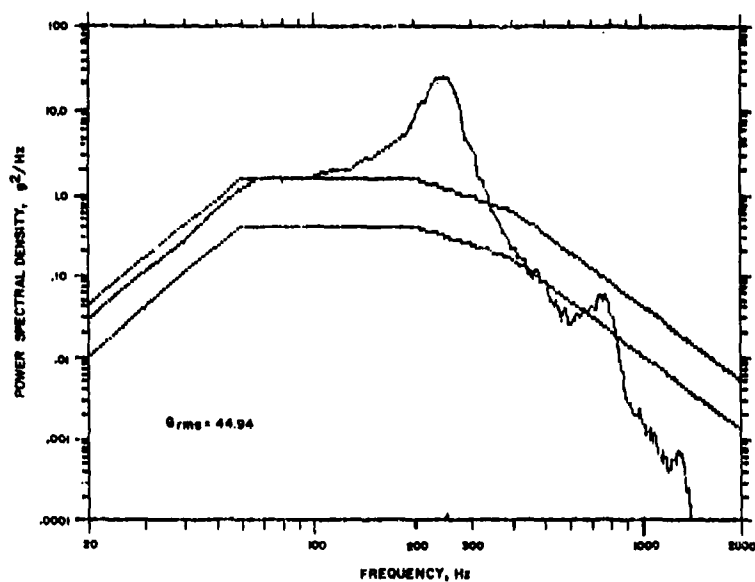
FIGURE 5: TYPICAL ISOLATOR ACCELERATION OUTPUT, RANDOM VIBRATION TEST
