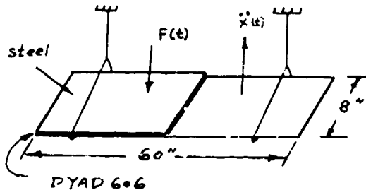
Figure 1: Test specimen
