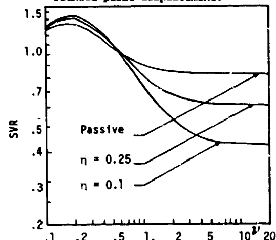
Figure 12: SVR response of sequential damper.
