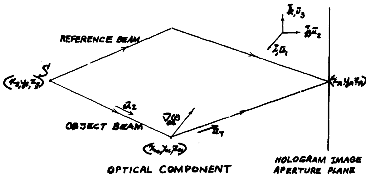
FIGURE 8 REPRESENTATIVE LINE DRAWING SHOWING VIBRATORY MOTION GEOMETRY FOR AN OPTICAL COMPONENT IN OBJECT BEAM PATH. NOTE THAT \bar{u}_i , \bar{u}_t ARE THREE-DIMENSIONAL UNIT VECTORS FOR INCIDENT, TRANSMITTED OPTICAL BEAMS AT OPTICAL COMPONENT
