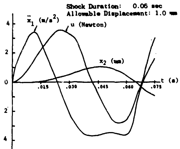
Fig. 2 Time variation of control u , acceleration \ddot{x}_1 , and displacement x_2 by use of natural frequencies
