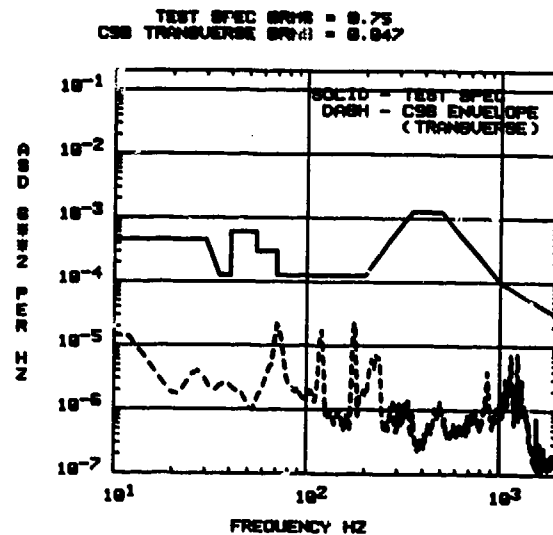
Figure 9. Comparison of Horizontal Axis Aircraft Cruise Test Specification and C98 Transverse Axis Random Vibration Envelope.
