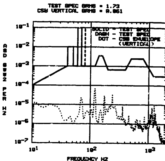
Figure 8. Comparison of Vertical Axis Aircraft Cruise Test Specification and C98 Vertical Axis Random Vibration Envelope.
