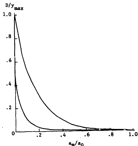
Fig. 2 Limiting performance trade-off curves
