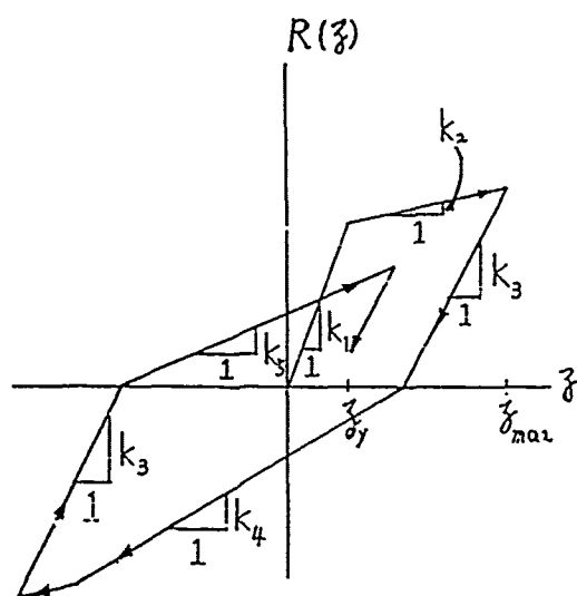
Fig. 3: The Q-hysteresis [3].
