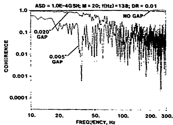
Fig. 11 - Coherence functions for the rattle gaps compared in Figures 8 through 10.
