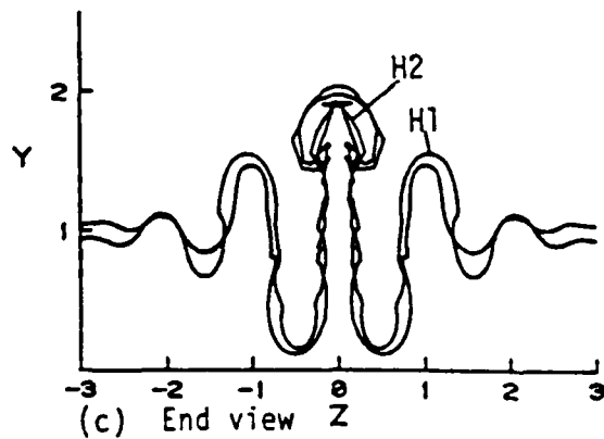
Figure 4. - Development of the two hairpin vortices at t=.048 .
