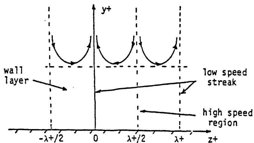
Figure 5. Schematic diagram of the assumed wall-layer structure during a typical quiescent period.
