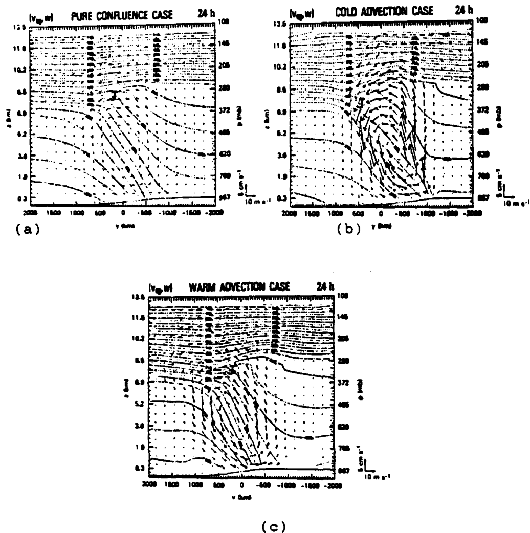
Figure 13. Cross sections of the transverse ageostrophic circulation ( v_{ag} , w ) and potential temperature in the jet entrance zone after 24 h integration of a two dimensional primitive equation model of frontogenesis; (a) for pure confluence; (b) confluence in the presence of cold air advection; (c) warm air advection with diffluence. Location of Jet axis along-front velocity indicated by J. (Keyser and Pecnic, 1985).
