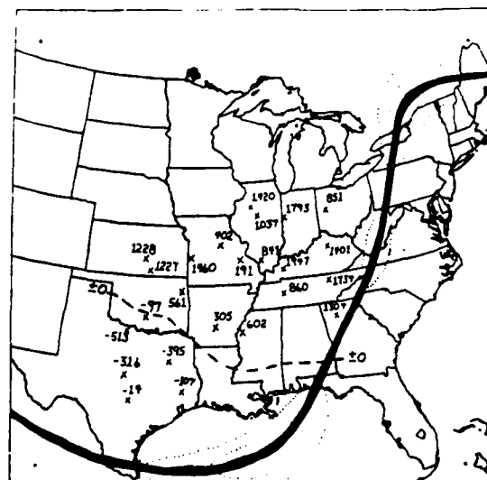
Figure 42. Computations at the midway point of all parcels in the preselected grid for the period of (a) 0000-1200 GMT 27 February 1984 and (b) 1200-0000 GMT 27-28 February 1984, for changes in potential energy. Dashed line is isopleth between positive and negative values.
