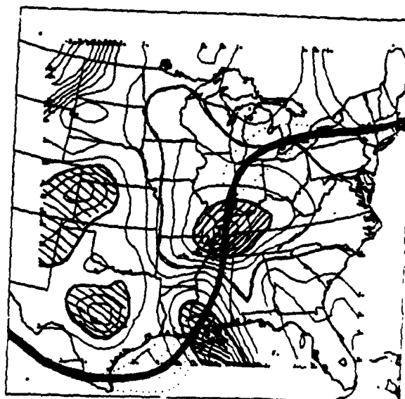
Figure 45. Calculations of omega (a) on a 292^{\circ}\text{K} isentropic surface at 0000 GMT 27 February (b) on a 288^{\circ}\text{K} isentropic surface at 1200 GMT. Right/Left stippled regions are enhanced areas of rising/sinking motions.
