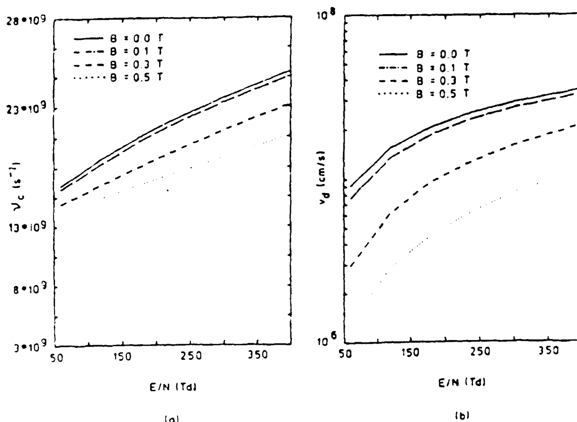
Fig. 2. Collision frequency (a) and drift velocity (b) as a function of E/N for various magnetic flux densities, p = 10 torr, 20% \text{SF}_6 - 80% \text{He} .
