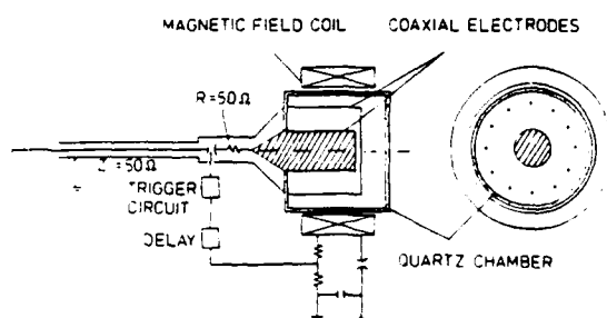
Fig. 5. Experimental apparatus.
