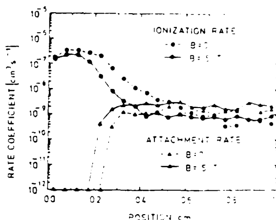
Fig. 6. Ionization and attachment rate coefficients in the cathode fall and positive column.
