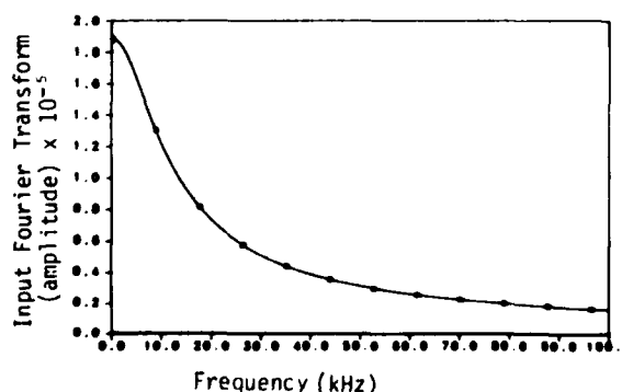
FIG. 6 - Frequency Content of Exponential Step Wave
