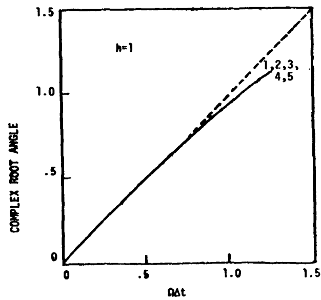
Figure 3.6b. Fully Implicit, Mode 2 Periodicity Error
