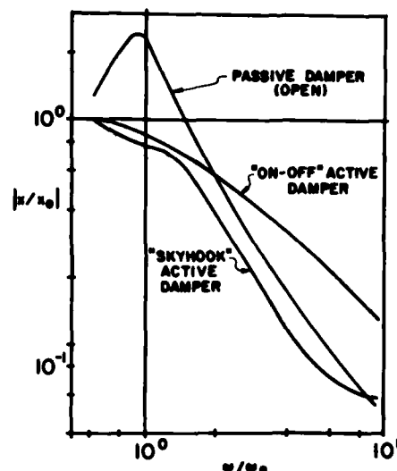
Figure 8 Comparing the Experimental Performance of Passive, "On-Off", and "Skyhook" Active Damping
