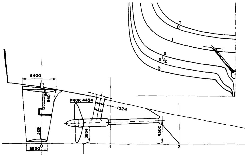
Figure 3 - Stern Configuration of Model 4148, Open Transom Design
